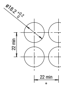
Round (LB6T)
