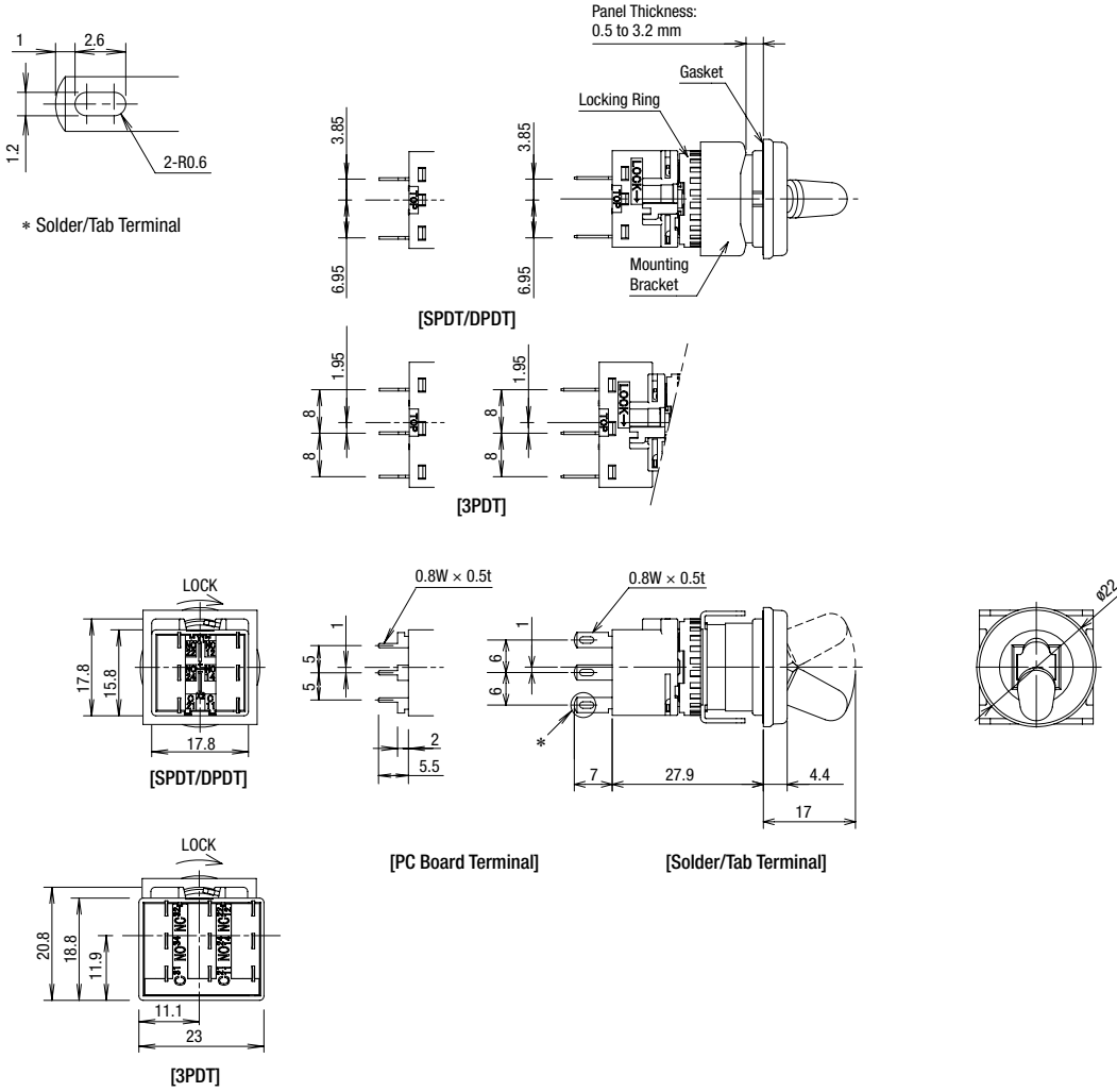
SPDT/DPDT Contacts
