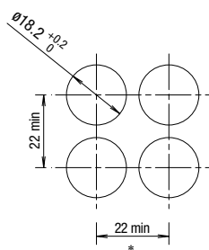
Round (LB6S/LB6MS)
