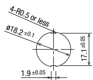
Round (LB6T)
