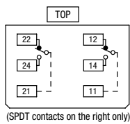
SPDT/DPDT Contacts
