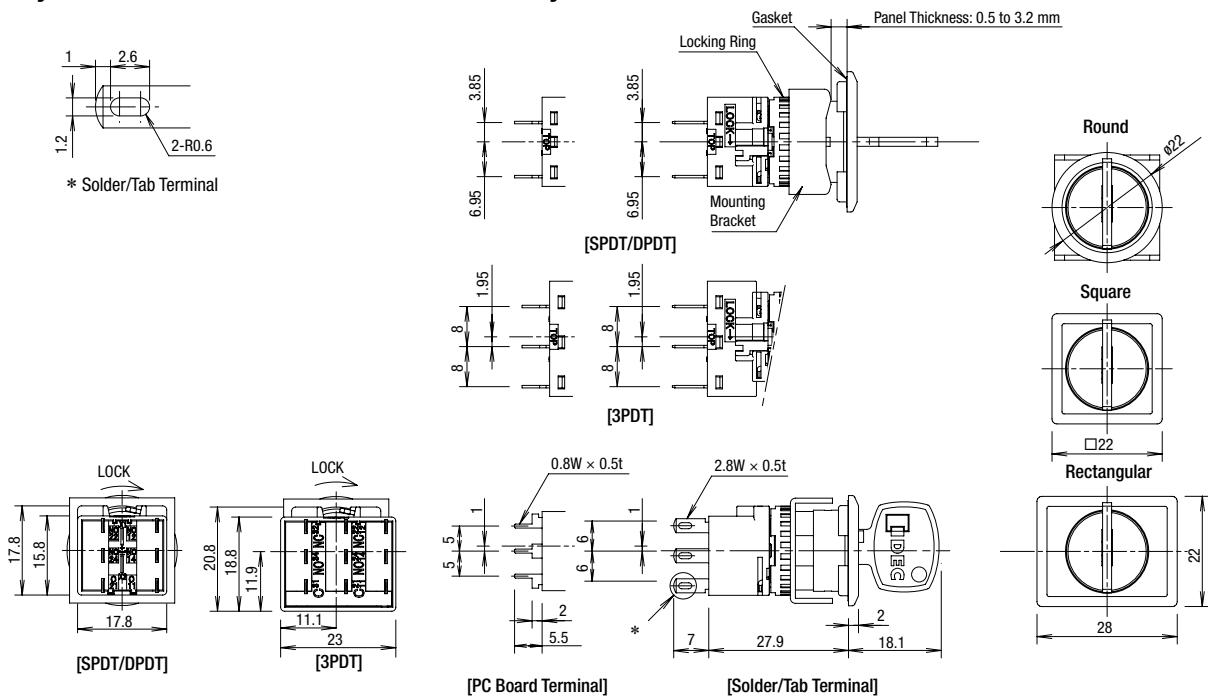
SPDT/DPDT Contacts
