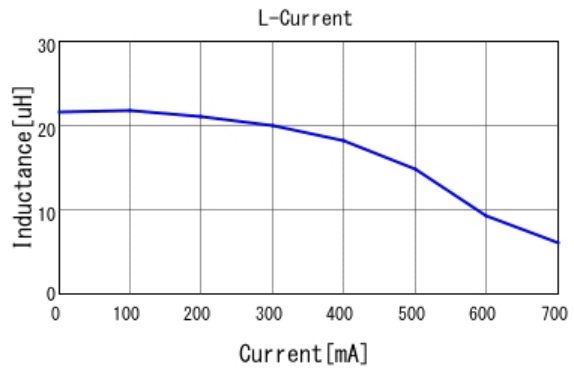
■ LQH2HPN220MGR L-Current 20degC
