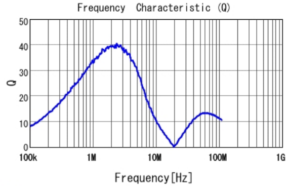
■ LQH2HPN220MGR Q
