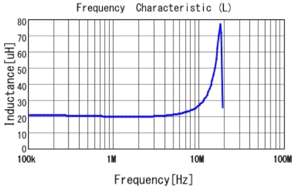
■ LQH2HPN220MGR L
