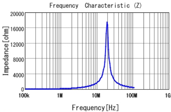
■ LQH2HPN220MGR |Z|
