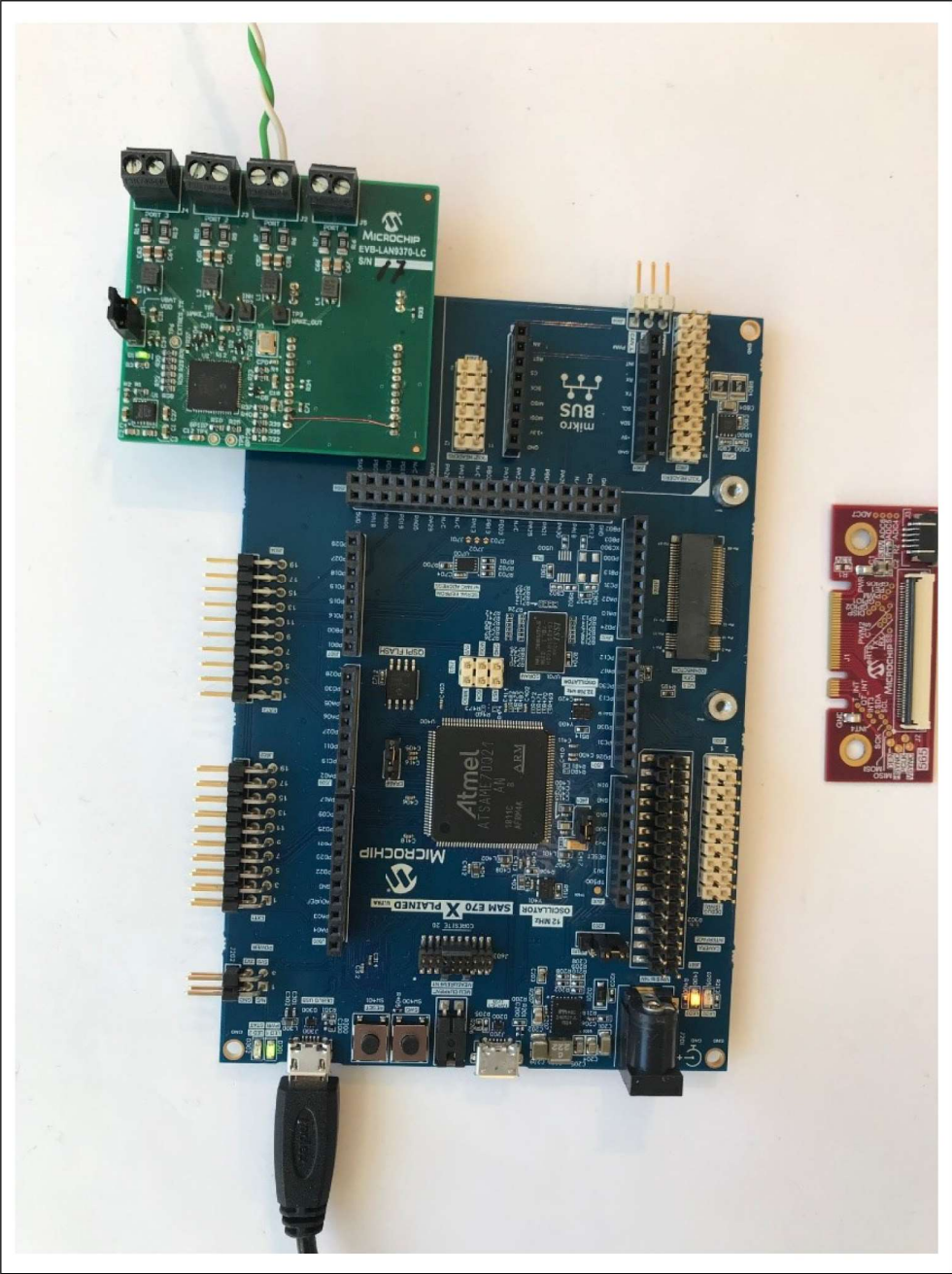
FIGURE 2-1: EVB-LAN9370 CONNECTION TO SAM E70
