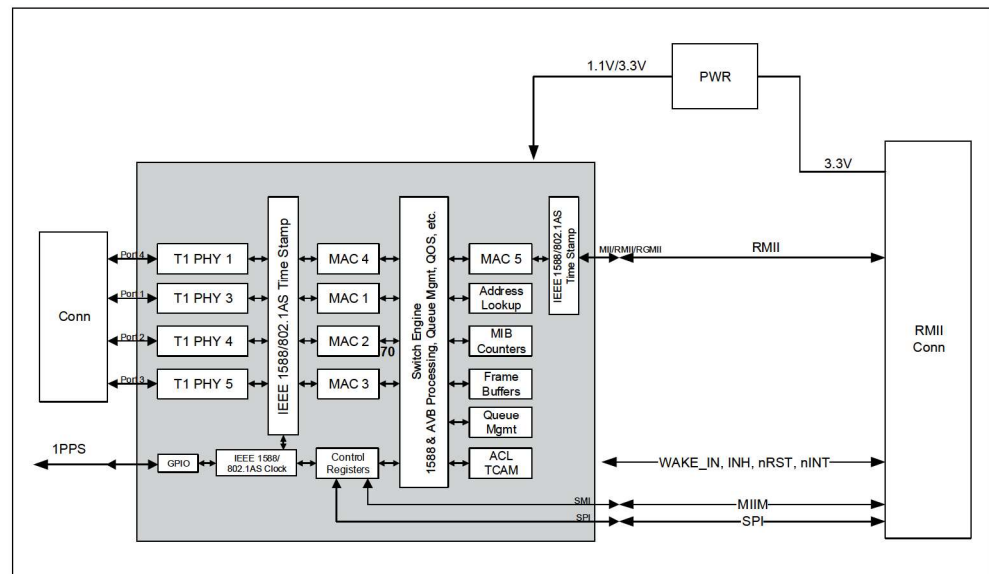
FIGURE 1-1: EVB-LAN9370 BLOCK DIAGRAM
