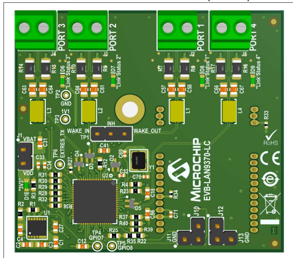
FIGURE 3-1: EVB-LAN9370 EVALUATION BOARD (TOP VIEW)
