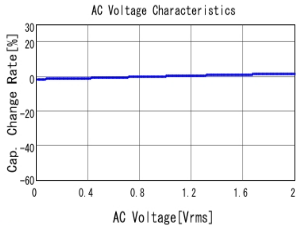
■ GCD188R71H103KA01 C-AC Voltage capchange, DC0V, 25.0d
