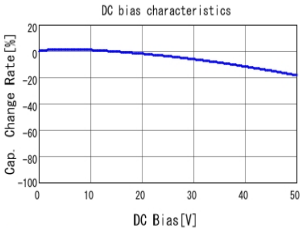
■ GCD188R71H103KA01 C-DC bias capchange, 25.0degC, AC1.
