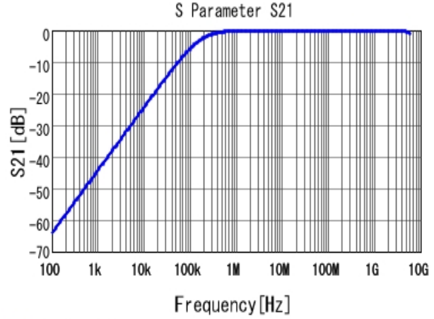
■ GCD188R71H103KA01 S21 DCOV, 25degC
