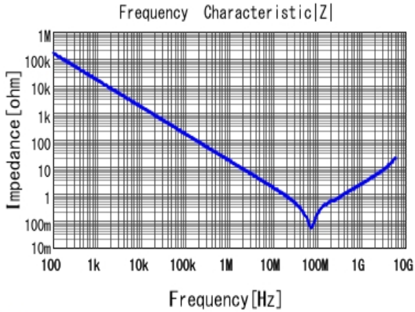
■ GCD188R71H103KA01 |Z| DC0V, 25degC
