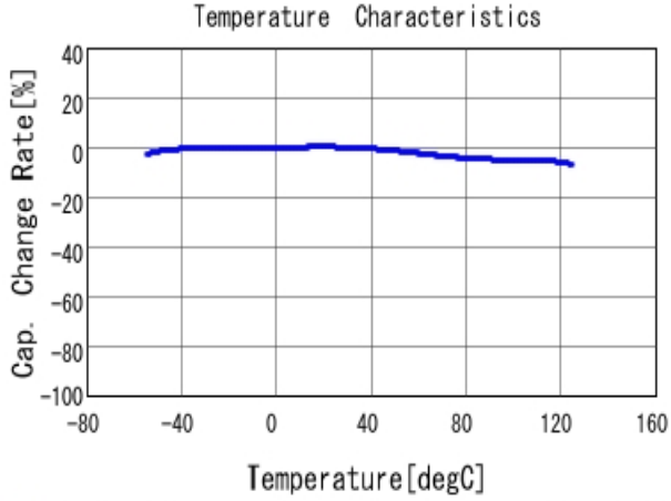
■ GCD188R71H103KA01 C-Temp. capchange, DCO. 0V, AC1.0V rm
