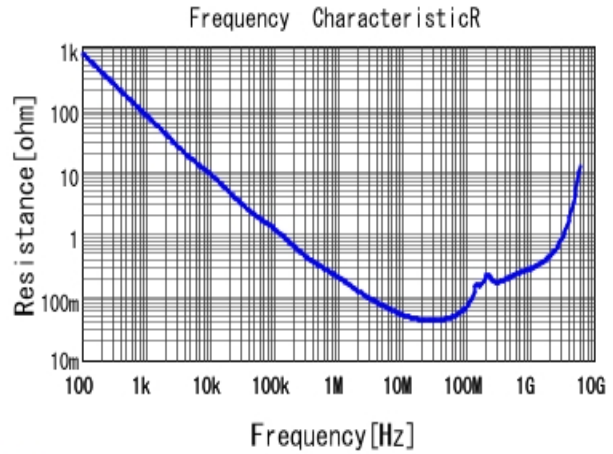
■ GCD188R71H103KA01 R DC0V, 25degC
