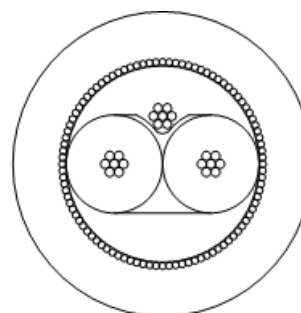
Cable Diagram
