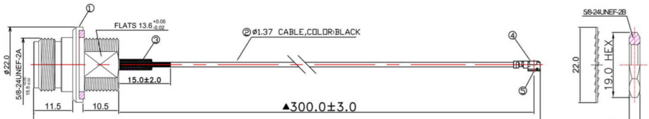
N B/H Jack \Phi 1.37 U.FL R/A Plug, Black, 50 \Omega , L=300,MM
