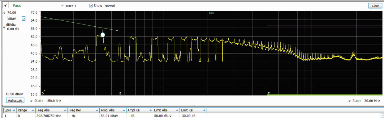
EMI; Conducted CISPR 22; Peak vs. Average Limit; L1; 208Vac 12Vdc @ 82A dc
