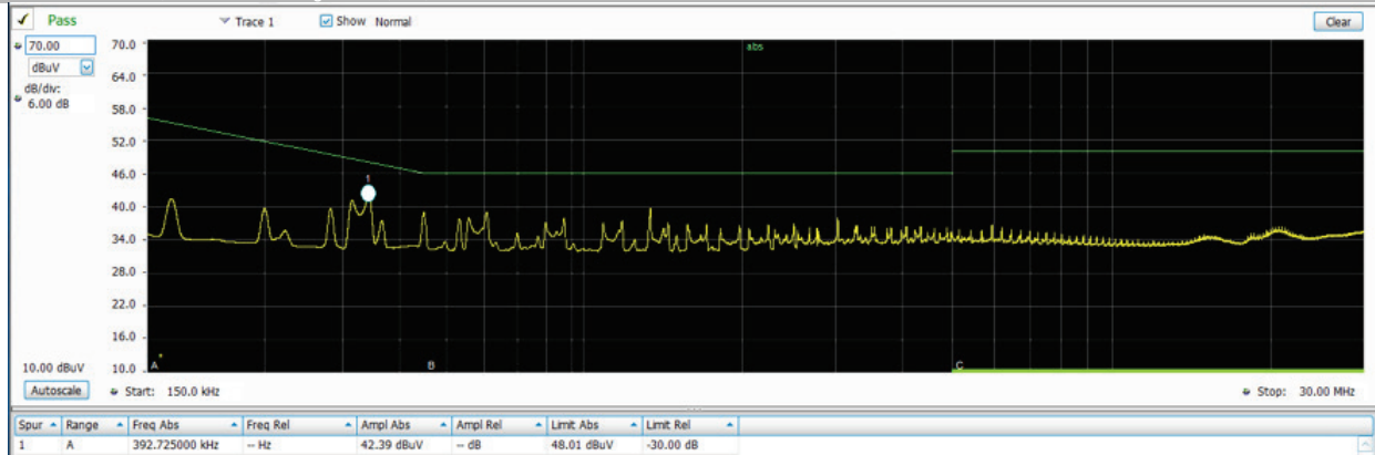
EMI; Conducted CISPR 22; QP Limit; 208Vac 12Vdc @ 82A dc
