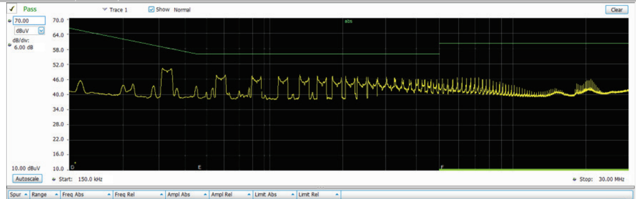
EMI; Conducted CISPR 22; QP Limit; 208Vac 12Vdc @ 82A dc
