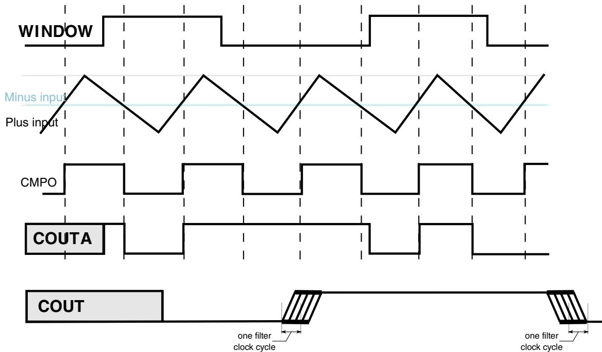
Figure 42-13. Windowed/Filtered mode operation
