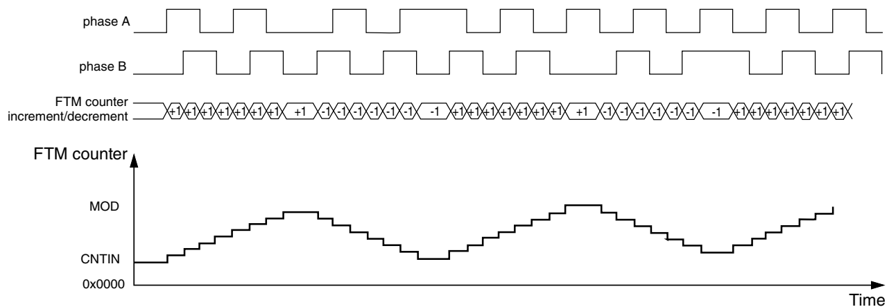
Figure 44-104. Quadrature Decoder – Phase A and Phase B Encoding Mode
