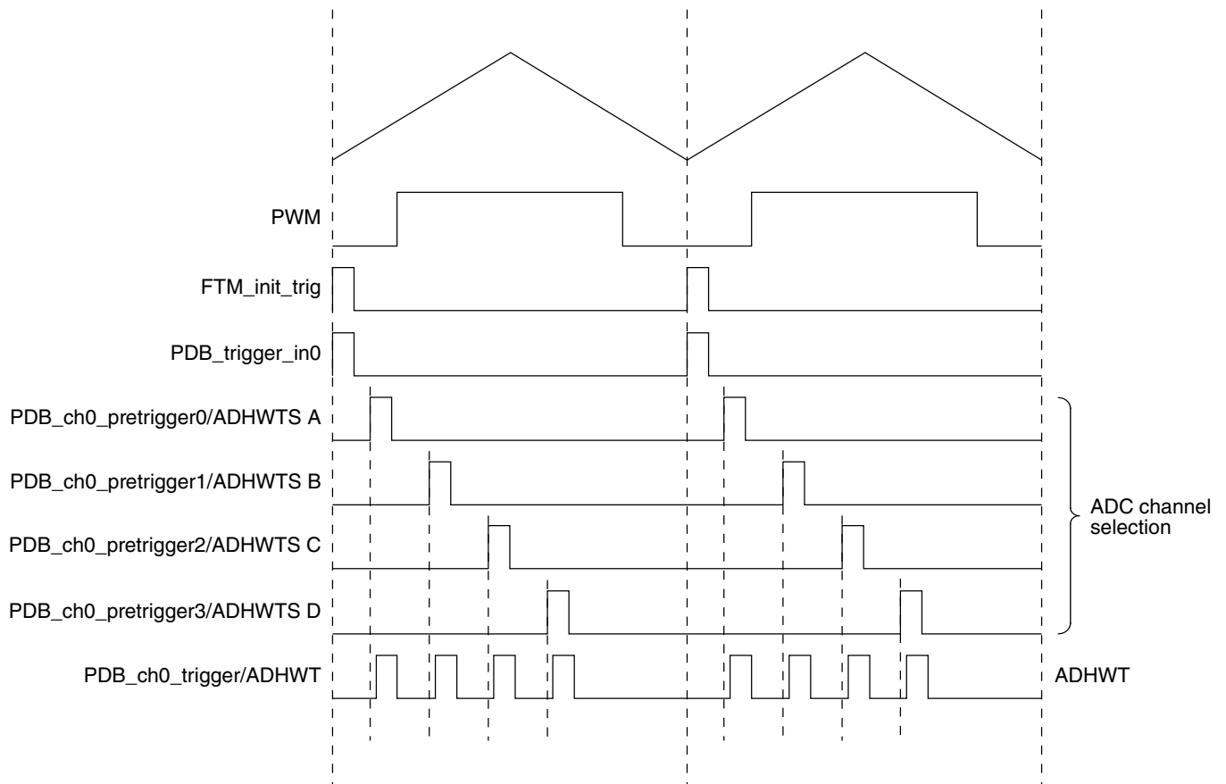
Figure 40-14. Example: PWM Load Diagnosis – ADC Trigger Concept 1 (Timing)
