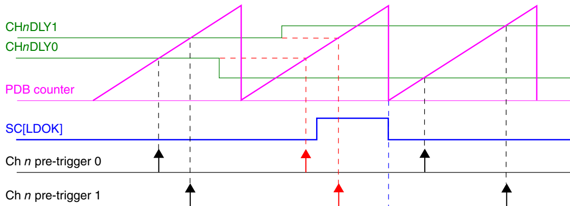
Figure 43-10. Registers update with SC[LDMOD] = x1
