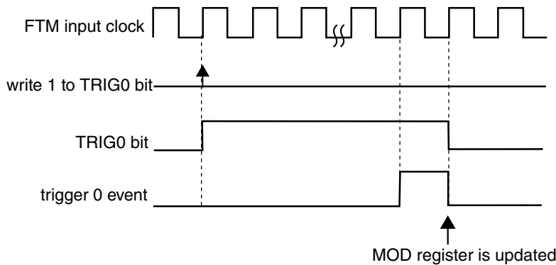
Figure 44-59. MOD synchronization with (SYNCMODE = 0), (HWTRIGMODE = 0), (PWMSYNC = 0), (REINIT = 1), and a hardware trigger was used
