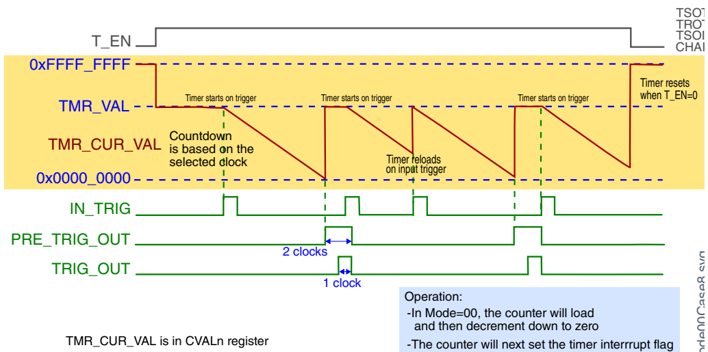
Figure 45-12. Case 8: TSOT = 1, TROT = 1, TSOI = 1, CHAIN = 0
