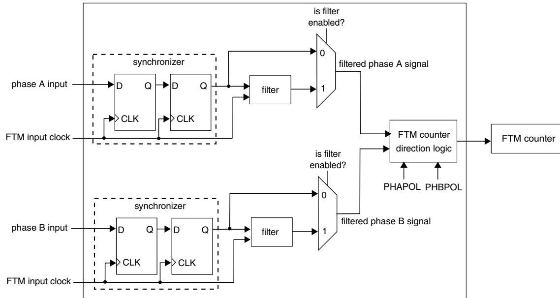
Figure 44-101. Diagram for Quadrature Decoder when FLTIPS[3:0] = 0
