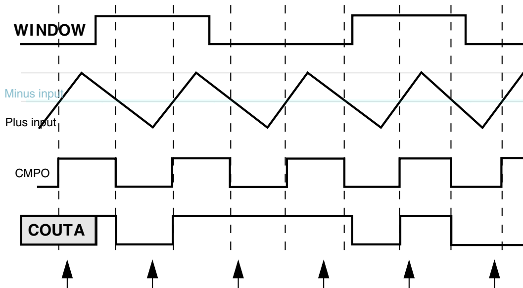
Figure 42-9. Windowed mode timing diagram
