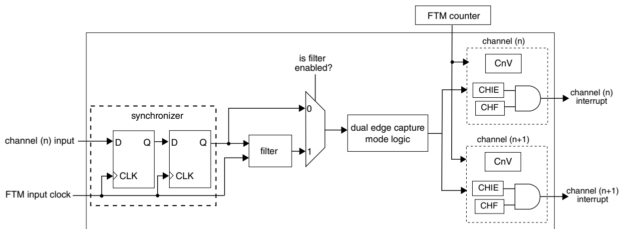
Figure 44-94. Diagram for Dual Edge Capture Mode when FLTPS[3:0] = 0
