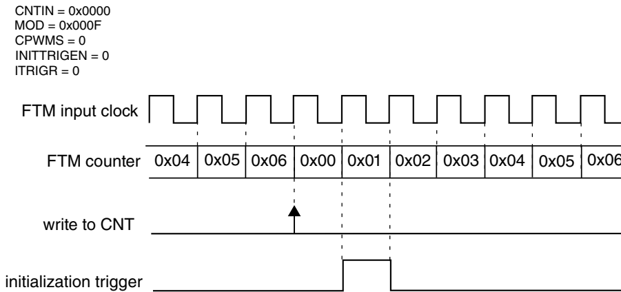
Figure 44-89. Example of the generation of the initialization trigger in the case 2.
