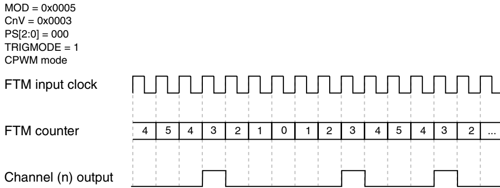
Figure 44-115. Example of channel (n) trigger at the channel (n) output in CPWM mode
