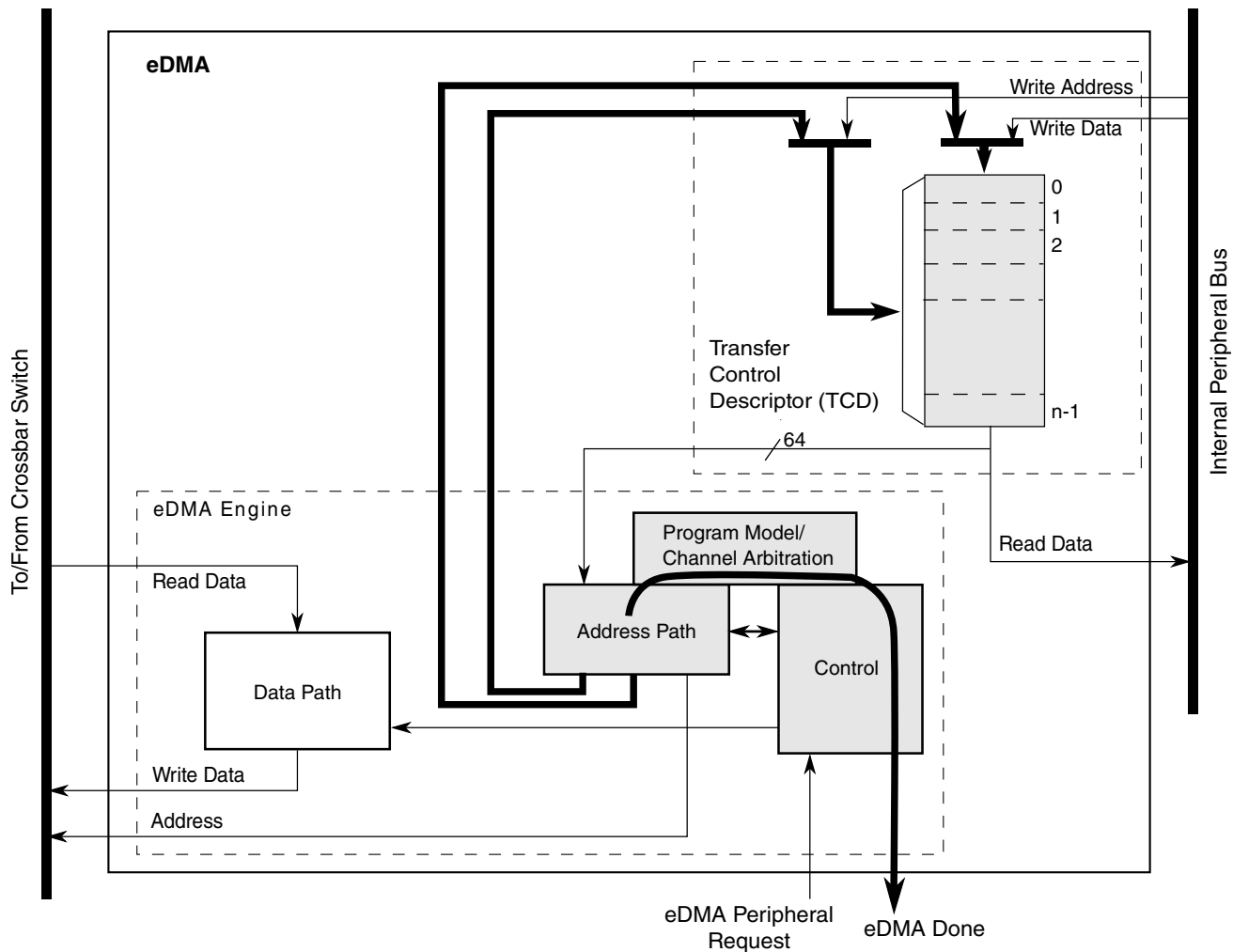
Figure 17-4. eDMA operation, part 3
