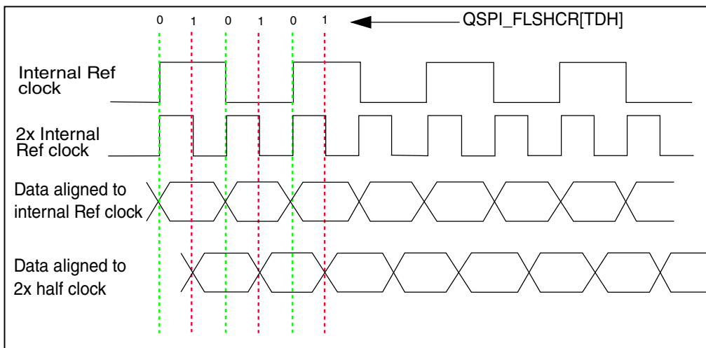
Figure 36-13. Data Hold
