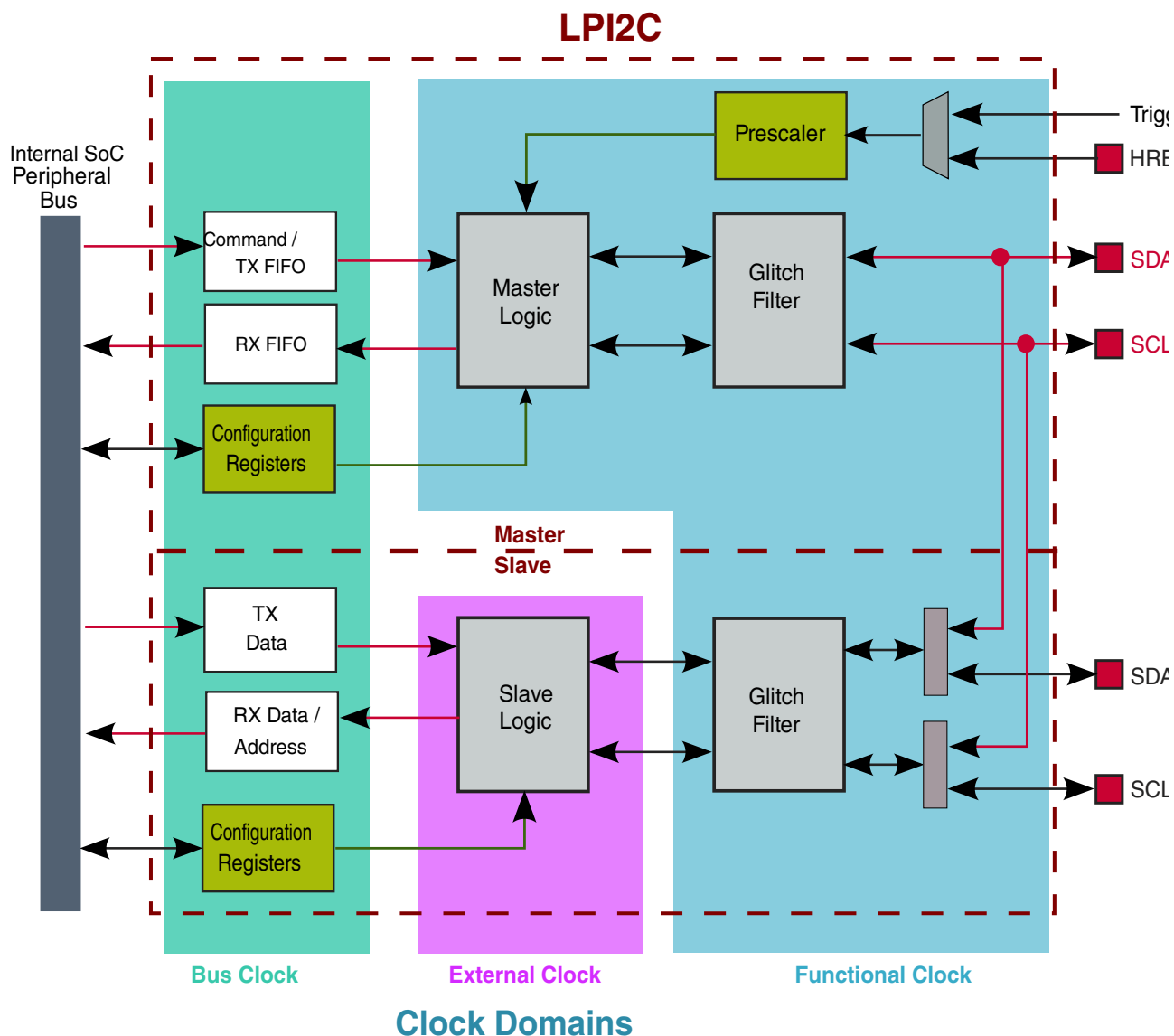
Figure 49-4. LPI2C block diagram
