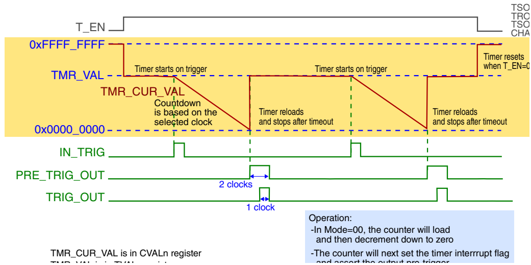
Figure 45-10. Case 6: TSOT = 1, TROT = 0, TSOI = 1, CHAIN = 0
