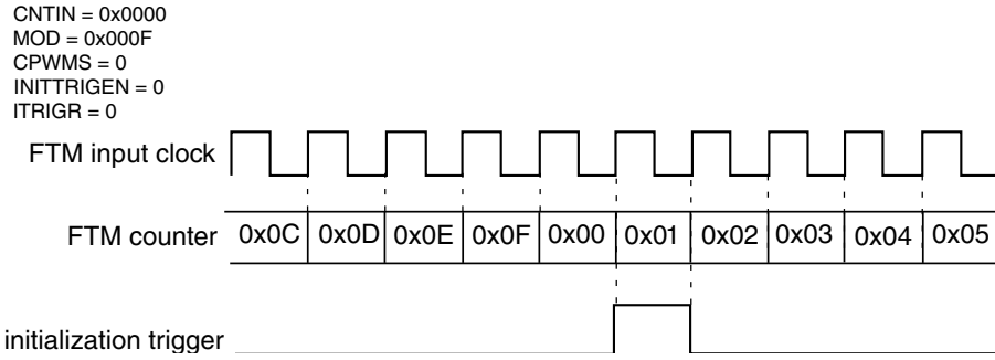
Figure 44-88. Example of the generation of the initialization trigger in the case 1.
