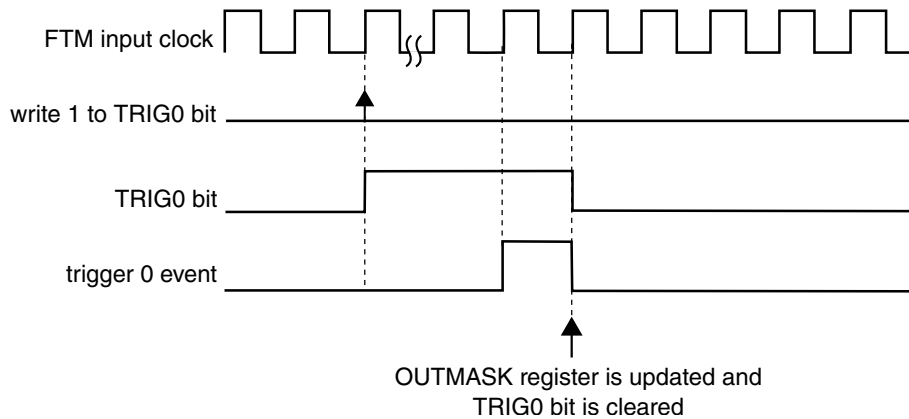
Figure 44-63. OUTMASK synchronization with (SYNCMODE = 0), (HWTRIGMODE = 0), (SYNCHOM = 1), (PWMSYNC = 0), and a hardware trigger was used
