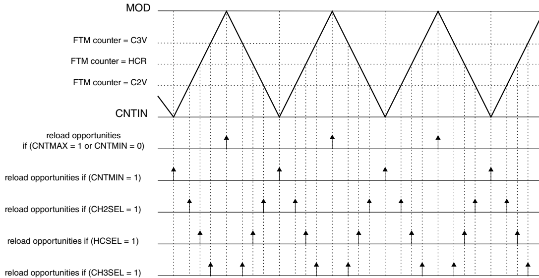
Figure 44-110. Reload opportunities when the FTM counter is an up-down counter
