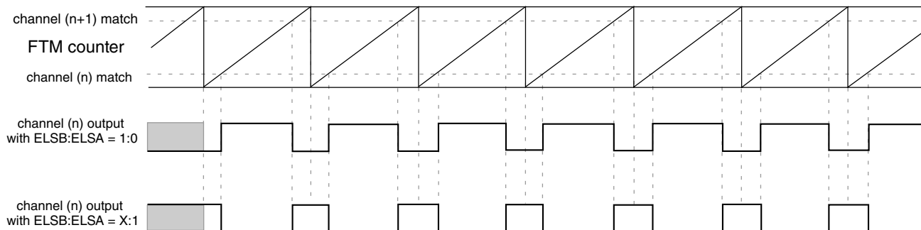
Figure 44-30. Combine mode
