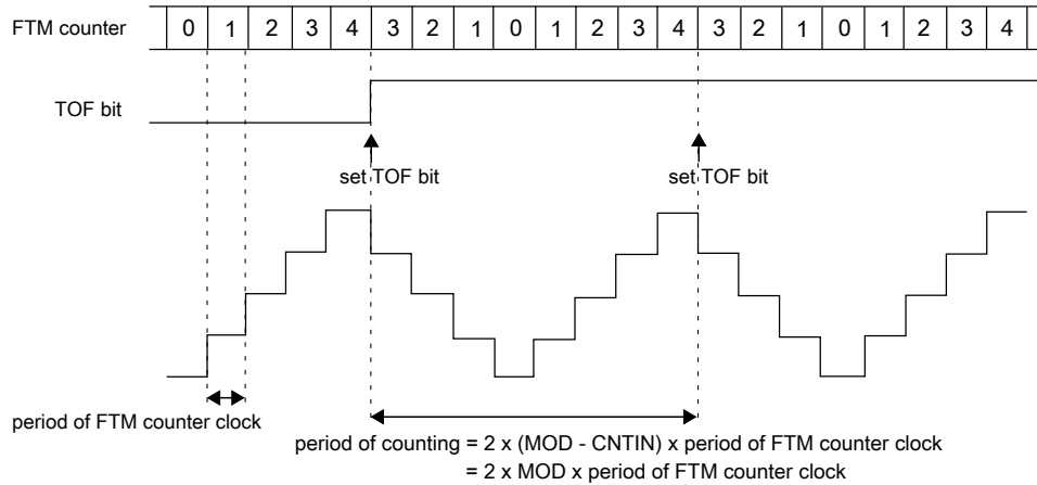
Figure 44-11. Example of up-down counting when CNTIN = 0x0000
