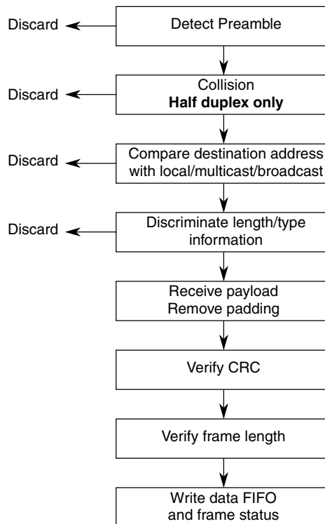
Figure 54-5. MAC receive flow
