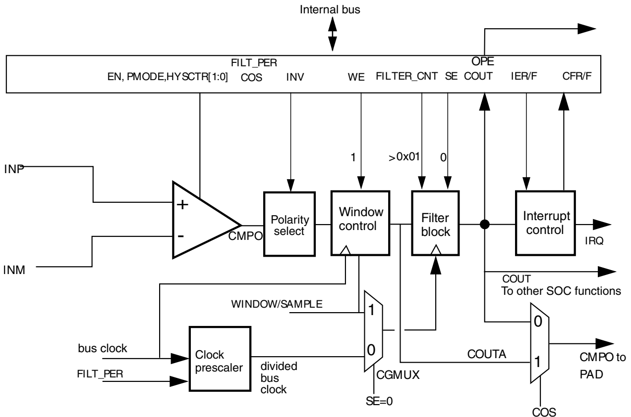
Figure 42-12. Windowed/Filtered mode
