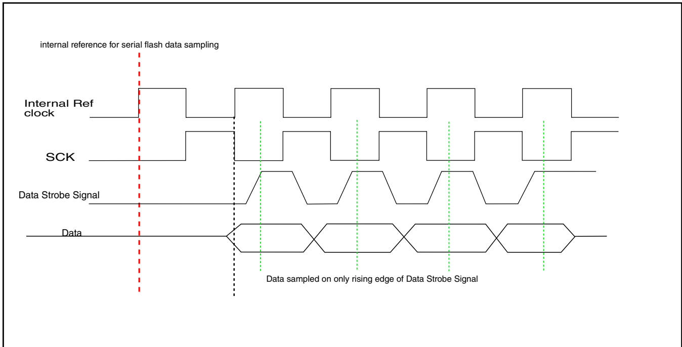
Figure 36-10. Data Strobe functionality in SDR mode
