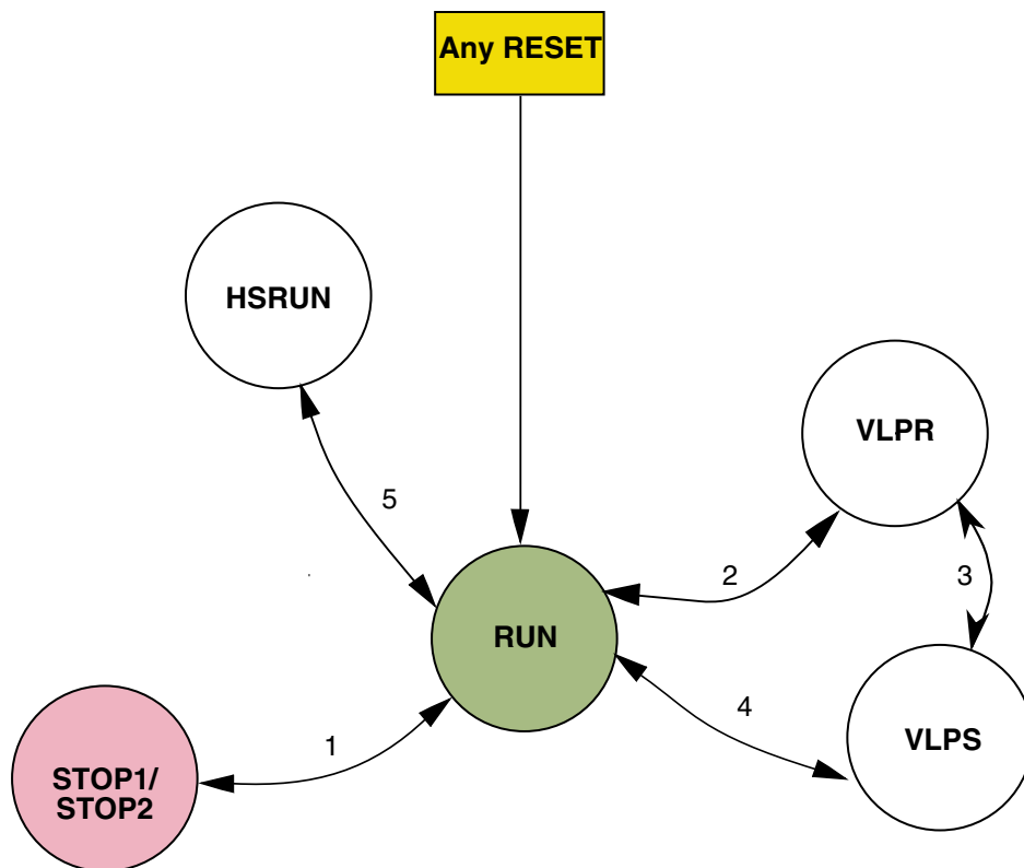
Figure 38-1. Power mode state diagram
