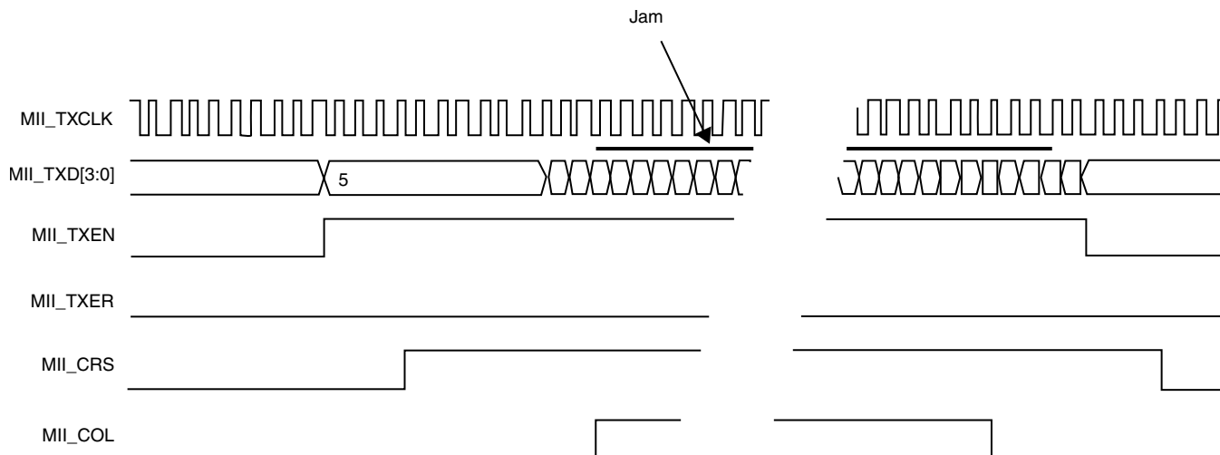
Figure 54-24. MII transmit operation — transmission with collision
