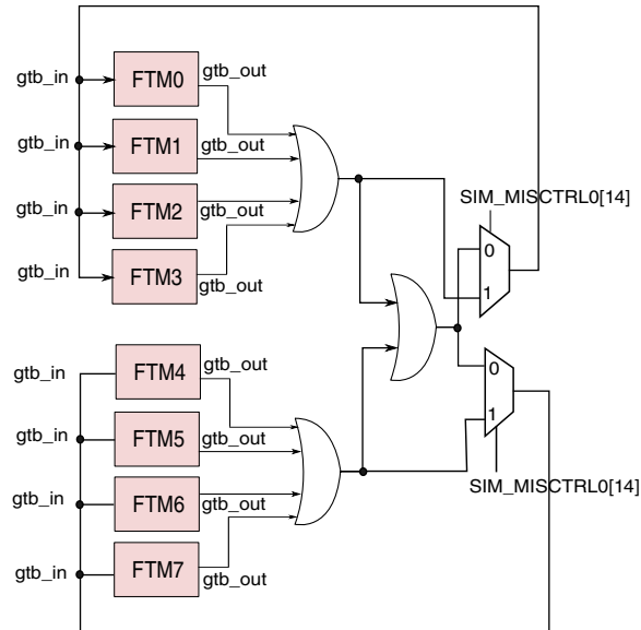
Figure 44-5. FTM global time base system interconnection
