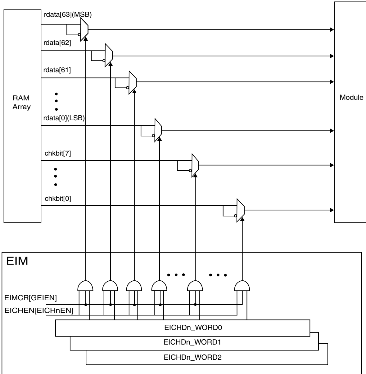
Figure 20-1. EIM functional block diagram (64-bit read data bus and 8-bit checkbit bus)
