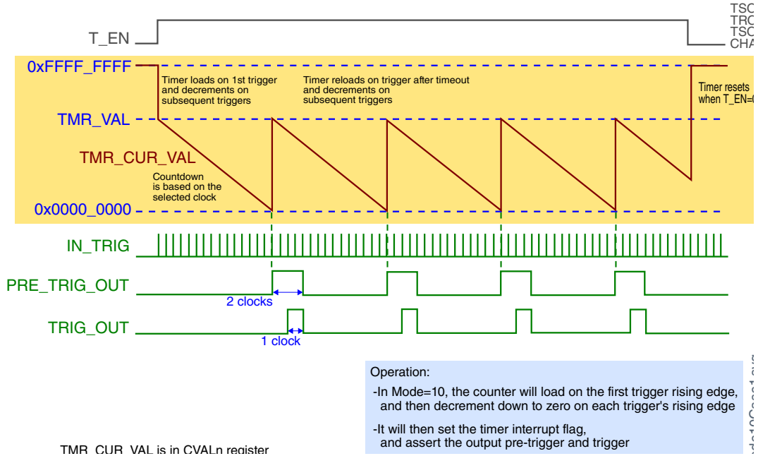
Figure 45-14. Case 1: TSOT = X, TROT = X, TSOI = 0, CHAIN = 0
