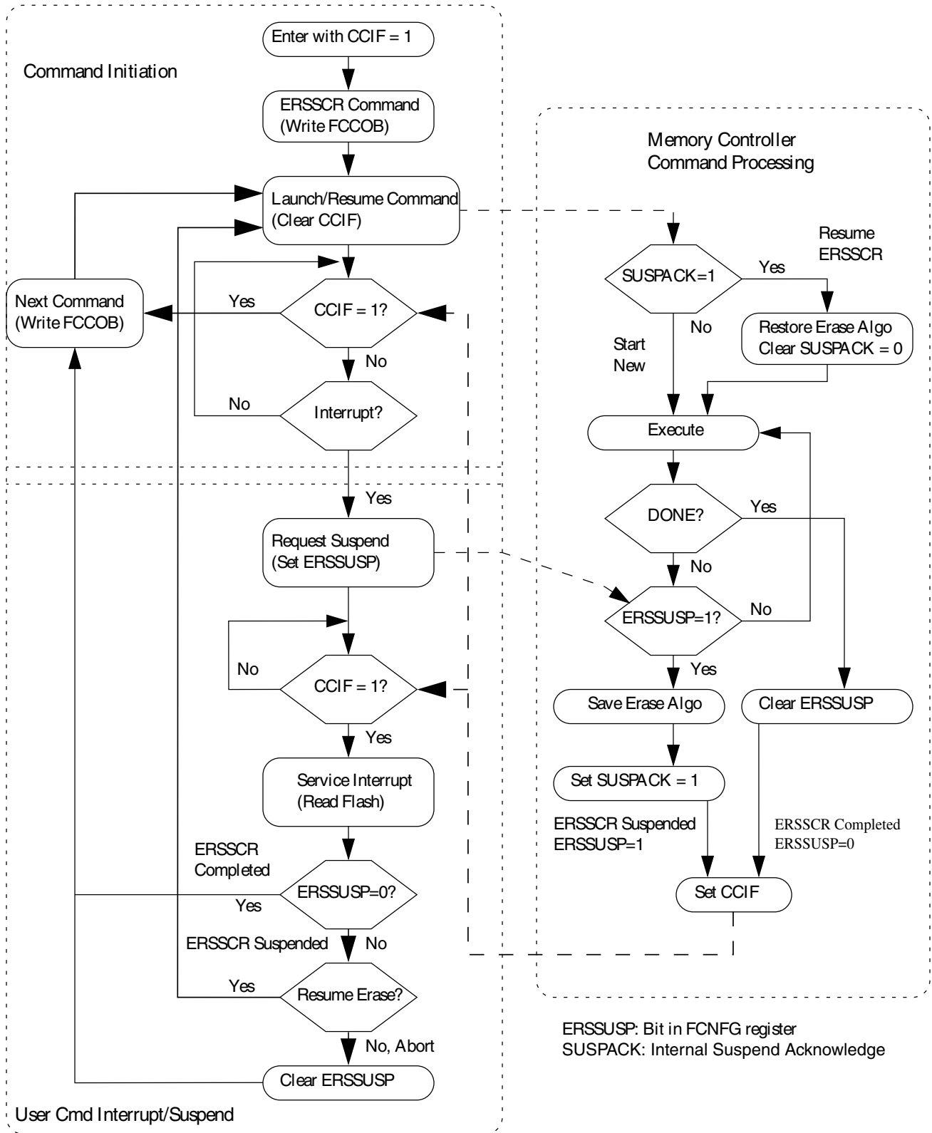
Figure 35-15. Suspend and resume of Erase Flash Sector operation
