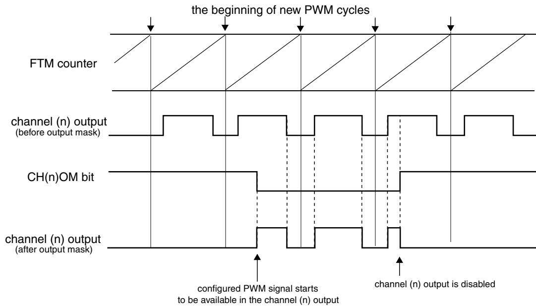
Figure 44-80. Output mask with POLn = 0
