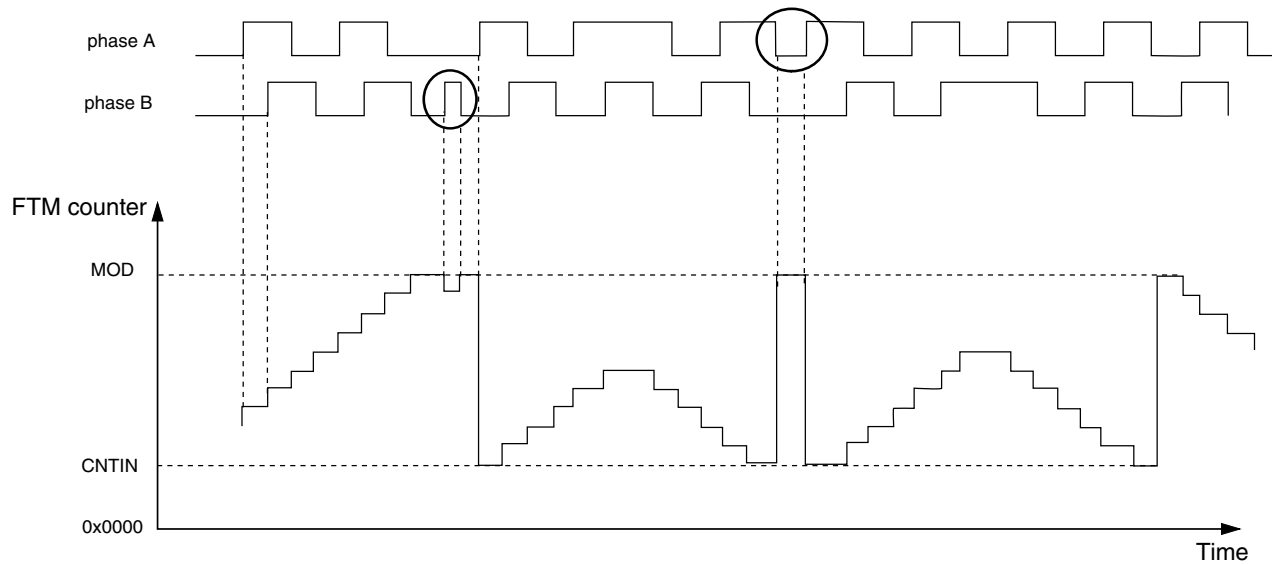
Figure 44-108. Motor position jittering near maximum and minimum count value
