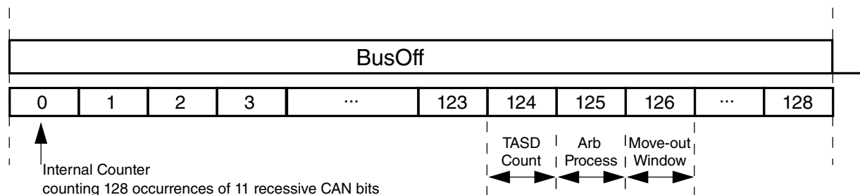
Figure 52-11. Arbitration at the end of bus off and move-out time windows
