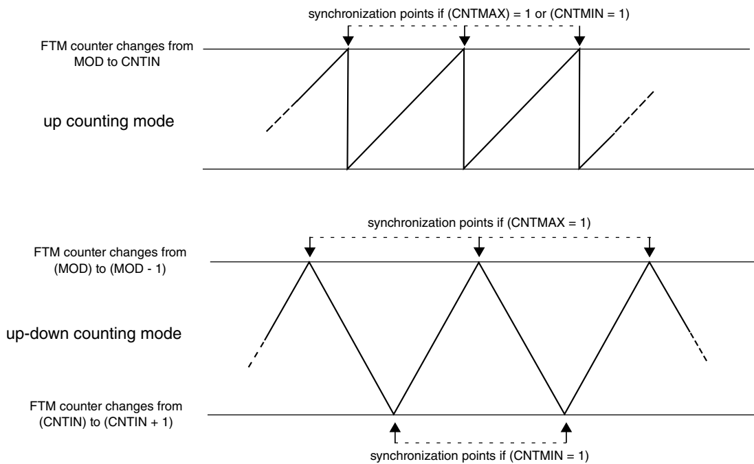
Figure 44-54. Synchronization Points
