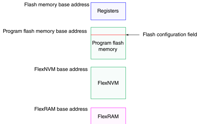
Figure 35-8. Flash memory map
