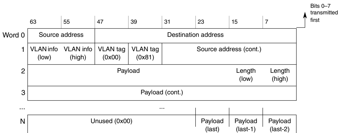
Figure 54-15. VLAN-tagged frame 64-bit mapping example
