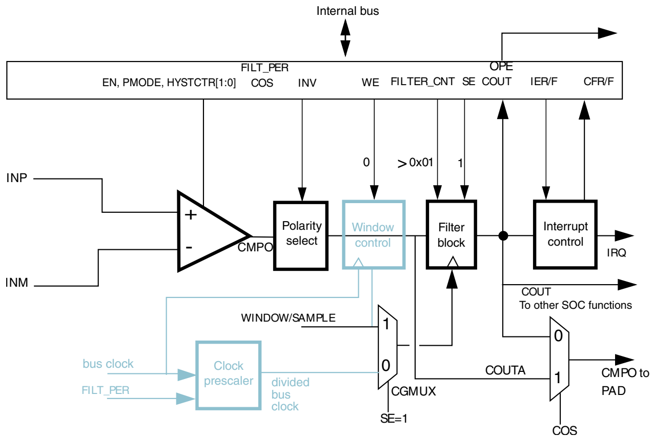
Figure 42-7. Sampled, Filtered (# 4A): sampling point externally driven
