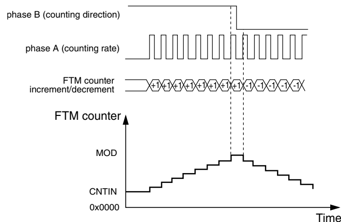
Figure 44-103. Quadrature Decoder – Count and Direction Encoding mode
