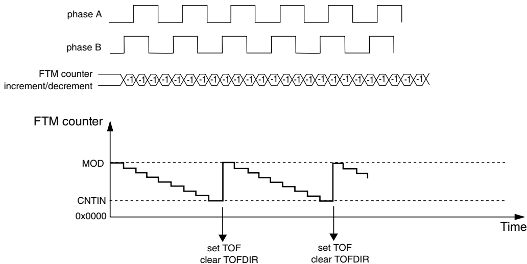
Figure 44-106. FTM Counter Overflow in Down Counting for Quadrature Decoder Mode
