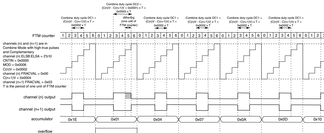
Figure 44-124. Channel (n+1) Match Edge Dithering in Combine Mode
