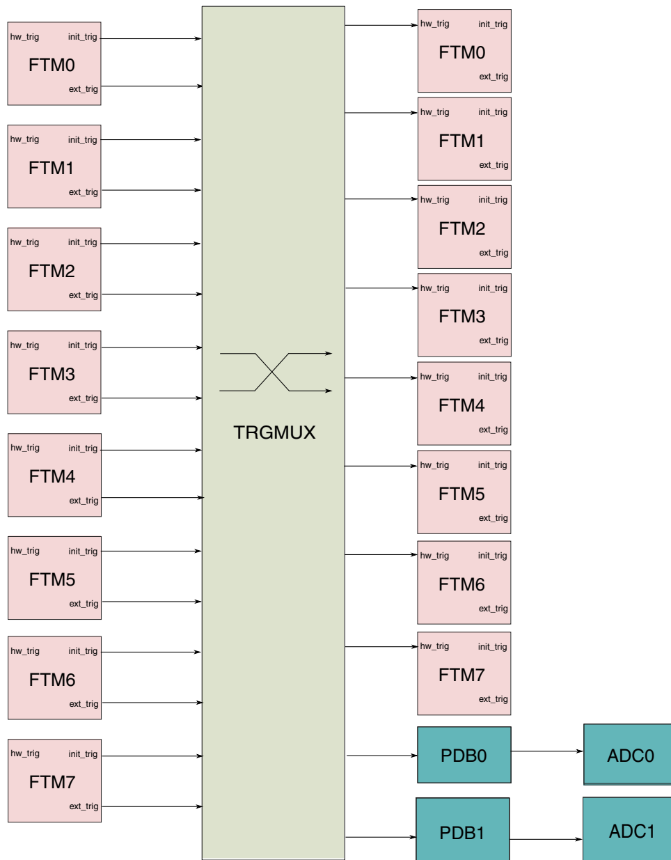
Figure 44-2. Hardware triggers
