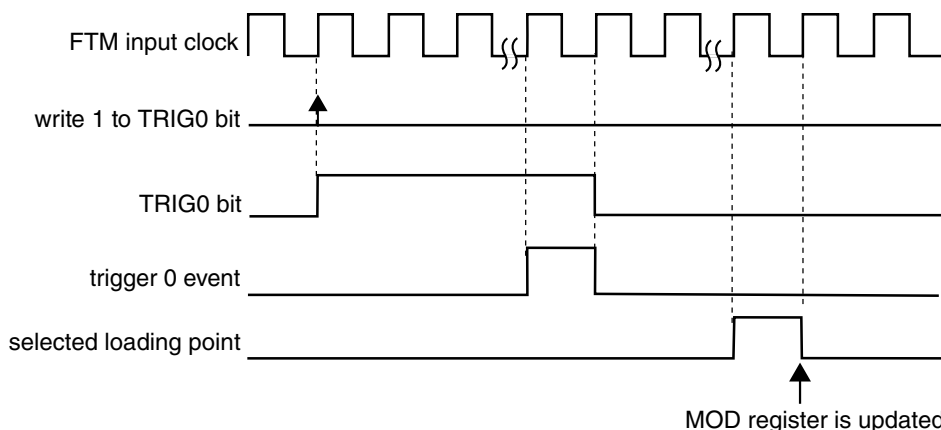
Figure 44-57. MOD synchronization with (SYNCMODE = 0), (HWTRIGMODE = 0), (PWMSYNC = 0), (REINIT = 0), and a hardware trigger was used
