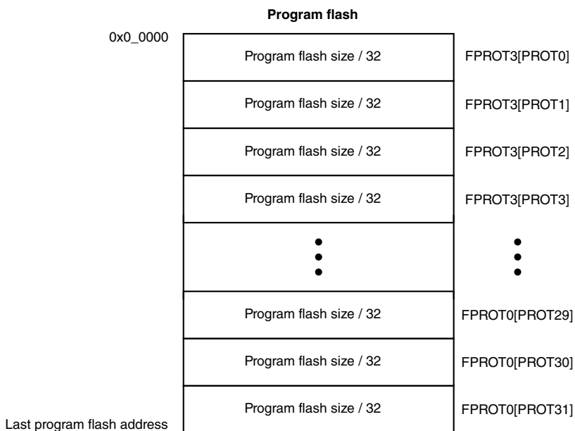
Figure 35-10. Program flash protection
