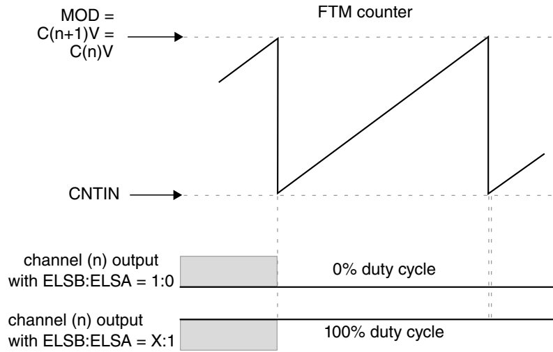
Figure 44-39. Channel (n) output if (C(n)V = C(n+1)V = MOD)
