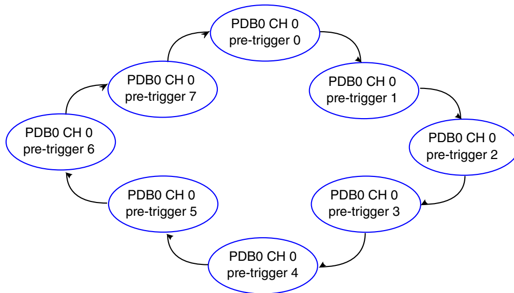
Figure 43-1. Example: PDB0 CH0 back-to-back chain
