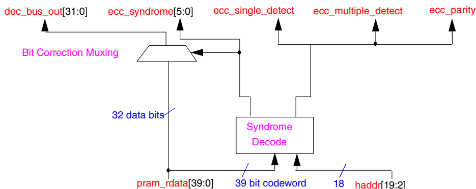
Figure 31-2. Block Diagram: 39-bit ECC Decode
