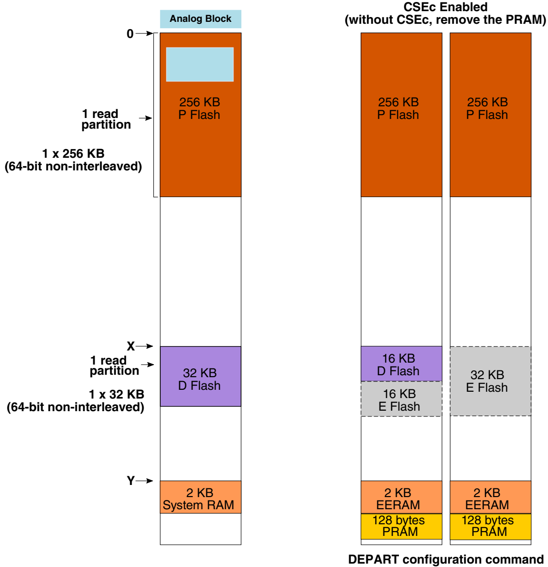
Figure 35-3. 256 KB flash memory map
