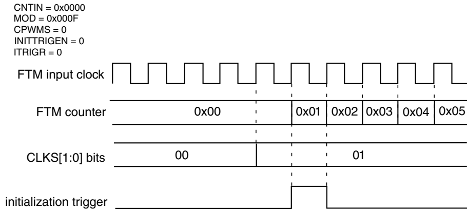
Figure 44-91. Example of the generation of the initialization trigger in the case 4.
