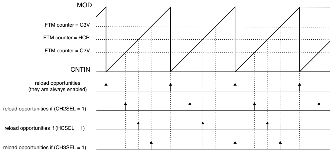
Figure 44-109. Reload opportunities when the FTM counter is an up counter
