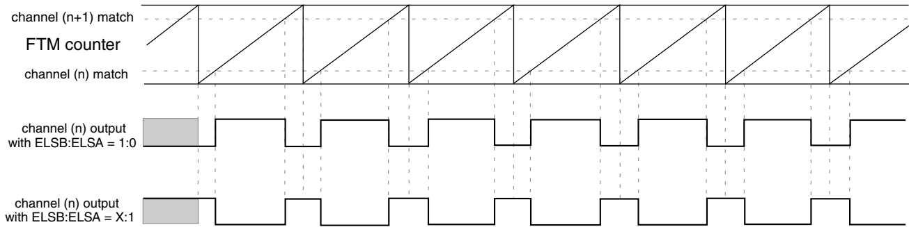
Figure 44-47. Modified Combine PWM Mode
