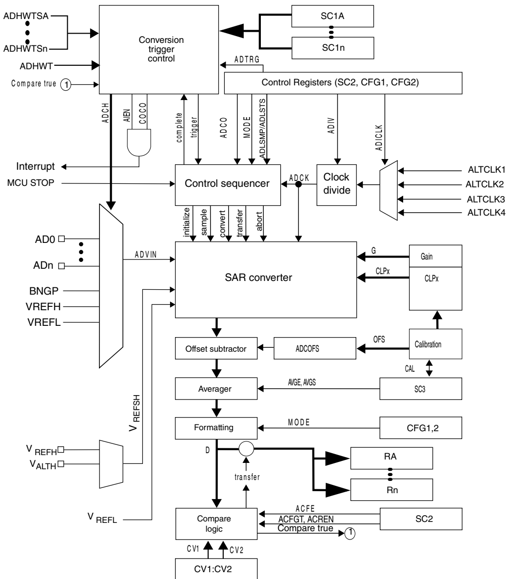
Figure 41-1. ADC block diagram
