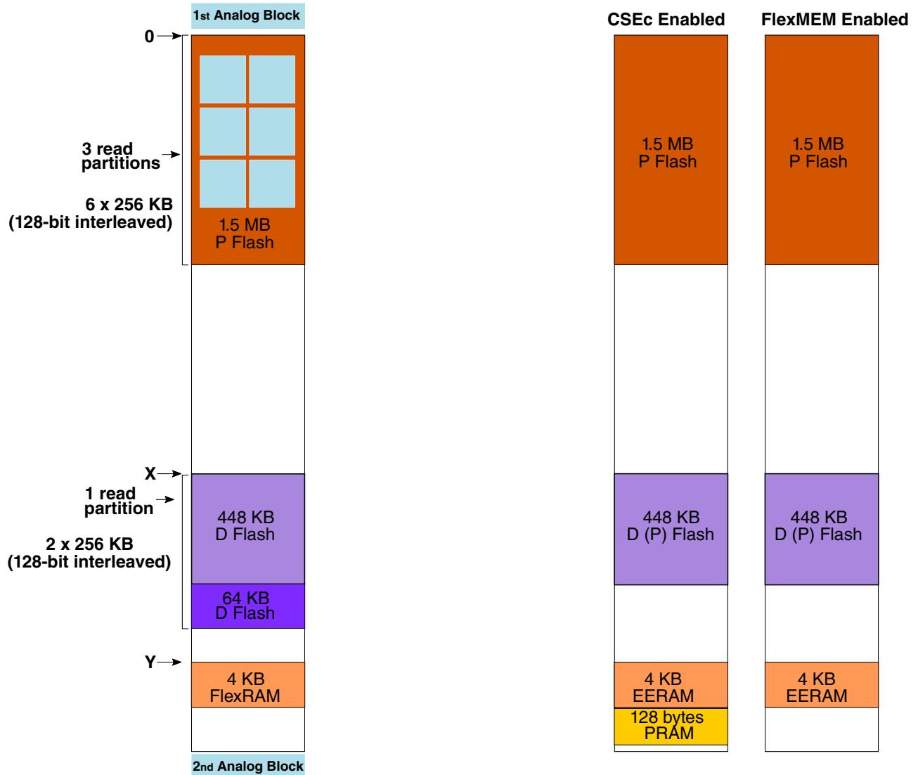
Figure 35-7. 2 MB flash memory map
