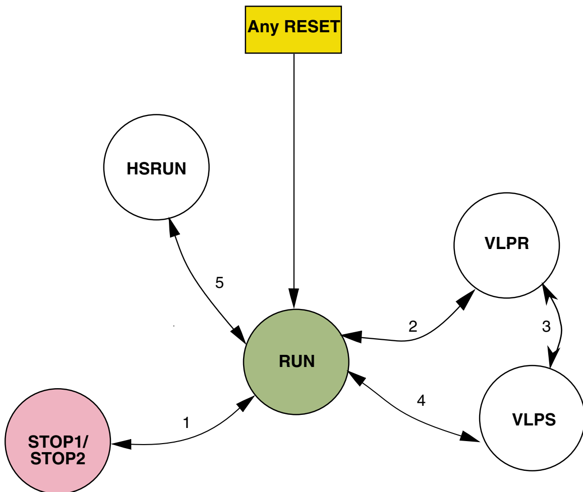
Figure 37-1. Power mode state transition diagram
