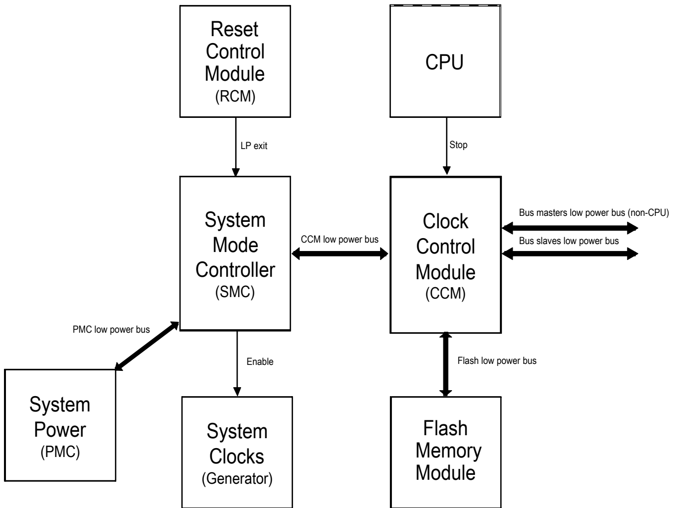
Figure 38-2. Low-power system components and connections
