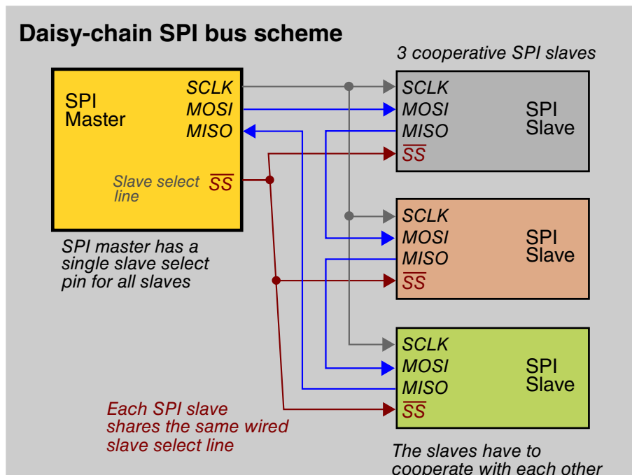
Figure 48-6. Shared slave select lines (daisy-chain) scheme
