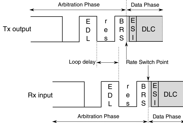
Figure 52-4. Transceiver loop delay measurement
