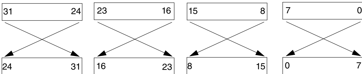
Figure 23-2. Transpose type 01
