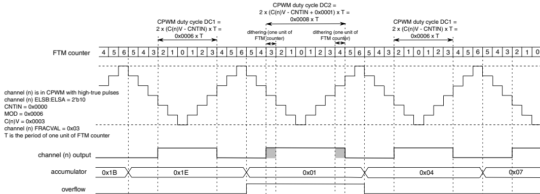
Figure 44-122. Channel (n) is in CPWM Mode with PWM Edge Dithering
