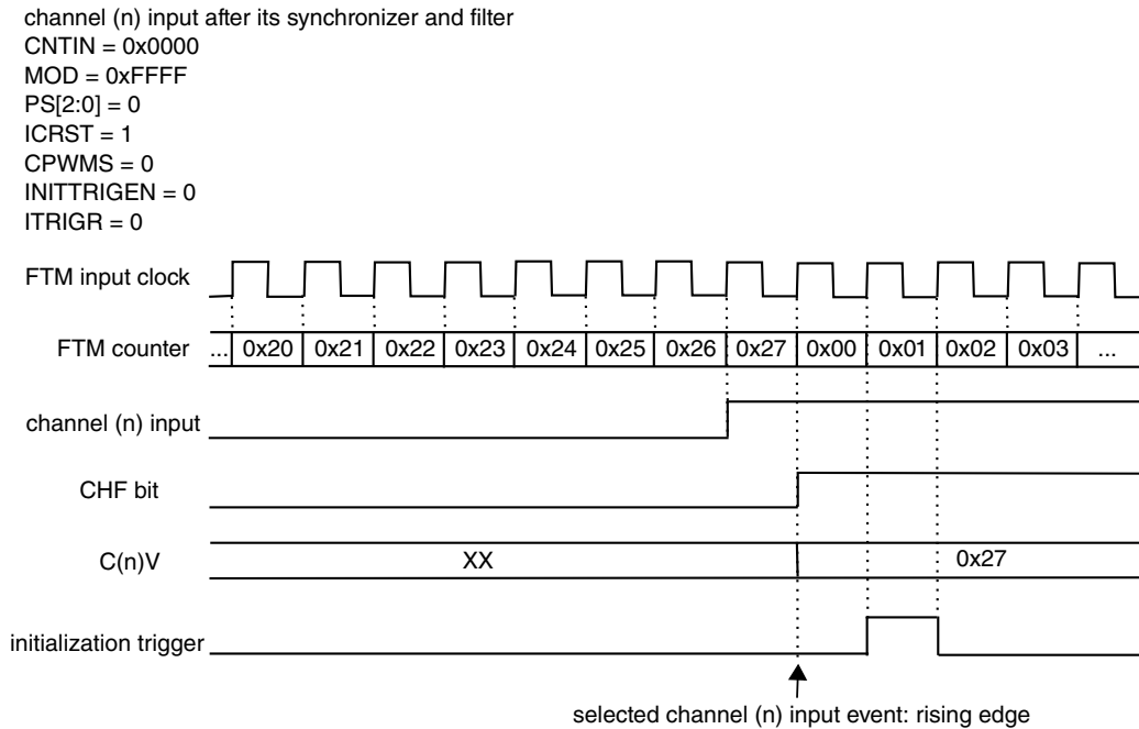
Figure 44-92. Example of the generation of the initialization trigger in the case 5.
