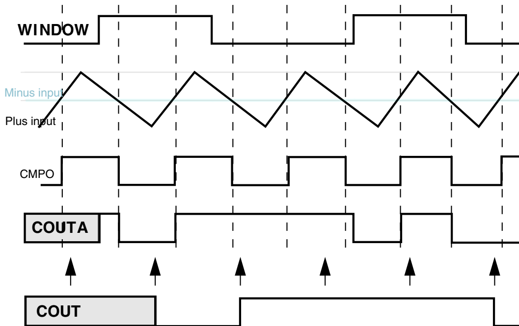
Figure 42-11. Windowed/resampled mode operation
