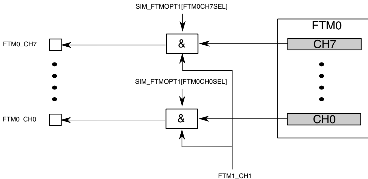
Figure 44-4. FTM Output Modulation
