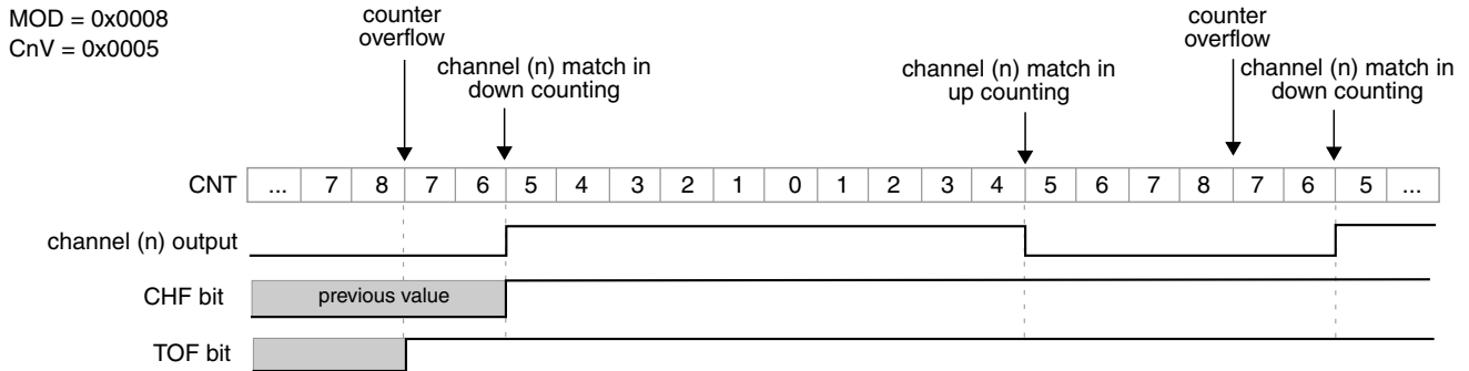
Figure 44-28. CPWM signal with ELSB:ELSA = 1:0
