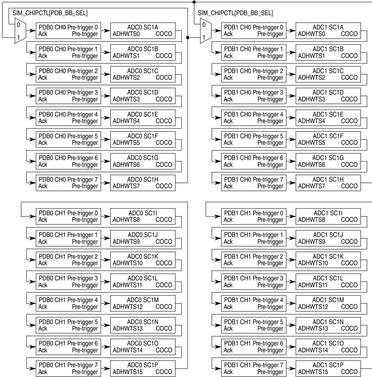
Figure 43-4. PDB-ADC back to back connection (Part 1 of 2)
