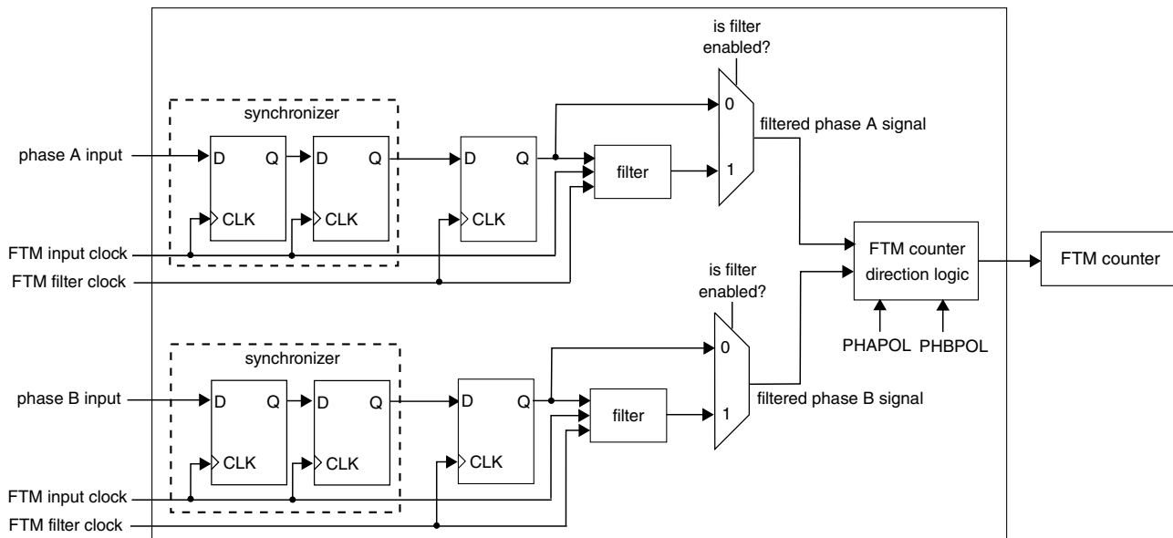
Figure 44-102. Diagram for Quadrature Decoder when FLTIPS[3:0] \neq 0
