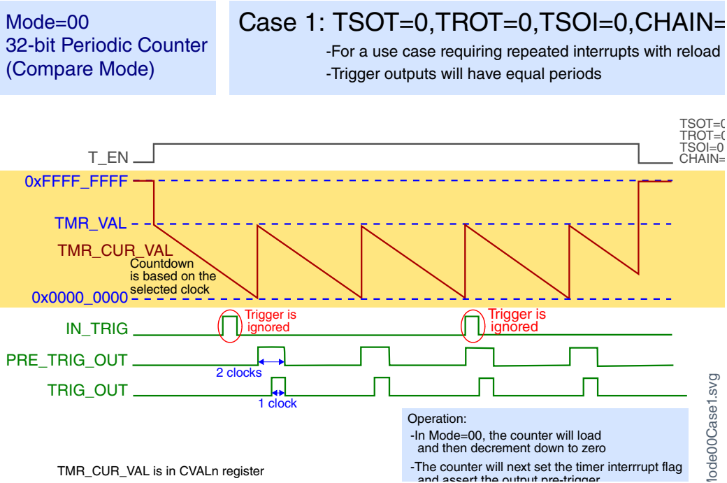
Figure 45-5. Case 1: TSOT = 0, TROT = 0, TSOI = 0, CHAIN = 0
