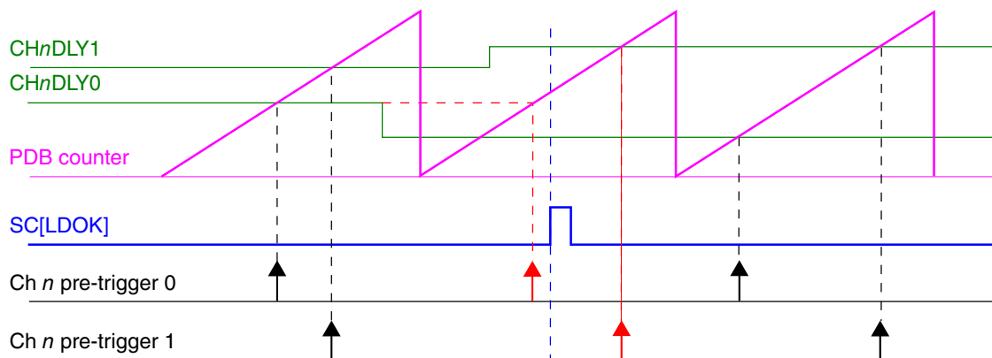
Figure 43-9. Registers update with SC[LDMOD] = 00
