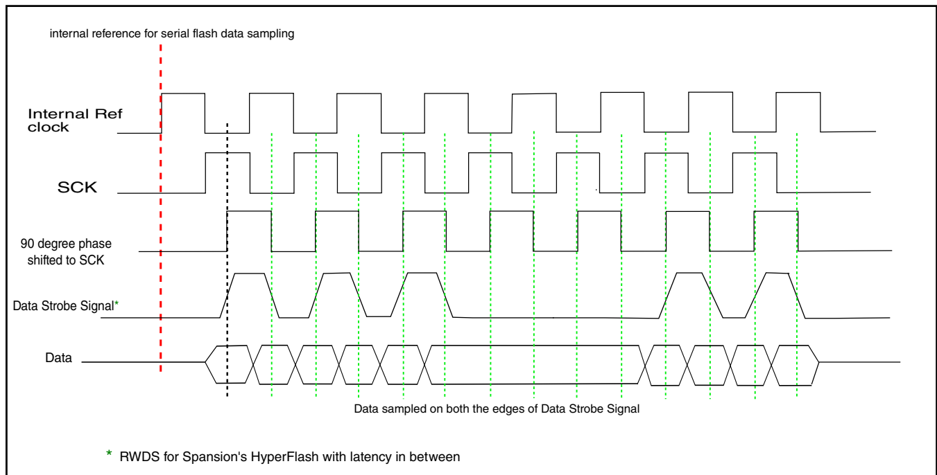
Figure 36-12. Data Strobe functionality with latency included
