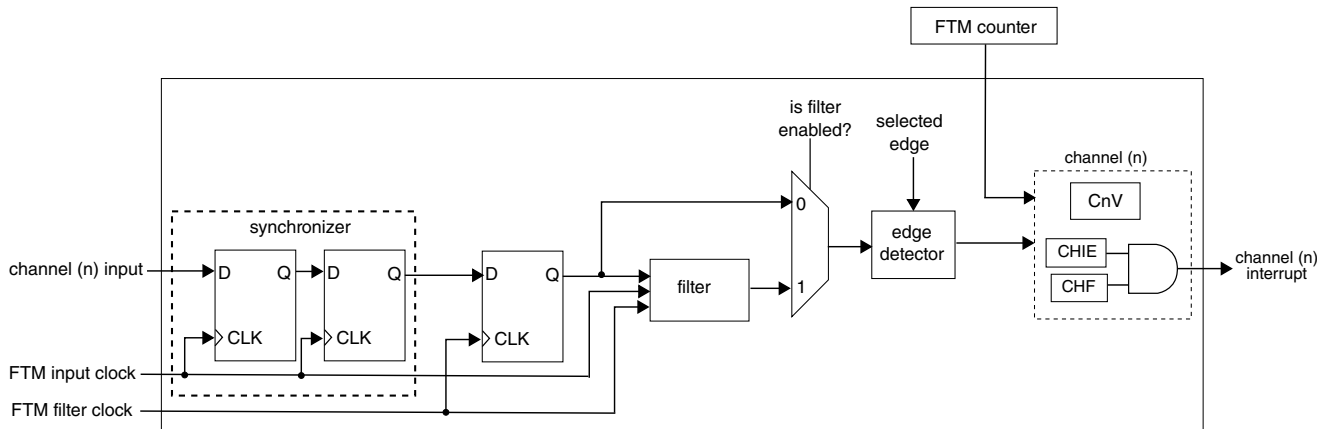
Figure 44-15. Diagram for Input Capture Mode when FLTPS[3:0] ≠ 0
