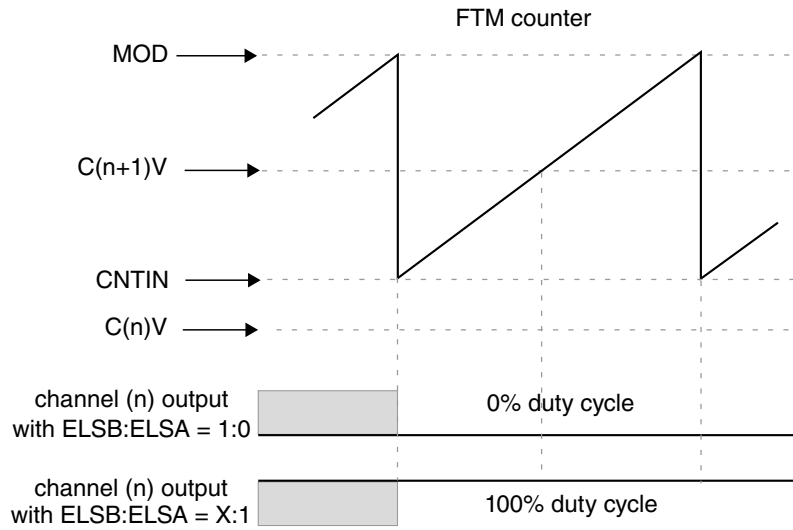
Figure 44-41. Channel (n) output if (C(n)V < CNTIN) and (CNTIN < C(n+1)V < MOD)
