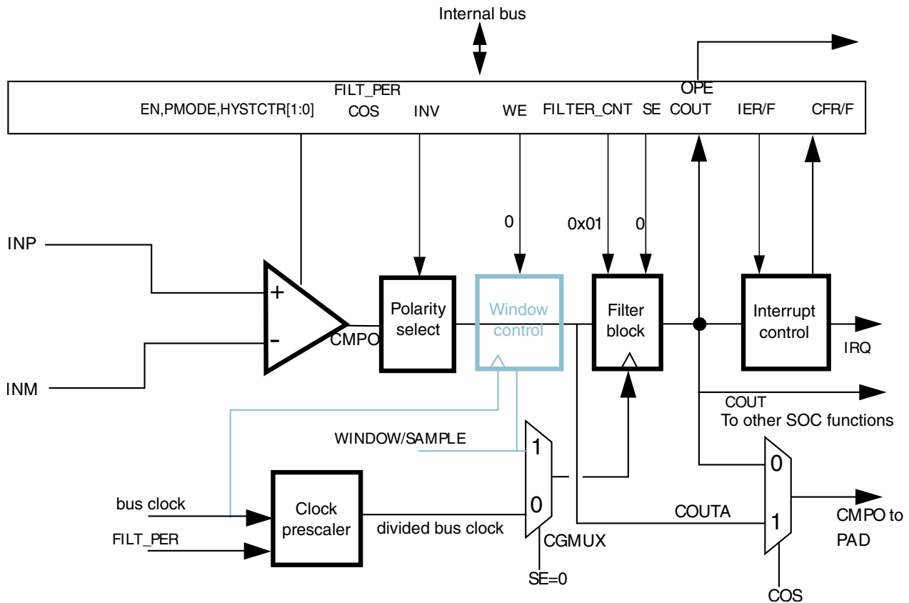
Figure 42-6. Sampled, Non-Filtered (# 3B): sampling interval internally derived
