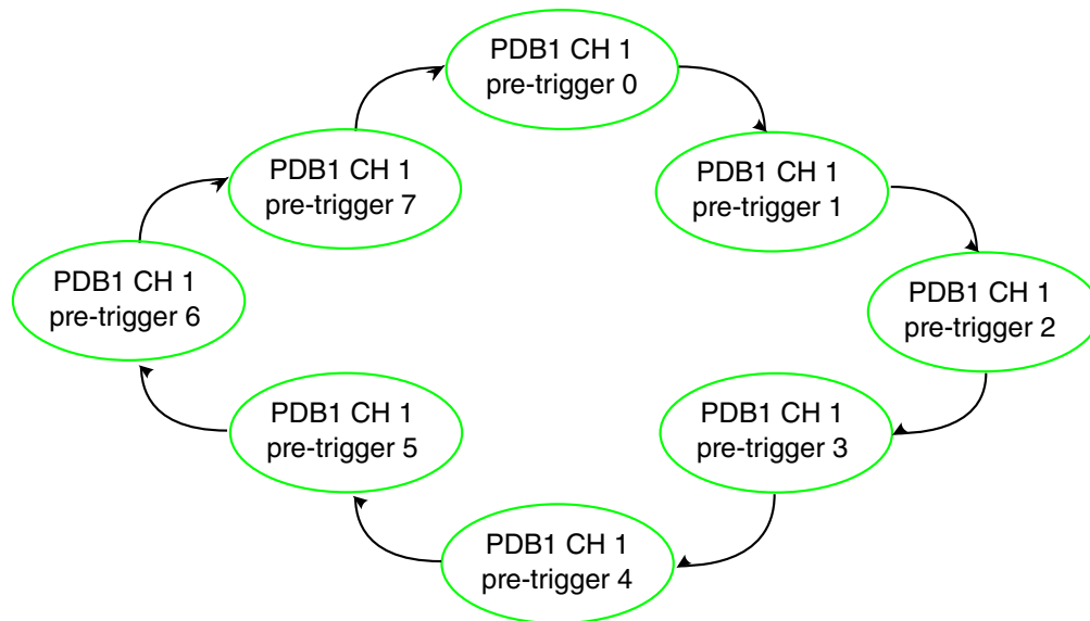
Figure 43-2. Example: PDB1 CH1 back-to-back chain
