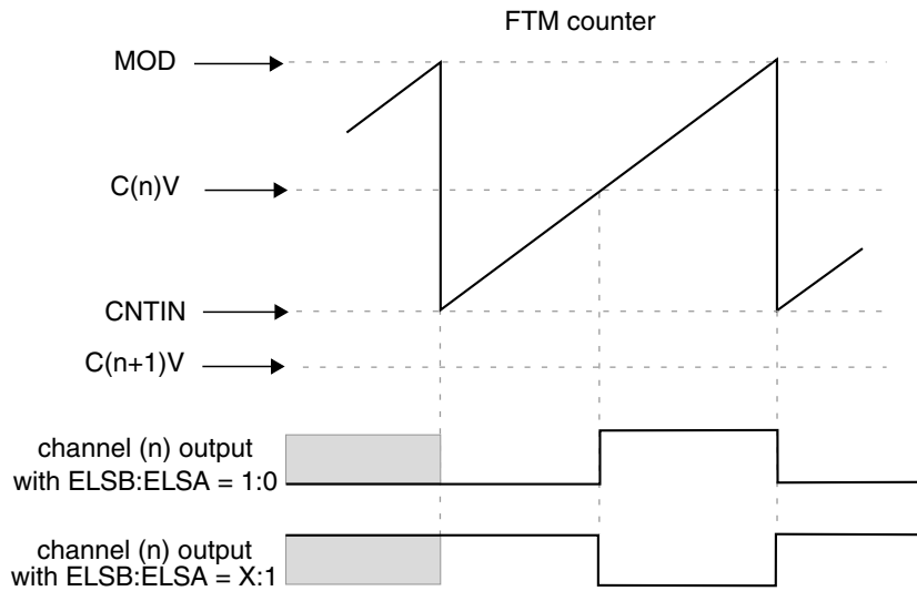
Figure 44-42. Channel (n) output if (C(n+1)V < CNTIN) and (CNTIN < C(n)V < MOD)
