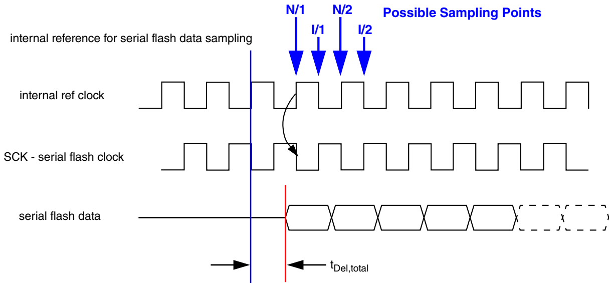
Figure 36-9. Internal sampling in SDR mode
