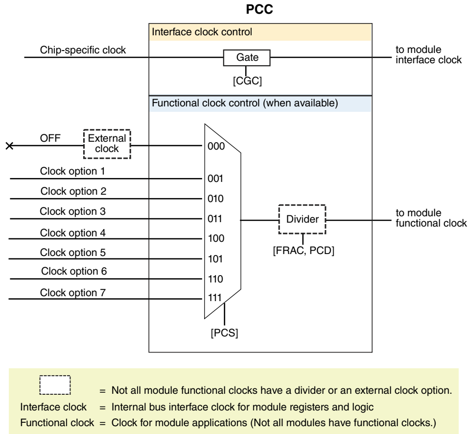
Figure 28-1. PCC Block Diagram
