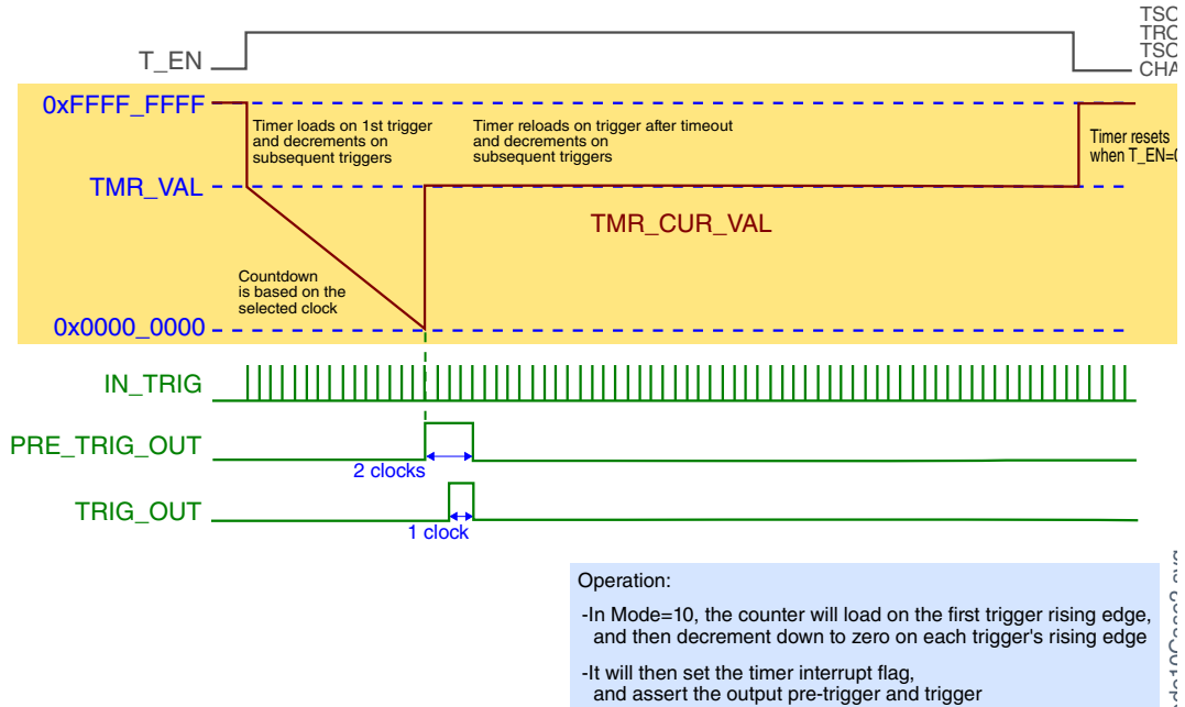
Figure 45-15. Case 2: TSOT = X, TROT = X, TSOI = 1, CHAIN = 0
