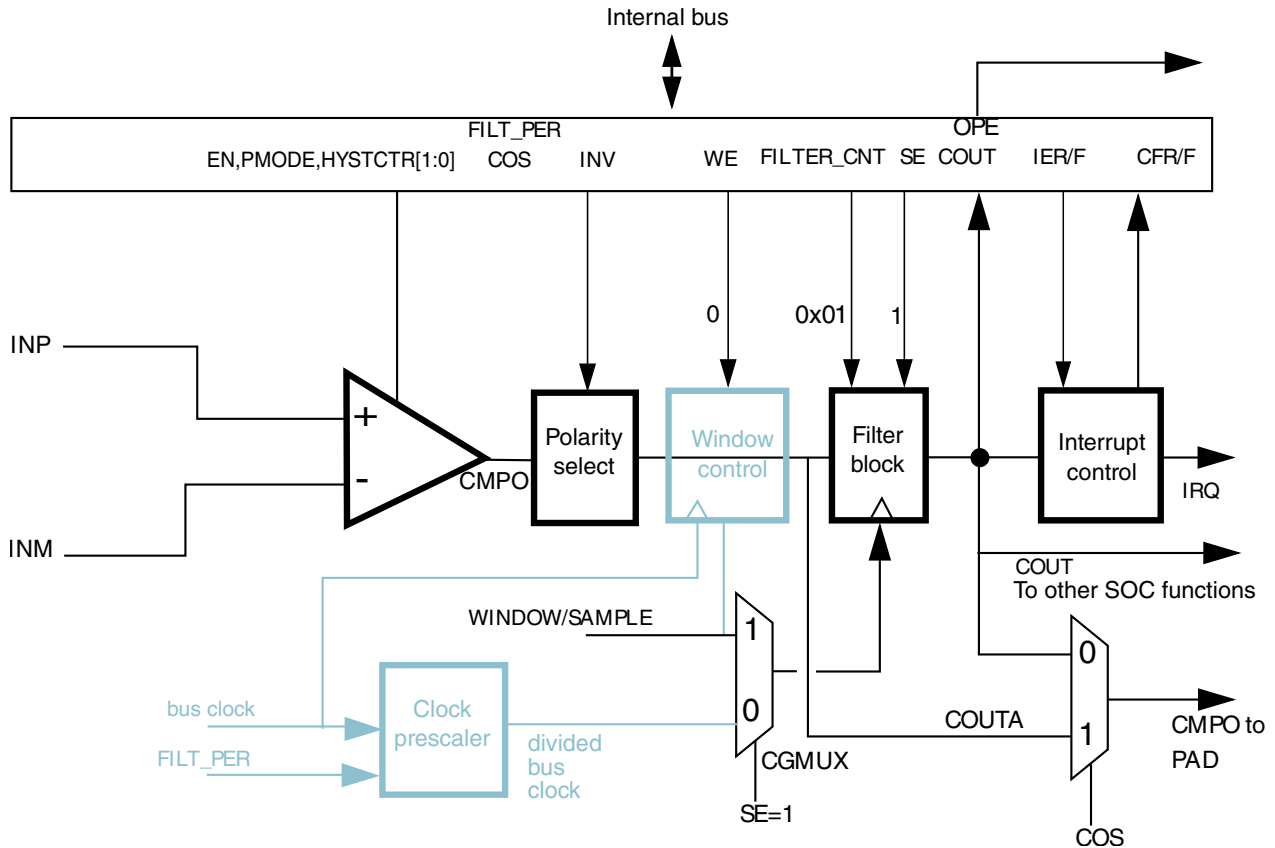
Figure 42-5. Sampled, Non-Filtered (# 3A): sampling point externally driven
