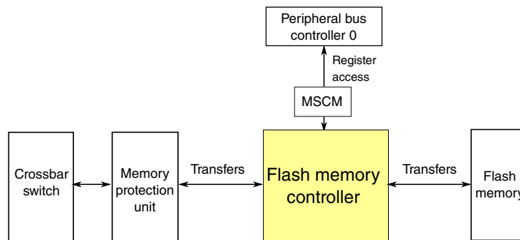
Figure 34-1. Flash Memory Controller configuration
