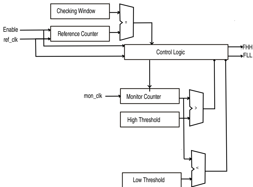
Figure 29-2. Block Diagram
