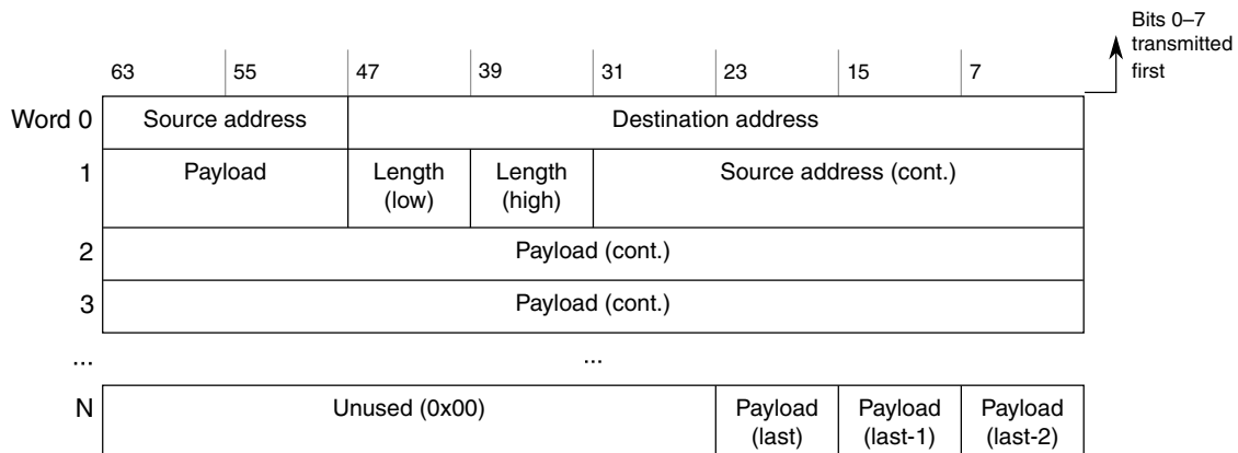
Figure 54-14. Normal Ethernet frame 64-bit mapping example
