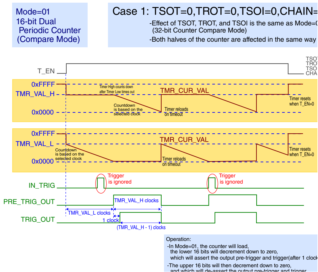
Figure 45-13. Case 1: TSOT = 0, TROT = 0, TSOI = 0, CHAIN = 0
