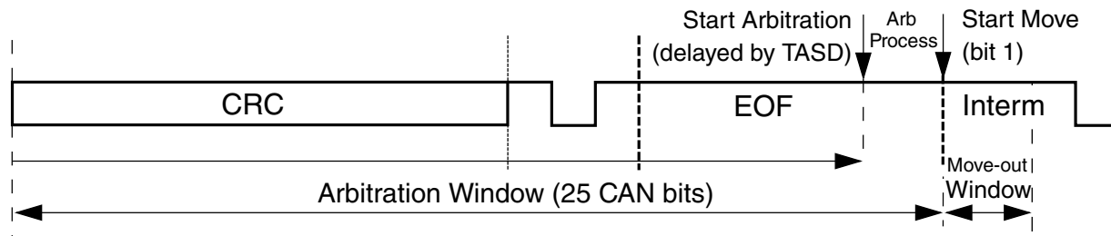
Figure 52-10. Arbitration and move-out time windows
