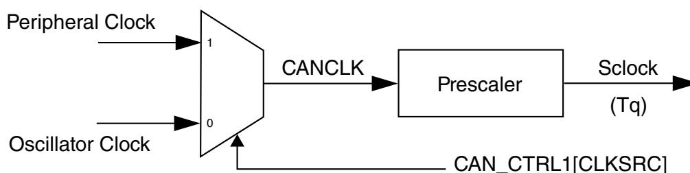
Figure 52-6. CAN engine clocking scheme
