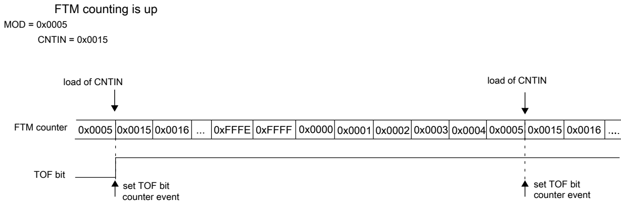
Figure 44-10. Example of up counting when the value of CNTIN is greater than the value of MOD
