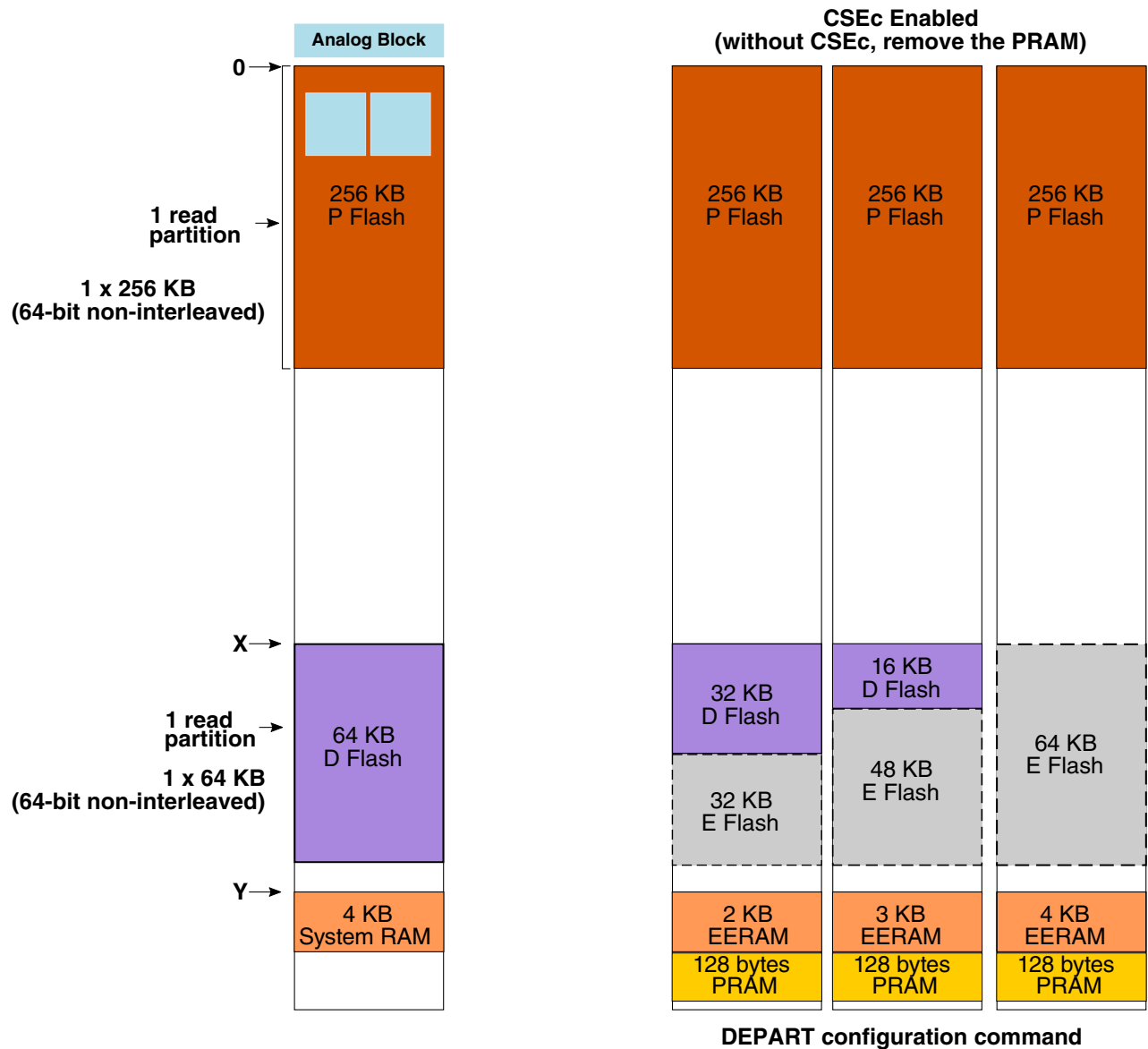
Figure 35-4. 256 KB flash memory map
