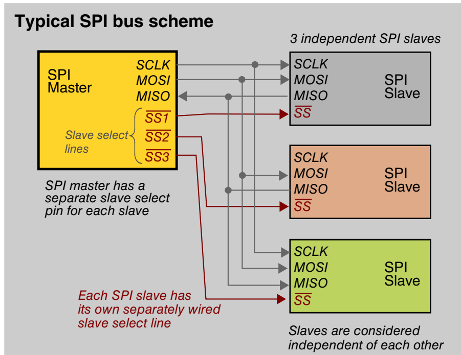
Figure 48-5. Dedicated slave select lines scheme
