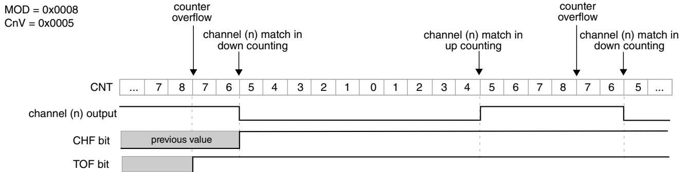
Figure 44-29. CPWM signal with ELSB:ELSA = X:1
