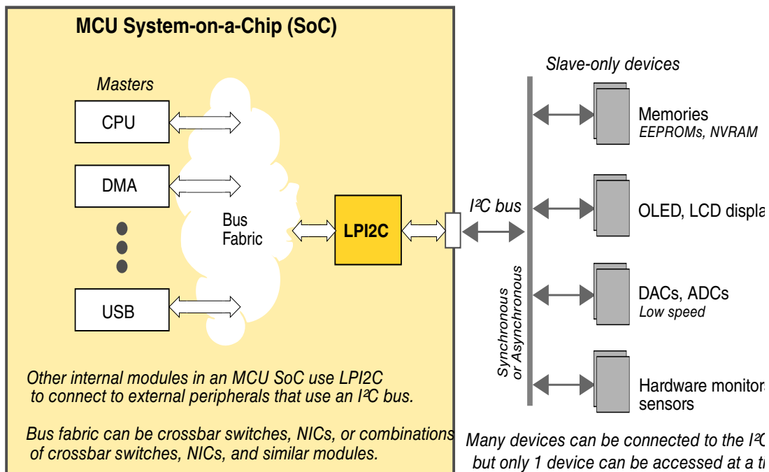
Figure 49-3. Typical LPI2C connection scheme
