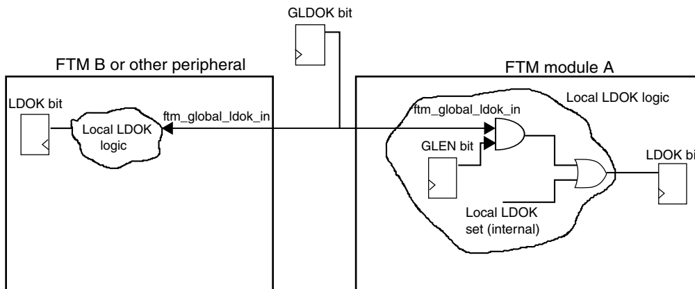
Figure 44-112. Global load logic
