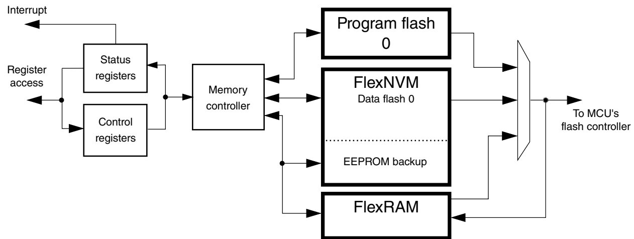
Figure 35-9. FTFC block diagram
