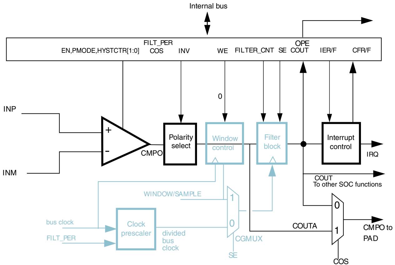
Figure 42-4. Comparator operation in Continuous mode
