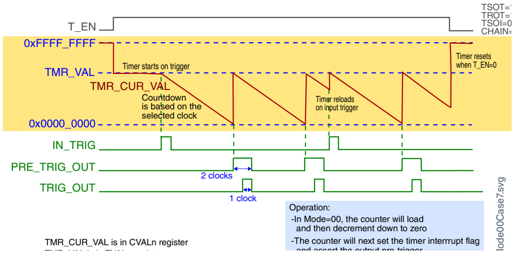
Figure 45-11. Case 7: TSOT = 1, TROT = 1, TSOI = 0, CHAIN = 0
