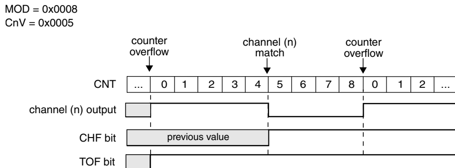
Figure 44-25. EPWM signal with ELSB:ELSA = 1:0
