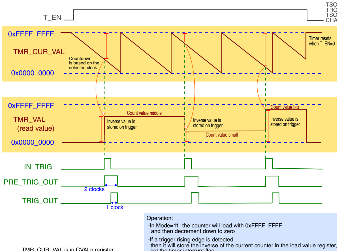
Figure 45-16. Case 1: TSOT = X, TROT = 0, TSOI = 0, CHAIN = 0
