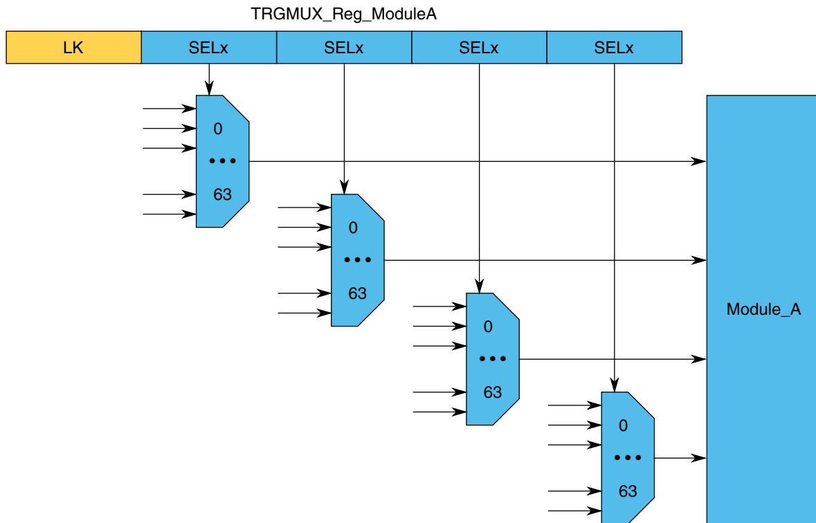
Figure 18-1. TRGMUX structure example (64 inputs)
