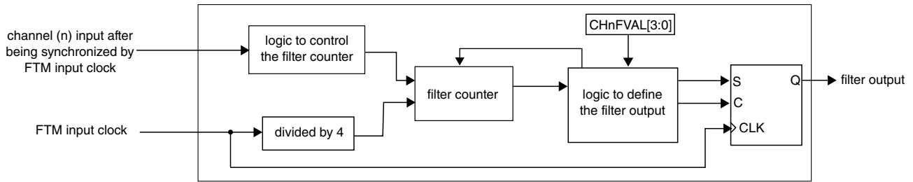
Figure 44-16. Channel Input Filter when FLTPS[3:0] = 0
