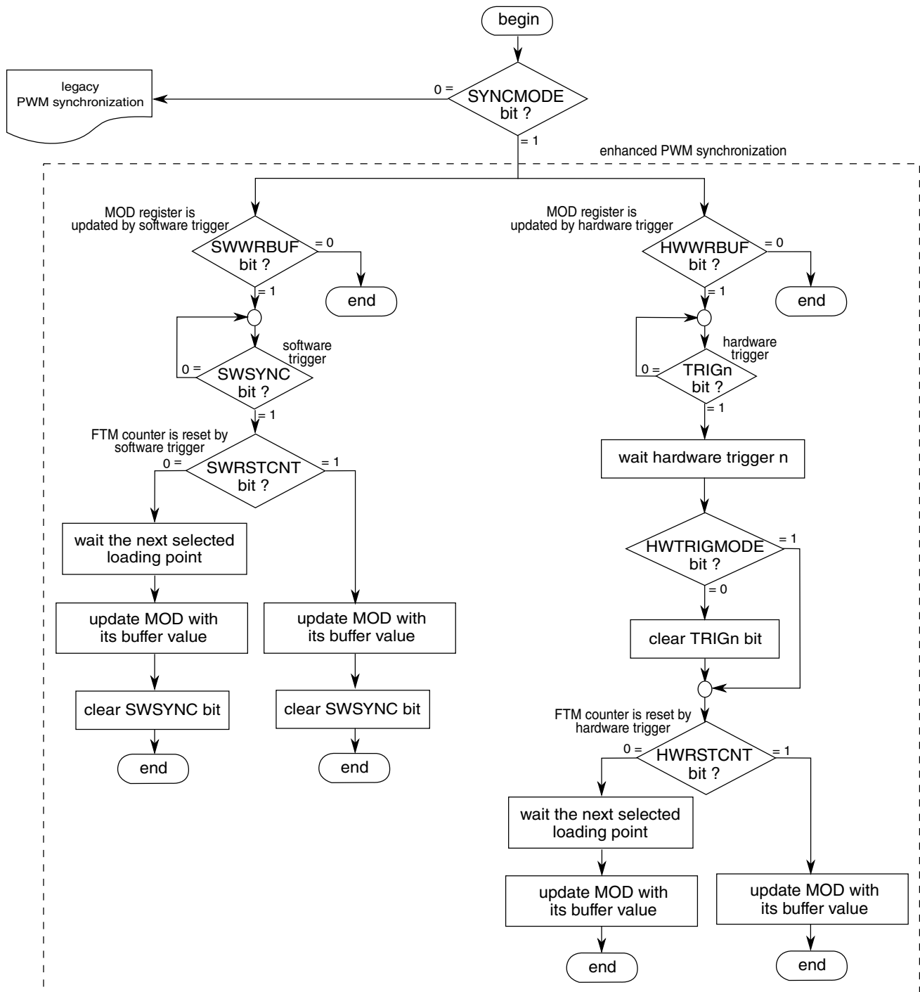
Figure 44-55. MOD register synchronization flowchart
