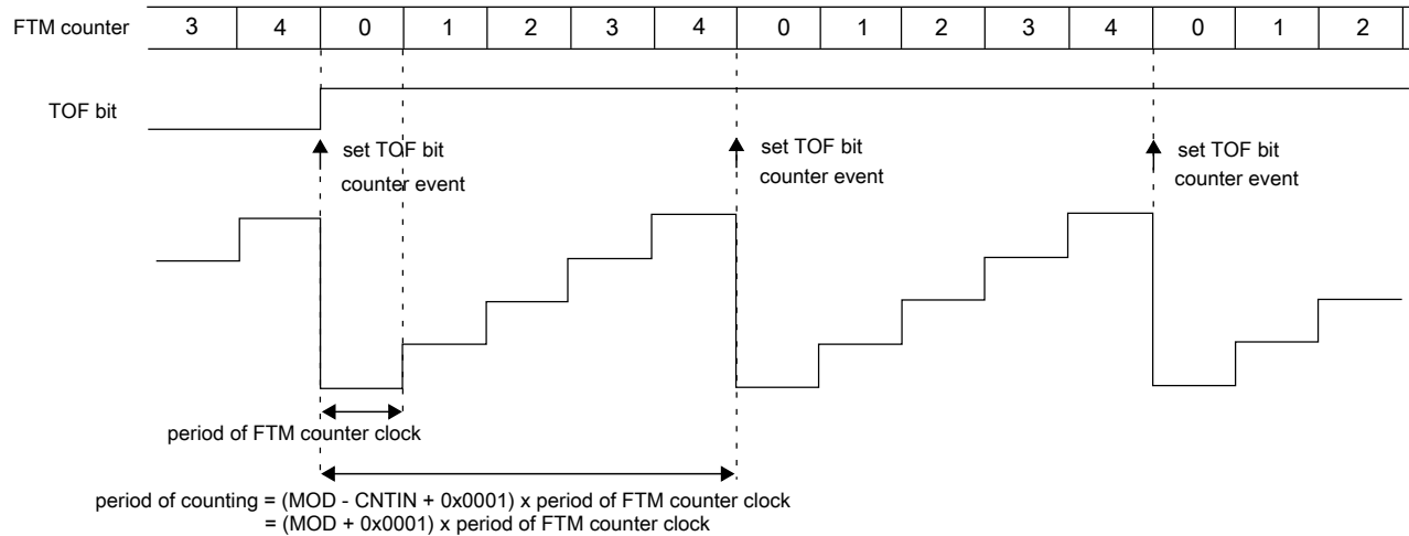
Figure 44-9. Example of FTM up counting with CNTIN = 0x0000
