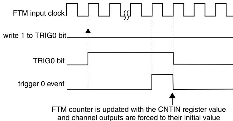
Figure 44-71. FTM counter synchronization with (SYNCMODE = 0), (HWTRIGMODE = 0), (REINIT = 1), (PWMSYNC = 1), and a hardware trigger was used
