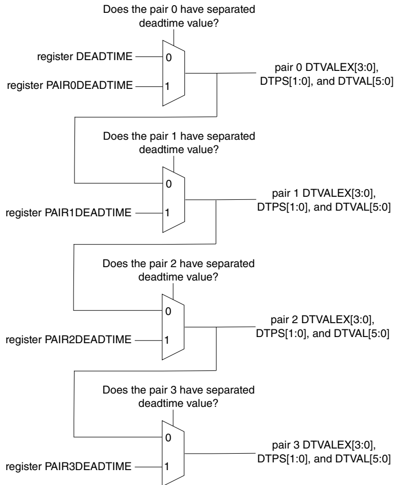
Figure 44-77. Separated Deadtime by Pair of Channels
