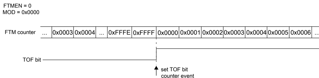
Figure 44-13. Example when the FTM counter is free running
