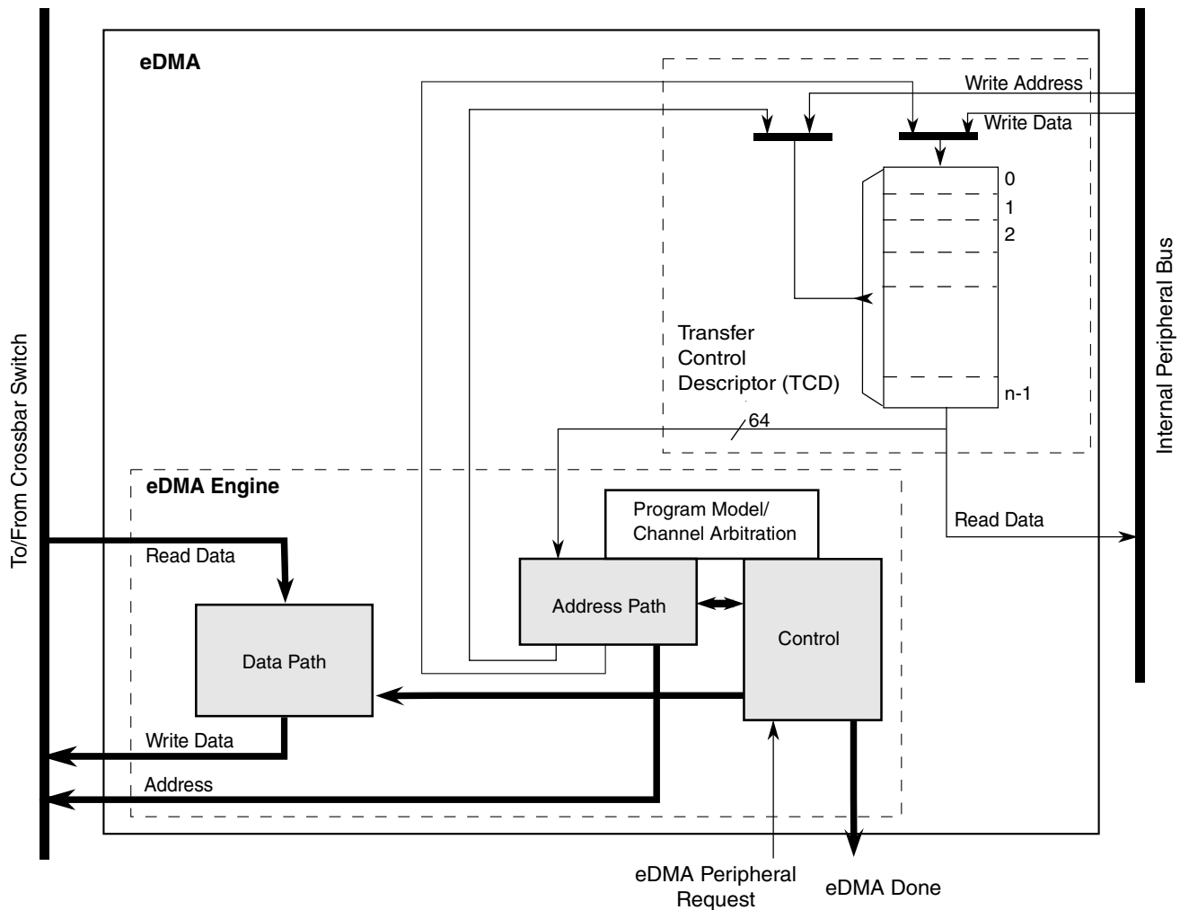
Figure 17-3. eDMA operation, part 2
