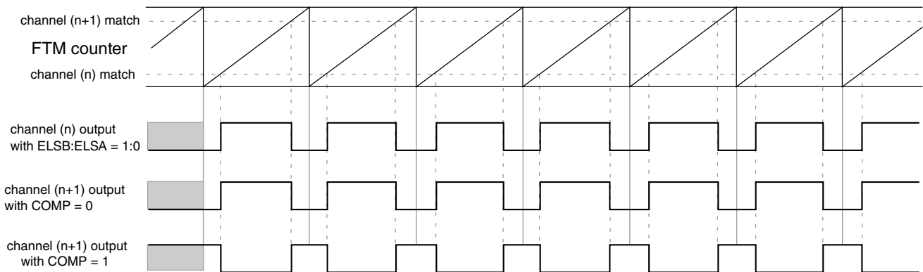
Figure 44-50. Channel (n+1) output in Complementary mode with (ELSB:ELSA = 1:0)
