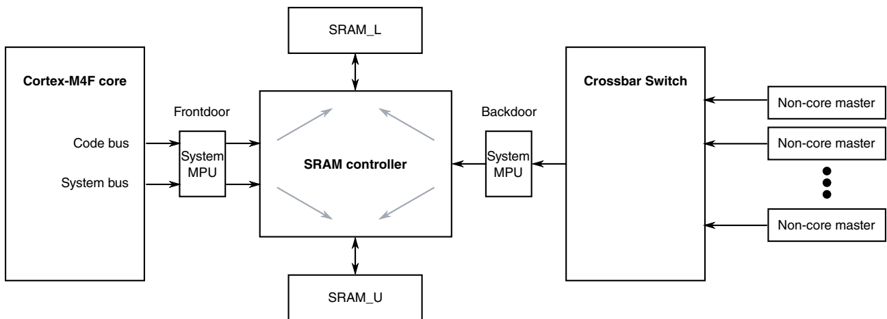
Figure 30-1. SRAM accessibility
