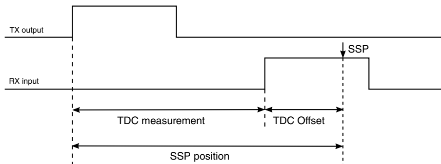
Figure 52-5. SSP position with optimal values
