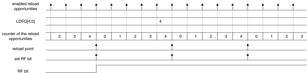
Figure 44-111. Frequency of Reload Opportunities with LDFQ[4:0] = 4
