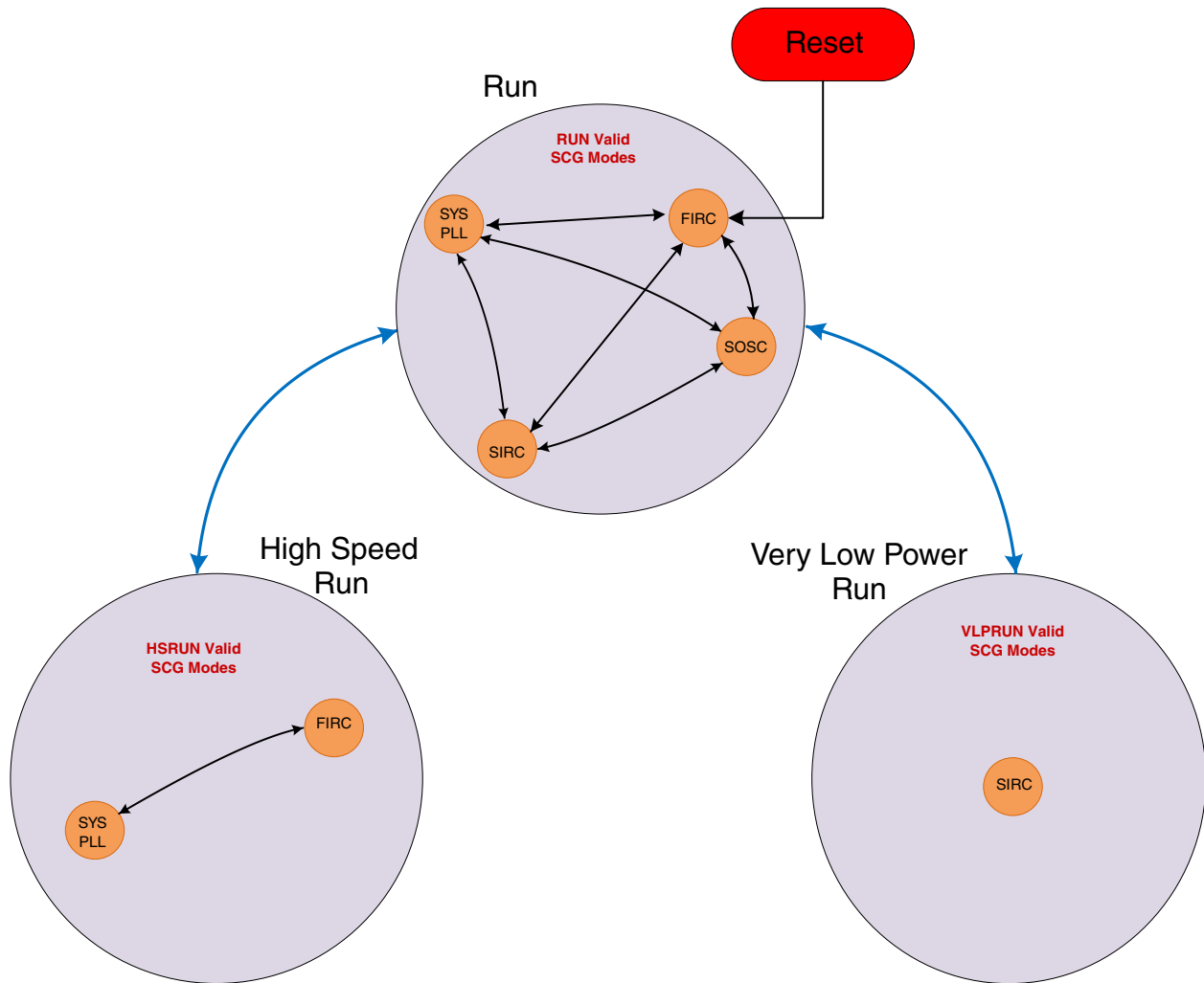
Figure 27-1. SCG Valid Mode Transition Diagram
