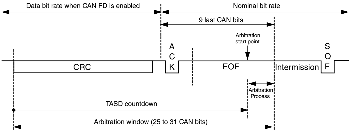
Figure 52-12. Optimal Tx Arbitration start point
