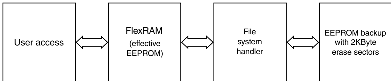
Figure 35-13. Top-level emulated EEPROM architecture
