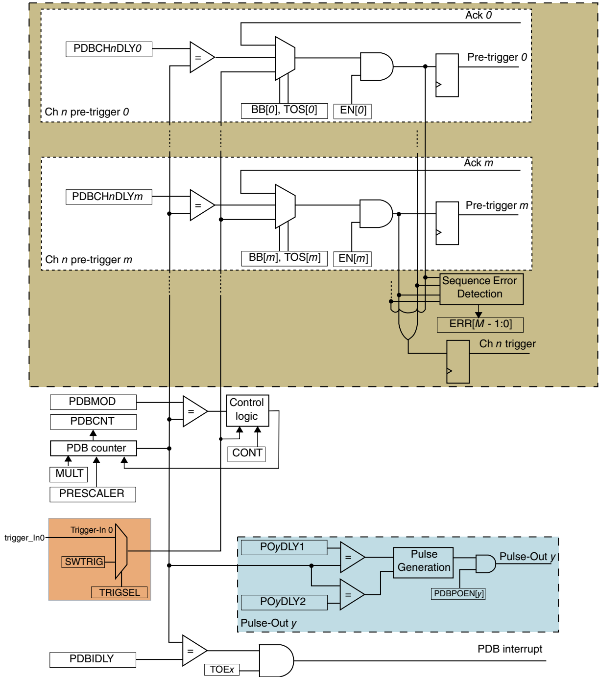
Figure 43-6. PDB block diagram
