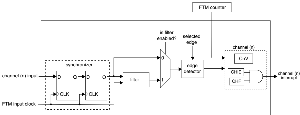
Figure 44-14. Diagram for Input Capture Mode when FLTPS[3:0] = 0
