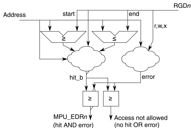
Figure 14-2. MPU access evaluation macro
