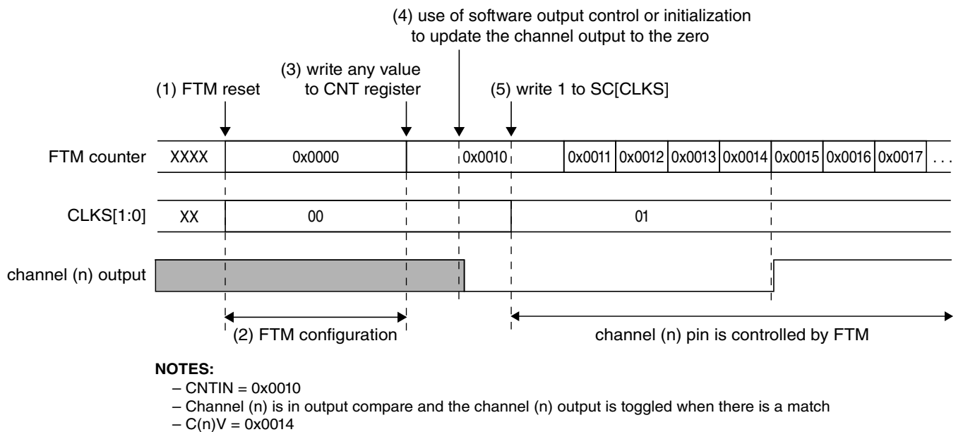
Figure 44-128. FTM behavior after reset when the channel (n) is in Output Compare mode
