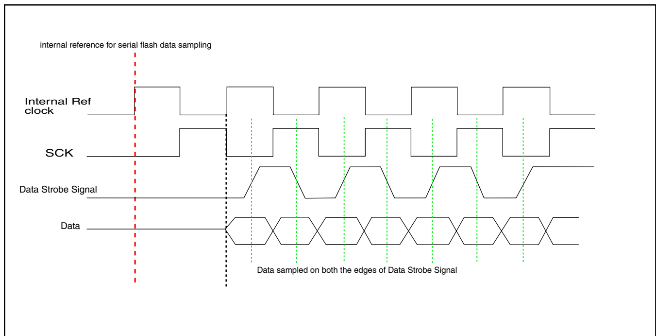
Figure 36-11. Data Strobe functionality in DDR mode
