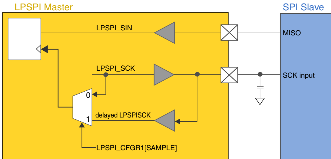
Figure 48-7. Clock Loopback
