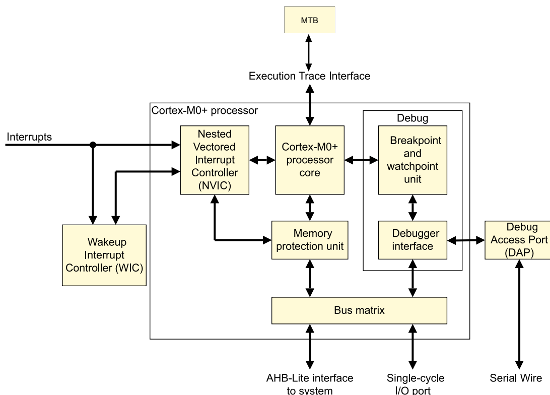
Figure 55-2. Cortex-M0+ debug topology
