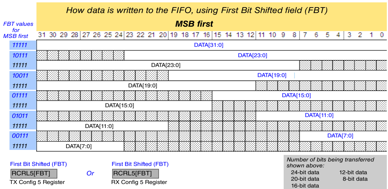
Figure 53-3. SAI first bit shifted, MSB first
