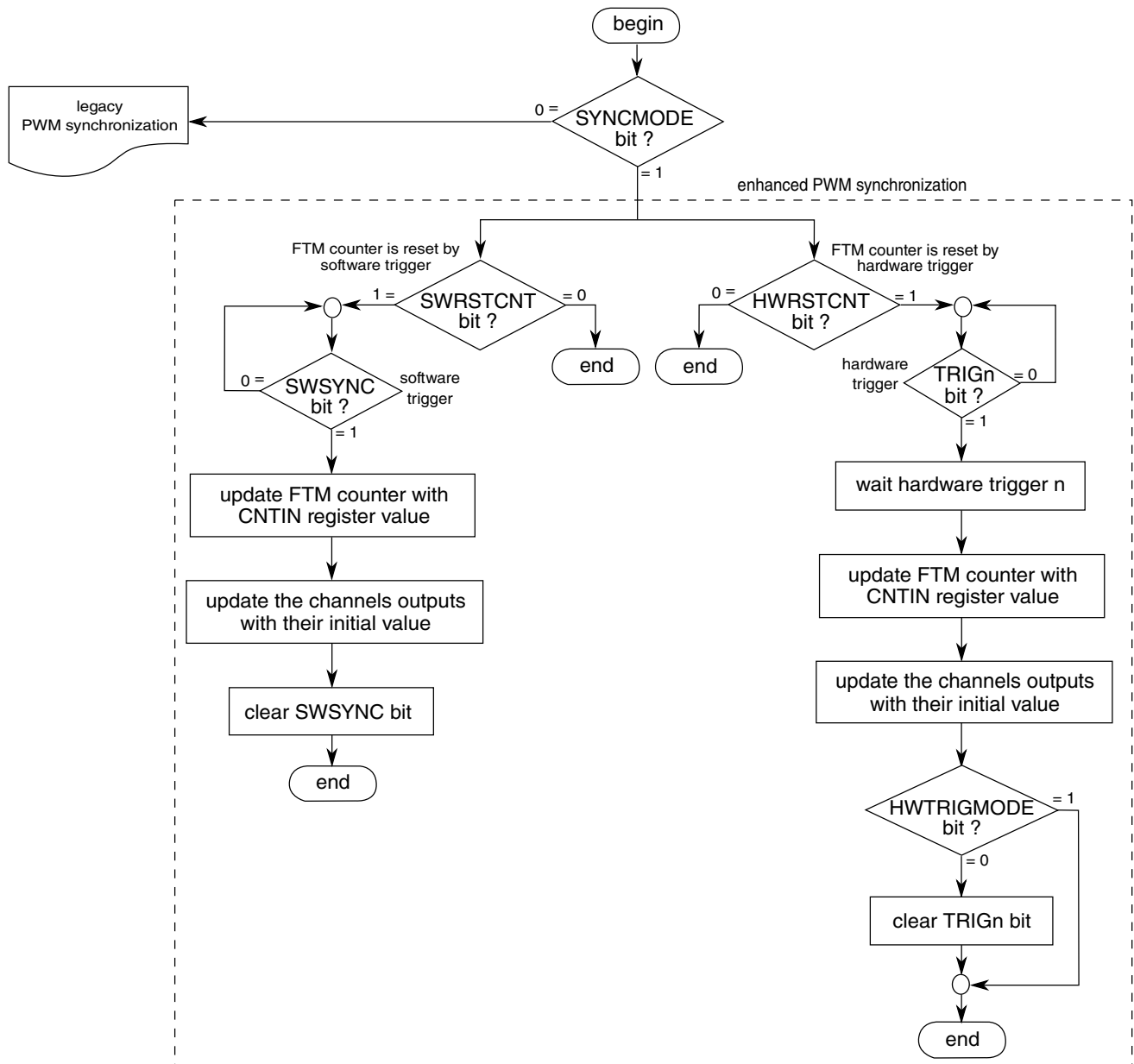
Figure 44-68. FTM counter synchronization flowchart
