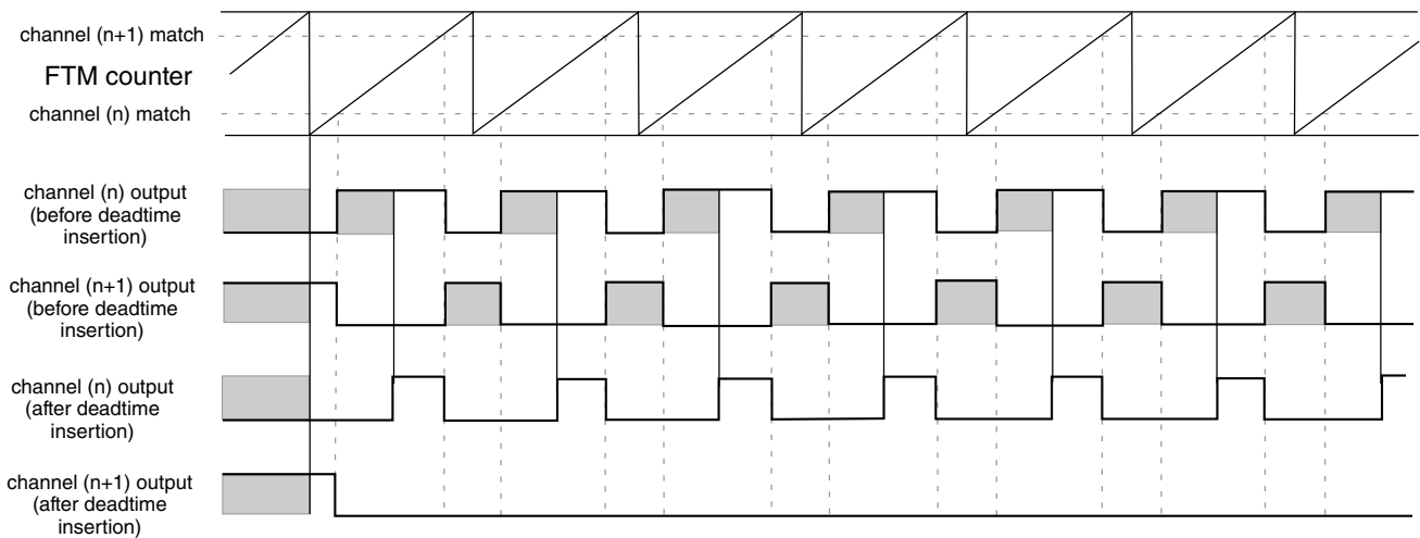
Figure 44-78. Example of the deadtime insertion (channel (n) ELSB:ELSA = 1:0, POL(n) = 0, and POL(n+1) = 0) when the deadtime delay is comparable to channel (n+1) duty cycle
