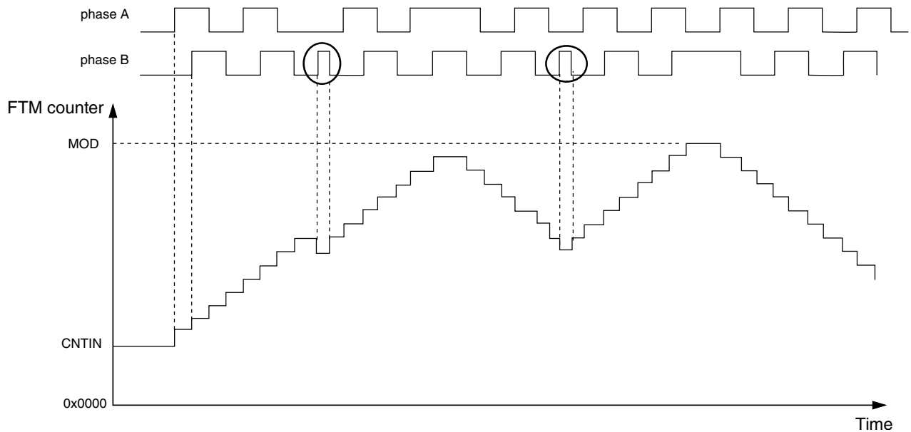
Figure 44-107. Motor position jittering in a mid count value
