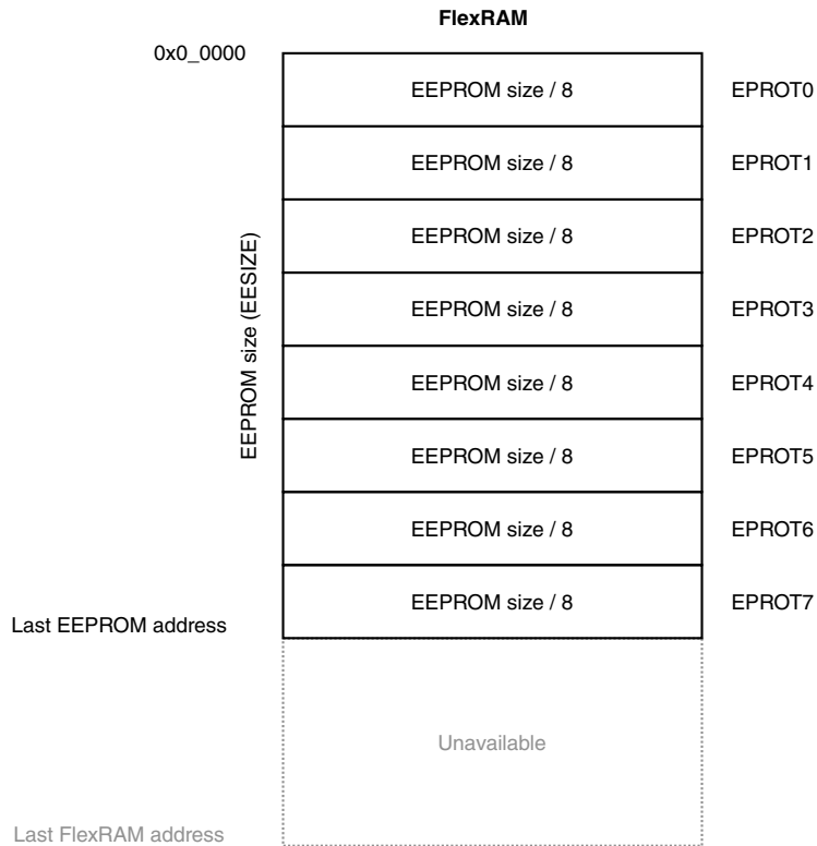
Figure 35-12. EEPROM protection
