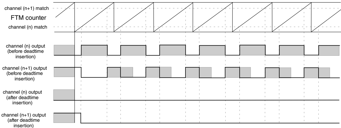
Figure 44-79. Example of the deadtime insertion (channel (n) ELSB:ELSA = 1:0, POL(n) = 0, and POL(n+1) = 0) when the deadtime delay is comparable to channels (n) and (n+1) duty cycle
