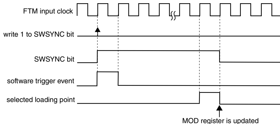
Figure 44-60. MOD synchronization with (SYNCMODE = 0) and (PWMSYNC = 1)
