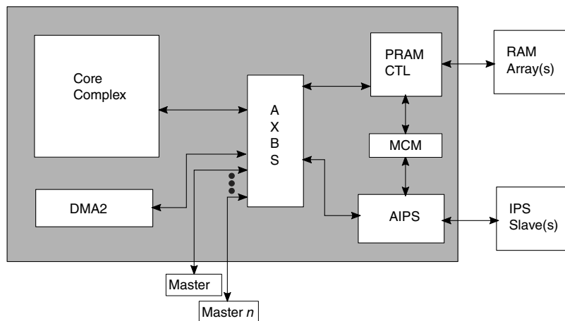
Figure 31-1. Simplified block diagram
