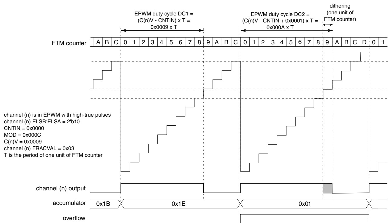
Figure 44-120. Channel (n) is in EPWM Mode with PWM Edge Dithering
