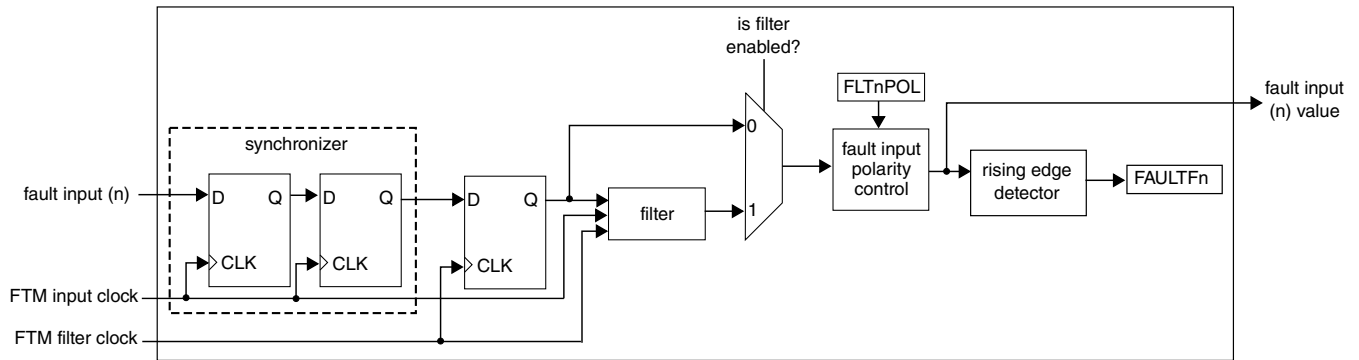
Figure 44-82. Diagram for Fault Control when FLTPS[3:0] ≠ 0
