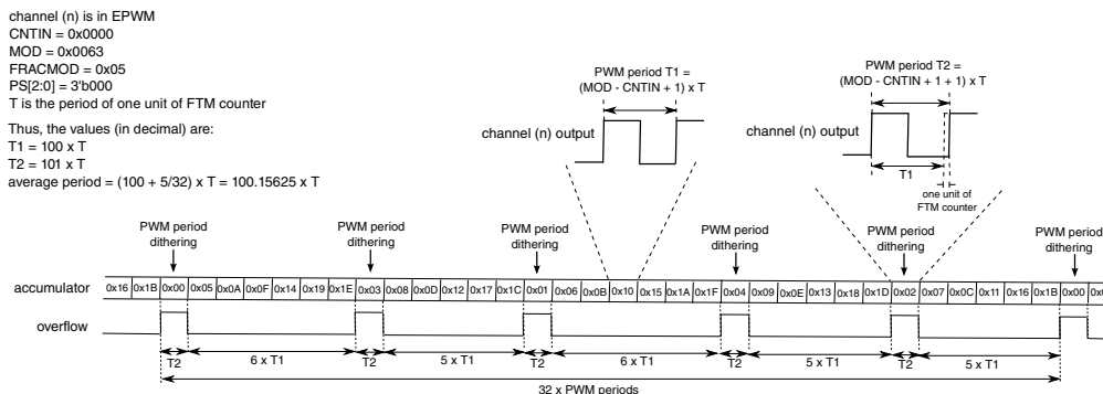
Figure 44-118. Example of Average Period when the PWM Period Dithering is used with the Up Counting
