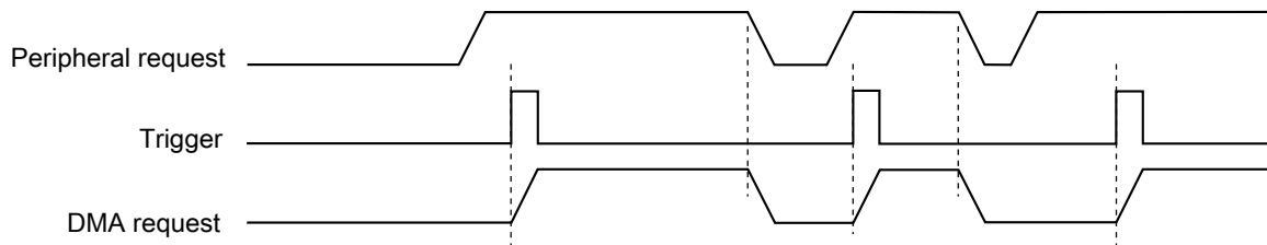
Figure 16-3. DMAMUX channel triggering: normal operation
