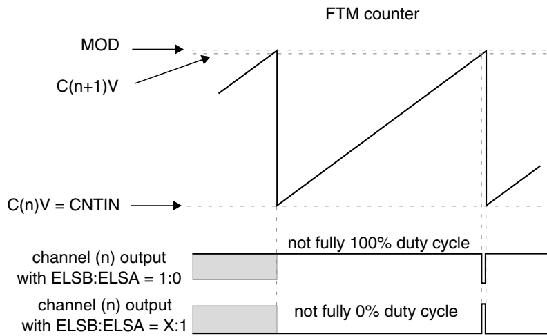
Figure 44-35. Channel (n) output if (C(n)V = CNTIN) and (CNTIN < C(n+1)V < MOD) and (C(n+1)V is Almost Equal to MOD )
