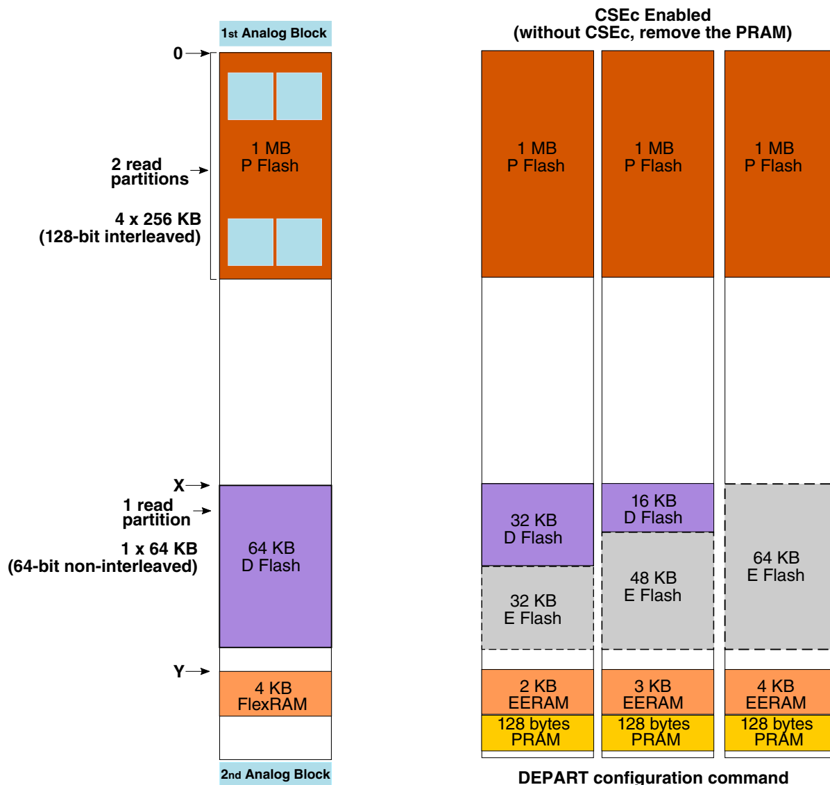
Figure 35-6. 1 MB flash memory map
