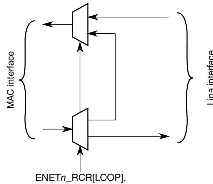
Figure 54-13. Loopback options
