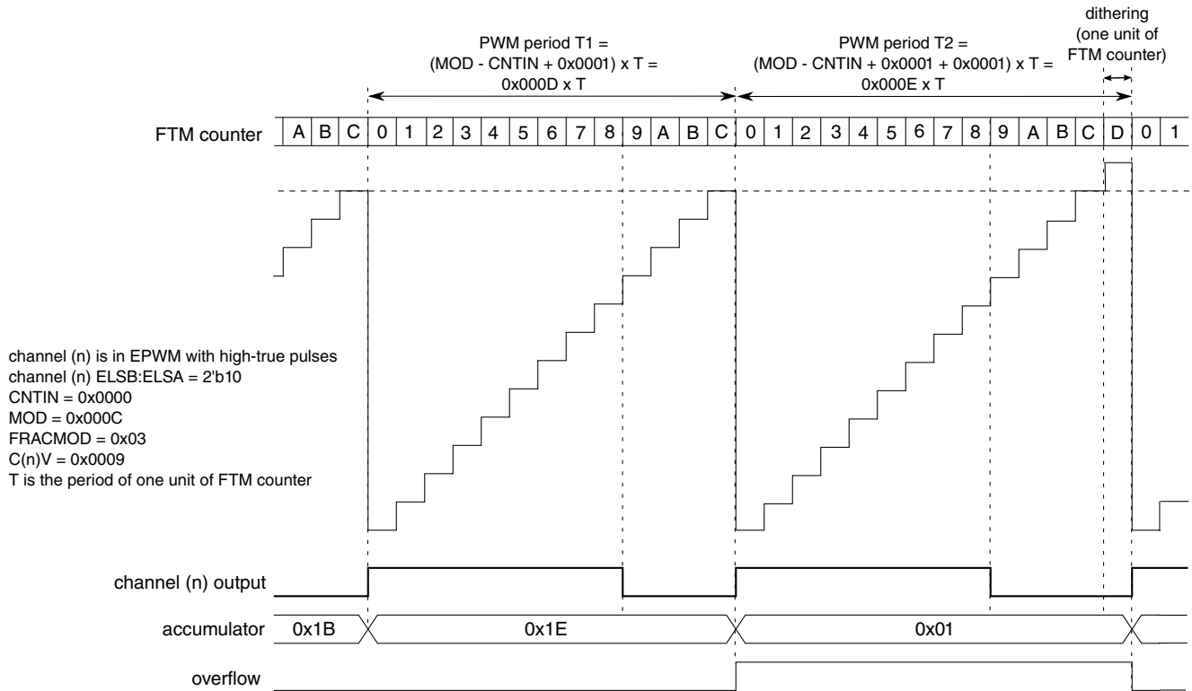
Figure 44-117. PWM Period Dithering with Up Counting
