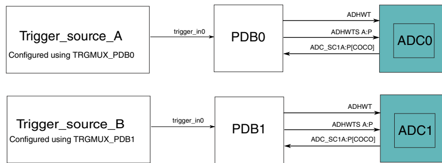
Figure 40-3. ADCs triggering with independent sources
