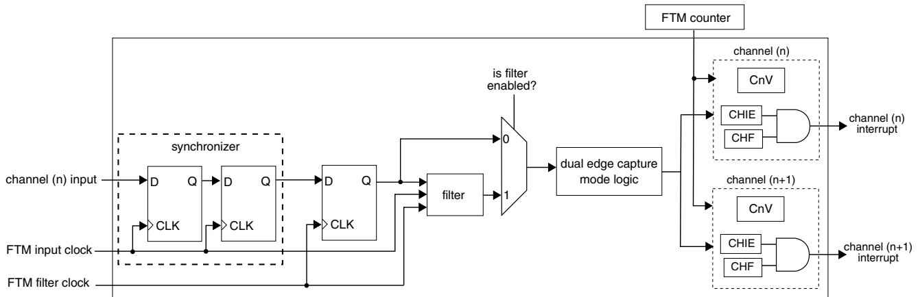
Figure 44-95. Diagram for Dual Edge Capture Mode when FLTPS[3:0] ≠ 0
