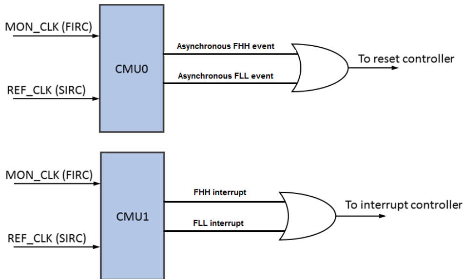
Figure 29-1. CMU on chip
