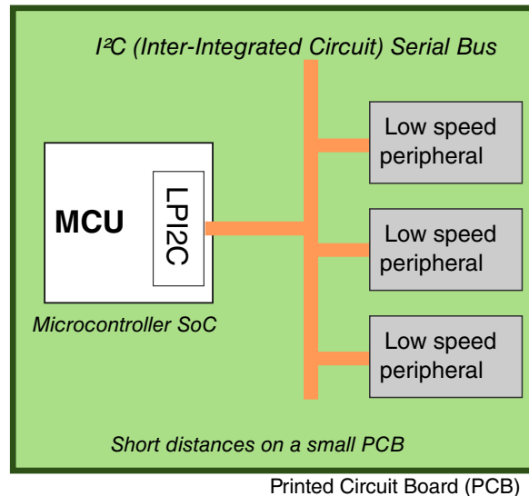
Figure 49-1. I 2 C bus connects MCU to low speed peripherals on PCB
