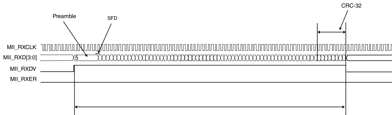
Figure 54-25. MII receive operation
