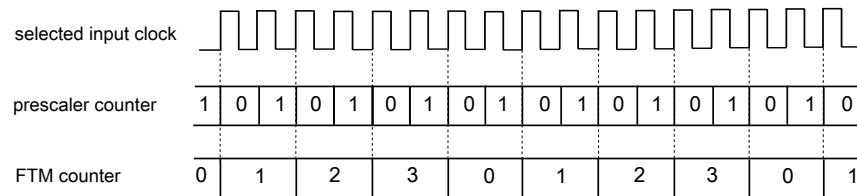
Figure 44-7. Example of the prescaler counter
