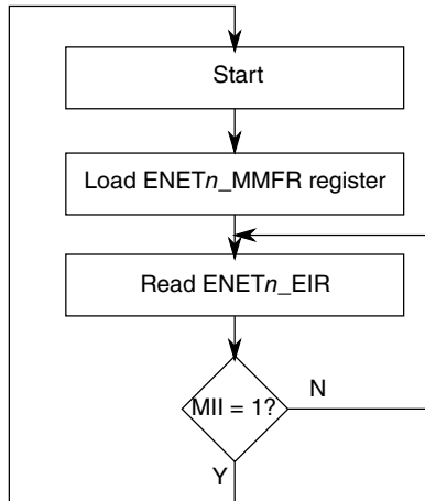
Figure 54-18. MDIO access overview
