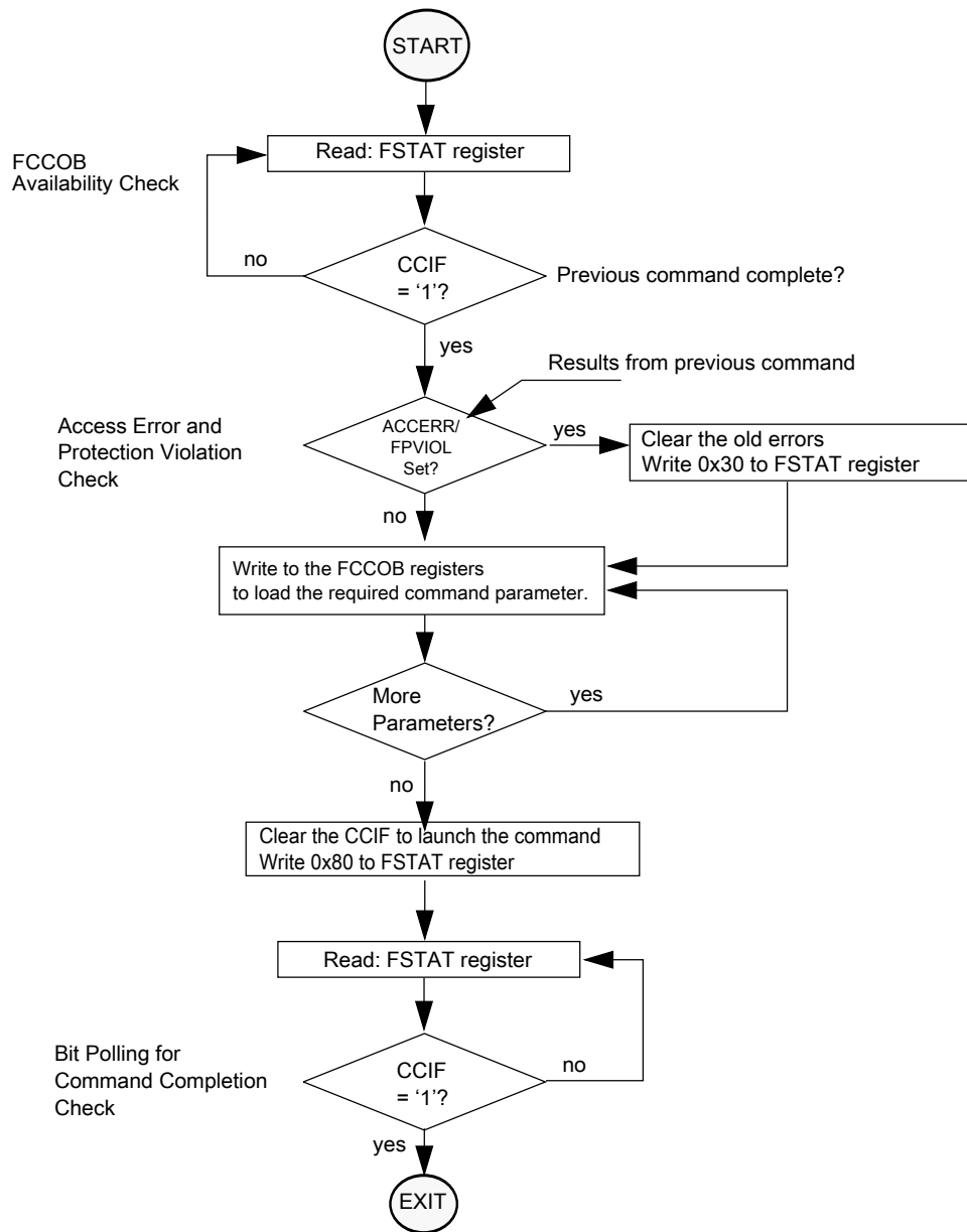
Figure 35-14. Generic flash command write sequence flowchart
