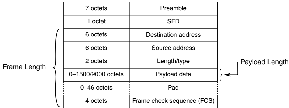
Figure 54-2. MAC frame format overview
