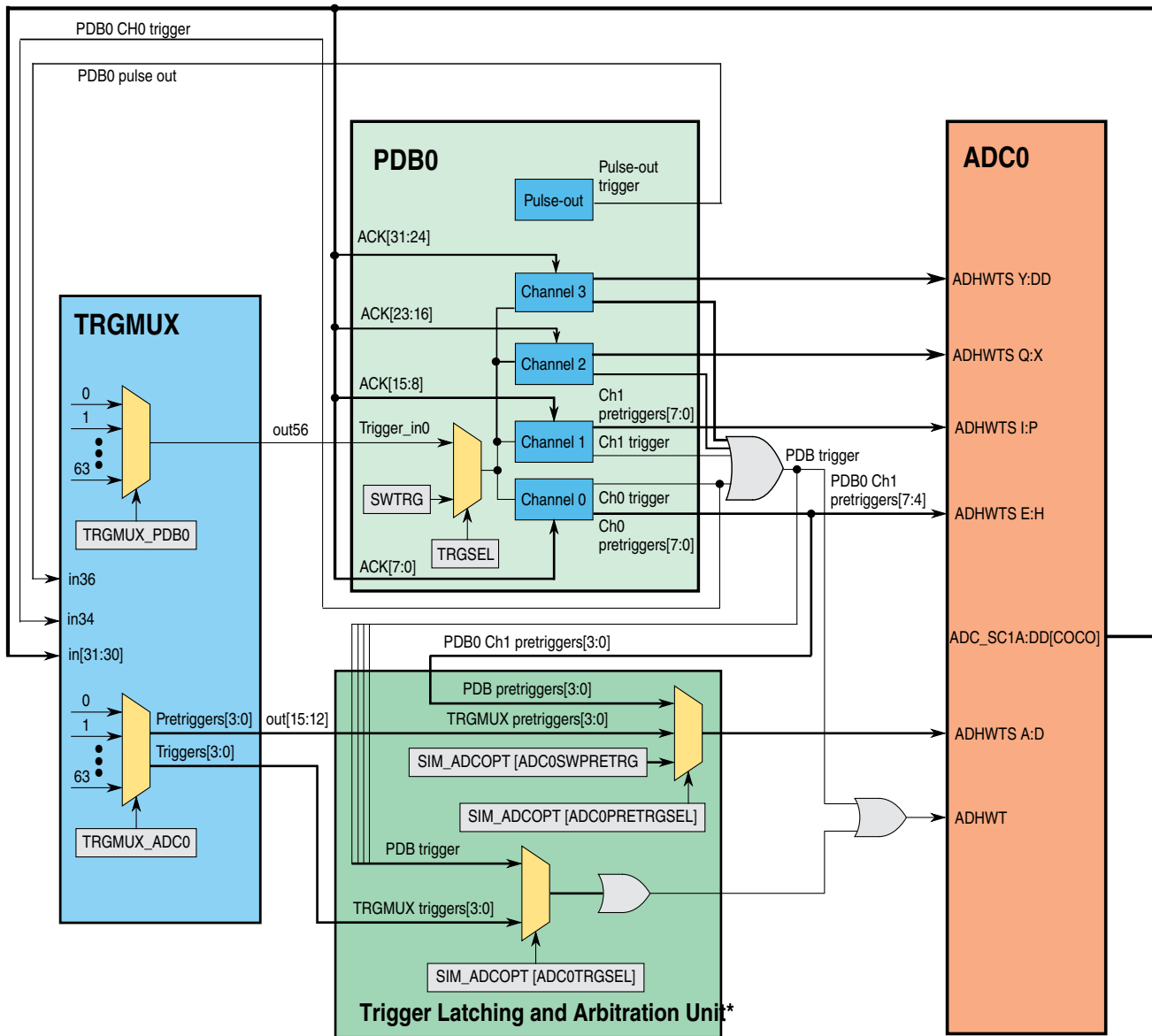
Figure 40-2. ADC0_PDB0 ADC Triggering scheme example
