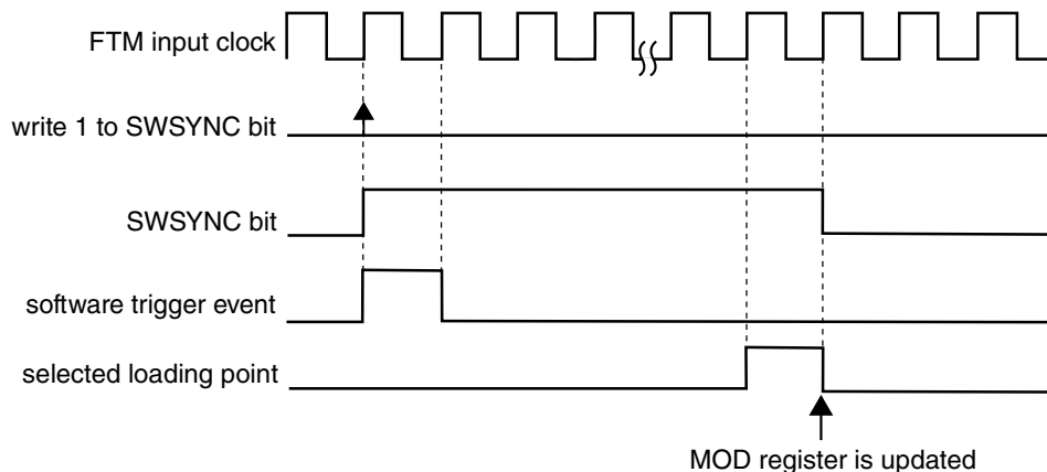
Figure 44-56. MOD synchronization with (SYNCMODE = 0), (PWMSYNC = 0), (REINIT = 0), and software trigger was used
