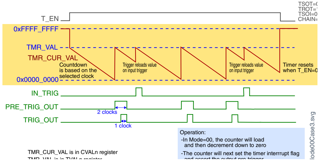
Figure 45-7. Case 3: TSOT = 0, TROT = 1, TSOI = 0, CHAIN = 0
