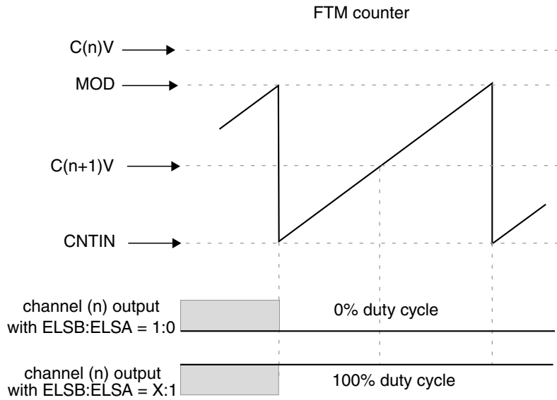
Figure 44-43. Channel (n) output if (C(n)V > MOD) and (CNTIN < C(n+1)V < MOD)
