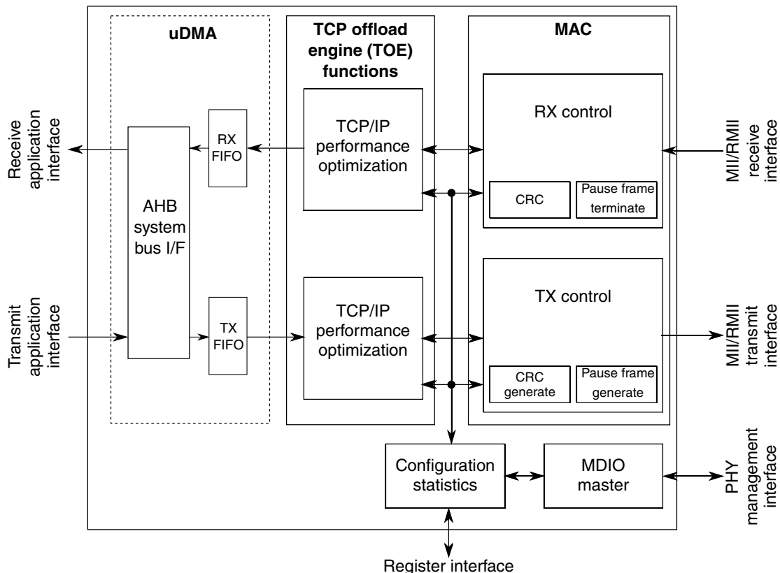
Figure 54-1. Ethernet MAC-NET core block diagram
