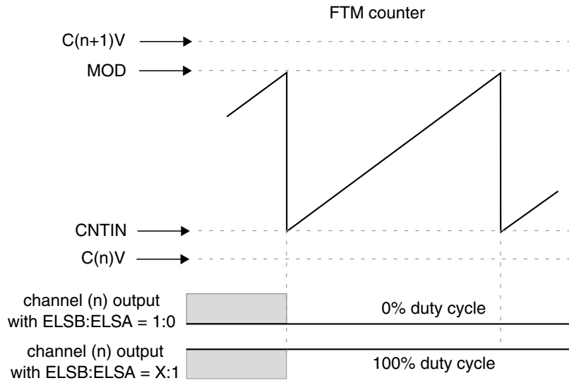
Figure 44-36. Channel (n) output if C(n)V and C(n+1)V are not between CNTIN and MOD
