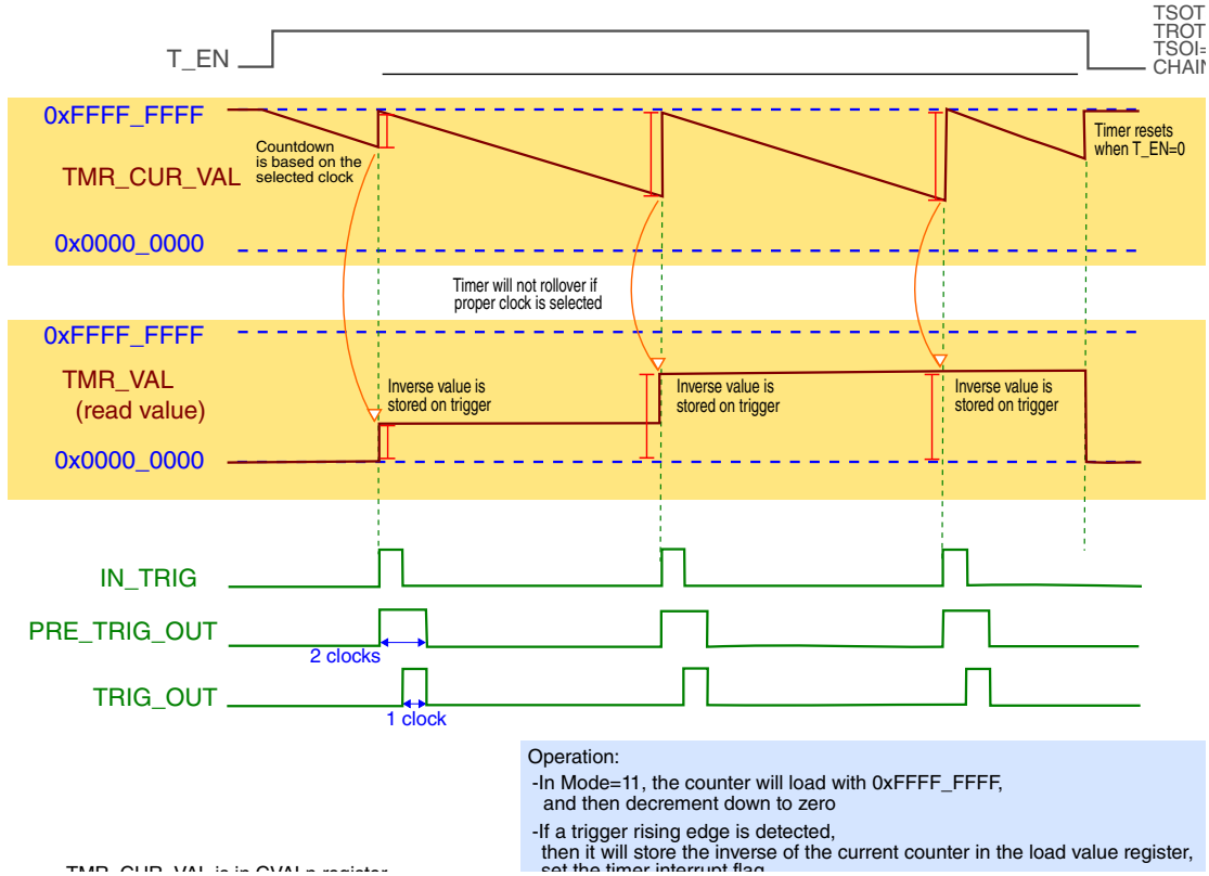
Figure 45-17. Case 2: TSOT = X, TROT = 1, TSOI = 0, CHAIN = 0
