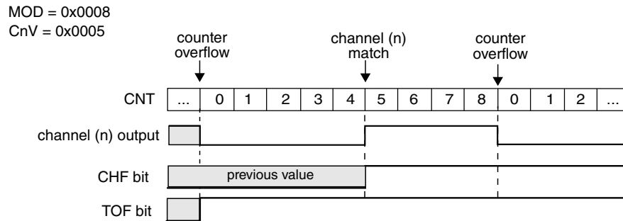
Figure 44-26. EPWM signal with ELSB:ELSA = X:1
