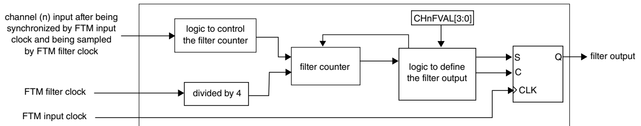
Figure 44-17. Channel Input Filter when FLTPS[3:0] \neq 0
