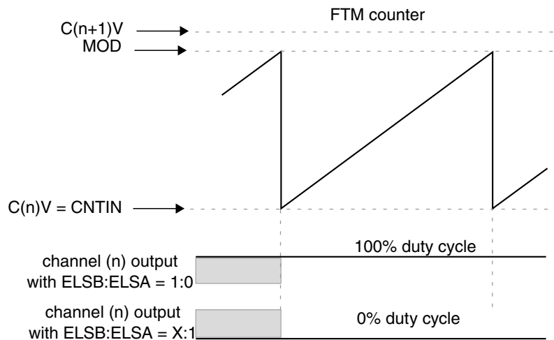
Figure 44-46. Channel (n) output if (C(n)V = CNTIN) and (C(n+1)V > MOD)
