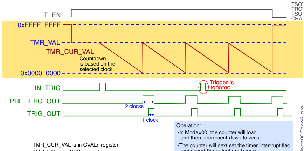
Figure 45-9. Case 5: TSOT = 1, TROT = 0, TSOI = 0, CHAIN = 0
