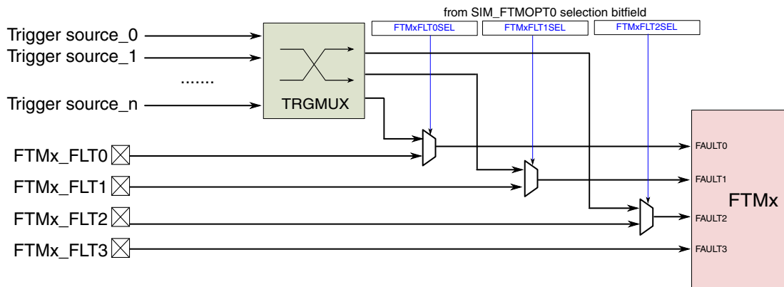
Figure 44-1. Fault detection inputs
