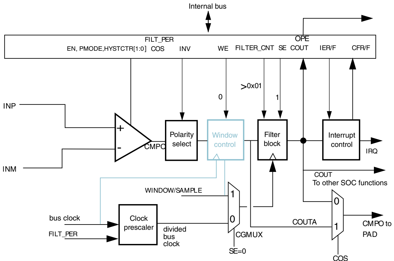
Figure 42-8. Sampled, Filtered (# 4B): sampling point internally derived
