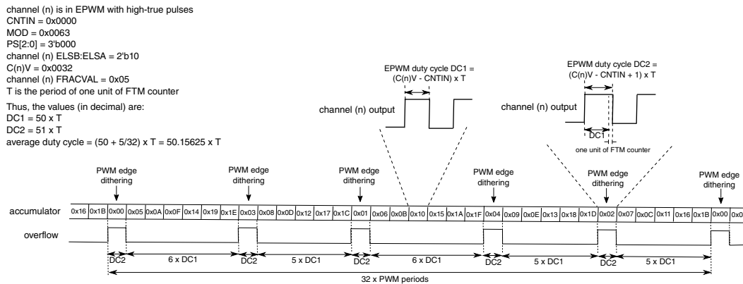
Figure 44-121. Example of Average Duty Cycle when the Channel (n) is in EPWM Mode with PWM Edge Dithering
