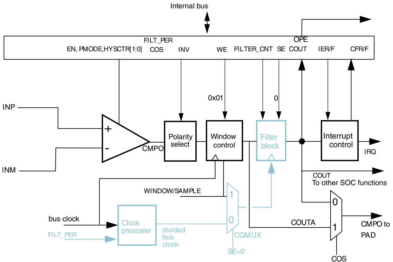
Figure 42-10. Windowed mode
