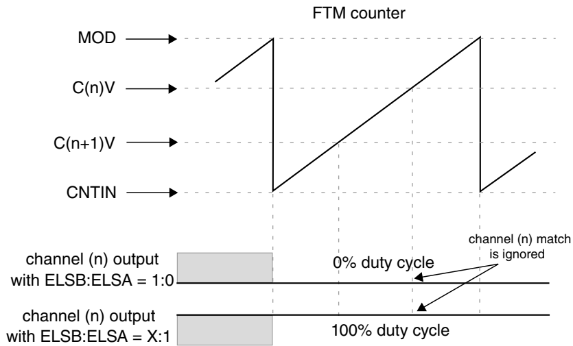
Figure 44-40. Channel (n) output if (CNTIN < C(n)V < MOD) and (CNTIN < C(n+1)V < MOD) and (C(n)V > C(n+1)V)
