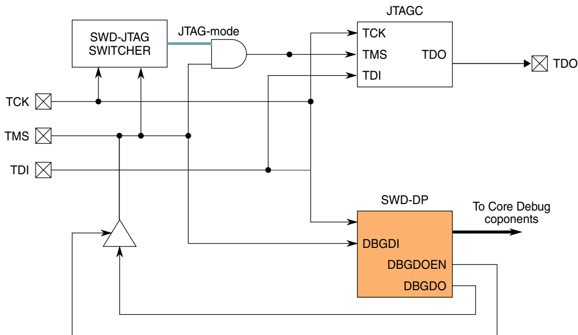
Figure 55-4. Modified debug port for CM0+ core
