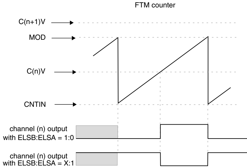
Figure 44-44. Channel (n) output if (C(n+1)V > MOD) and (CNTIN < C(n)V < MOD)
