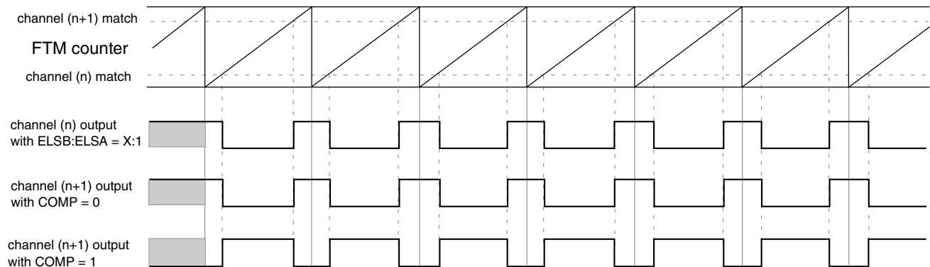
Figure 44-51. Channel (n+1) output in Complementary mode with (ELSB:ELSA = X:1)
