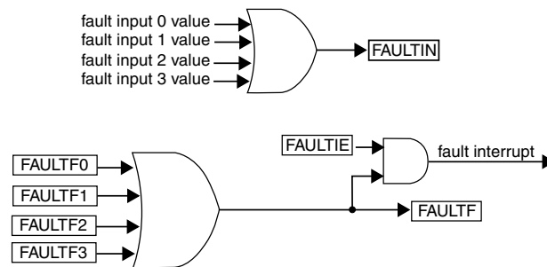
Figure 44-83. FAULTF and FAULTIN bits and fault interrupt
