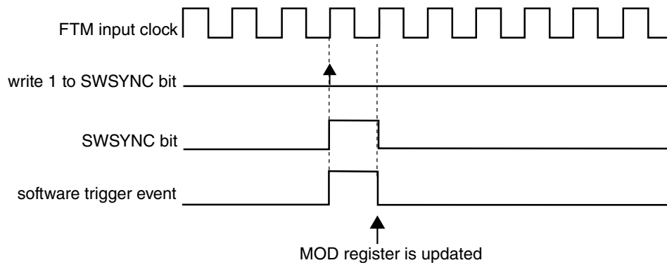
Figure 44-58. MOD synchronization with (SYNCMODE = 0), (PWMSYNC = 0), (REINIT = 1), and software trigger was used
