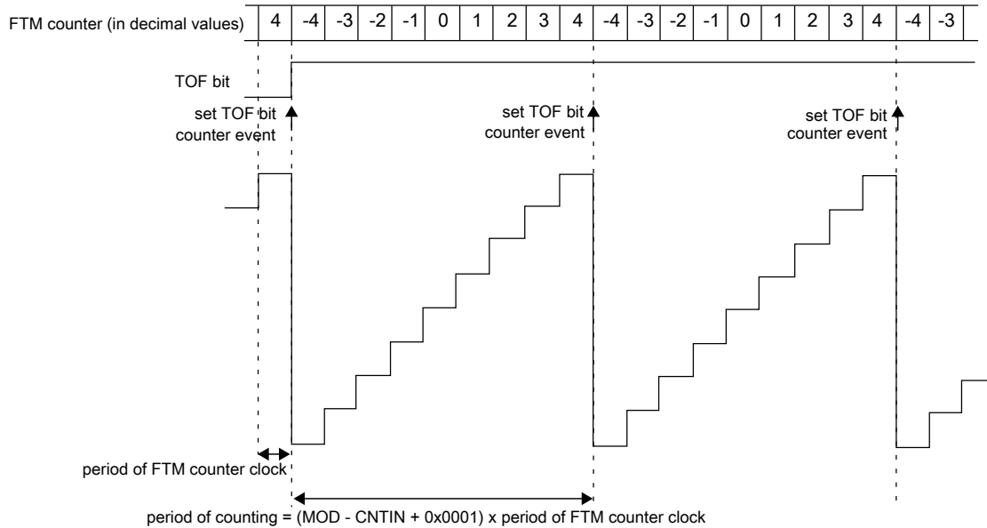
Figure 44-8. Example of FTM up and signed counting
