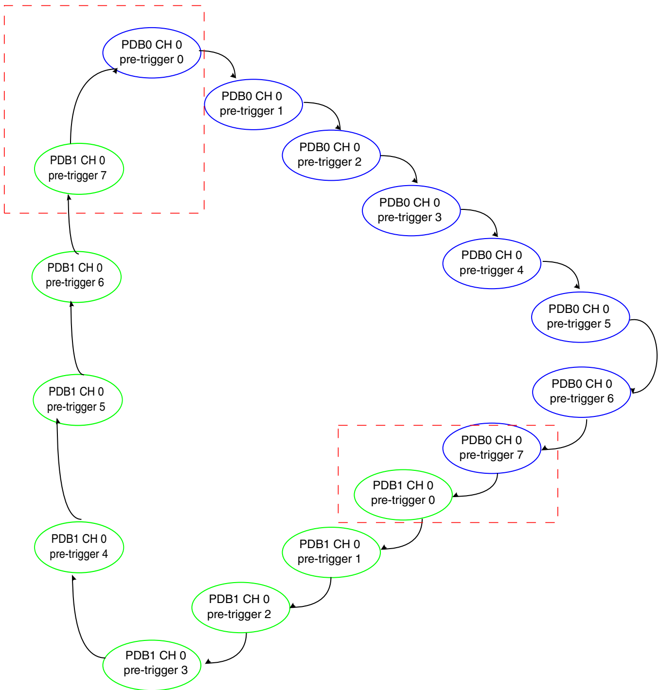
Figure 43-3. PDB back-to-back chain forming PDB0-PDB1 ring
