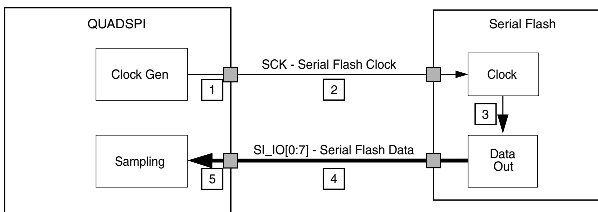
Figure 36-8. Serial Flash Sampling Clock Overview
