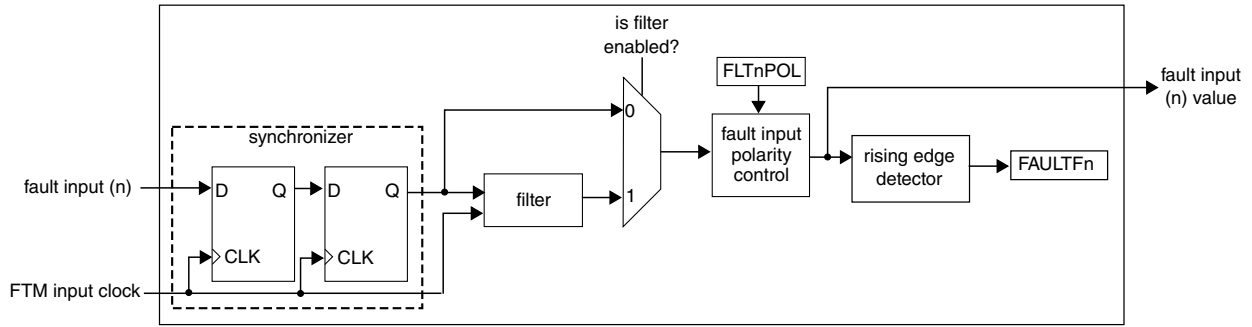
Figure 44-81. Diagram for Fault Control when FLTPS[3:0] = 0
