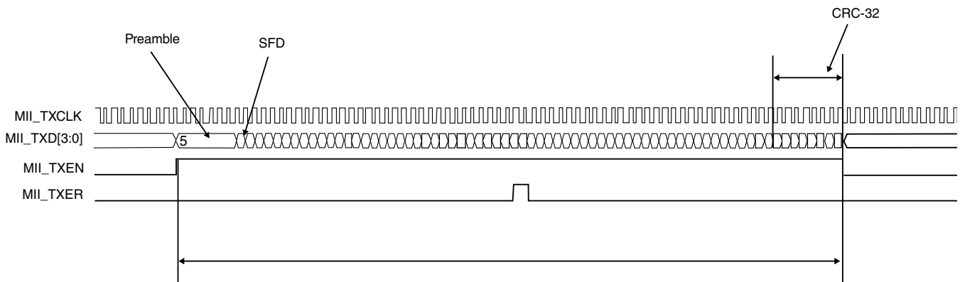
Figure 54-23. MII transmit operation — errored frame
