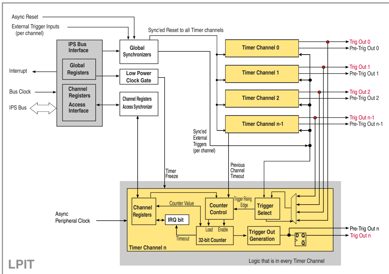
Figure 45-3. Detailed Block Diagram
