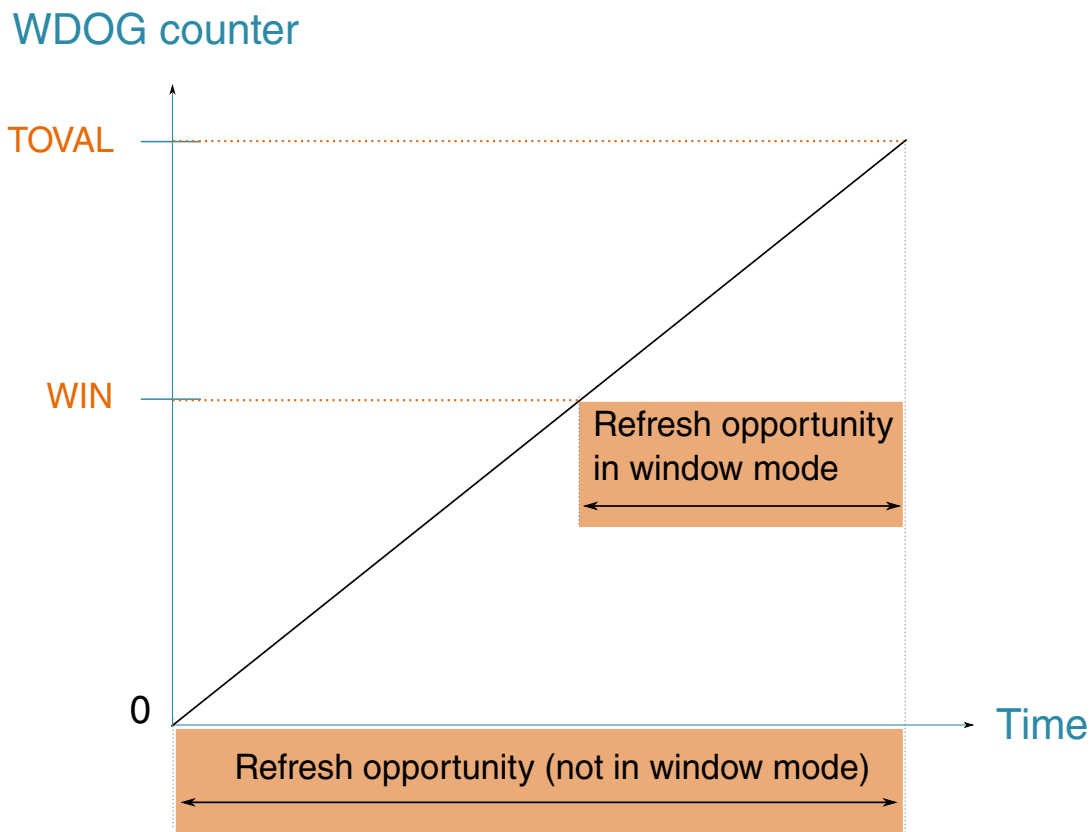
Figure 22-2. Refresh opportunity for the Watchdog counter
