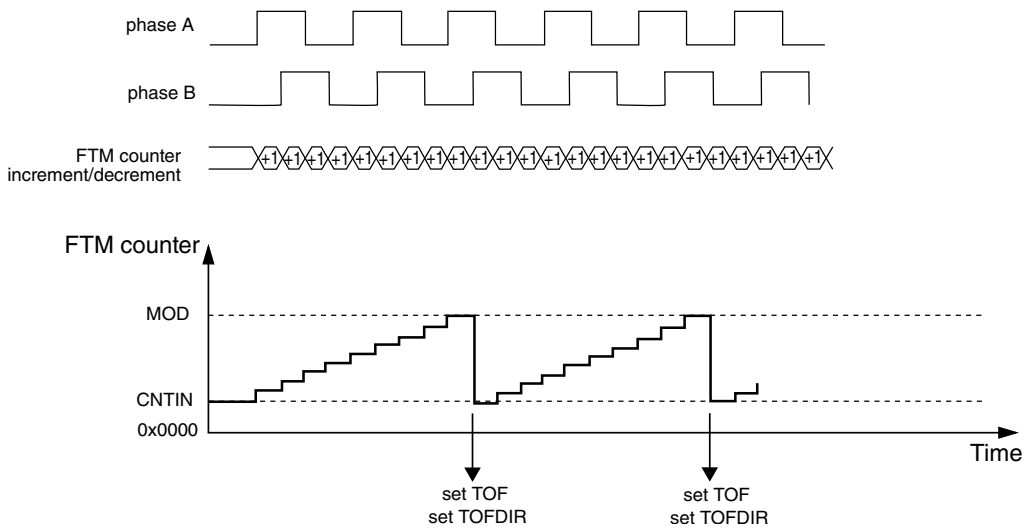
Figure 44-105. FTM Counter Overflow in Up Counting for Quadrature Decoder Mode
