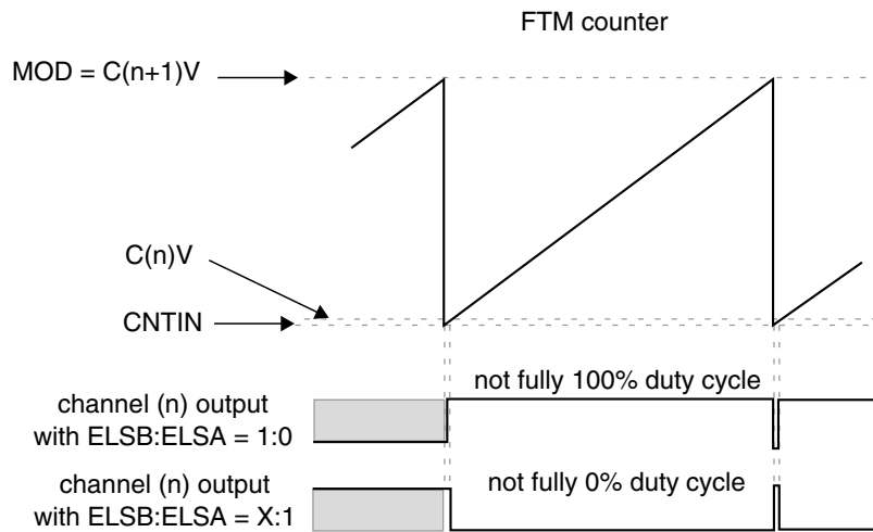
Figure 44-34. Channel (n) output if (CNTIN < C(n)V < MOD) and (C(n)V is Almost Equal to CNTIN ) and (C(n+1)V = MOD)
