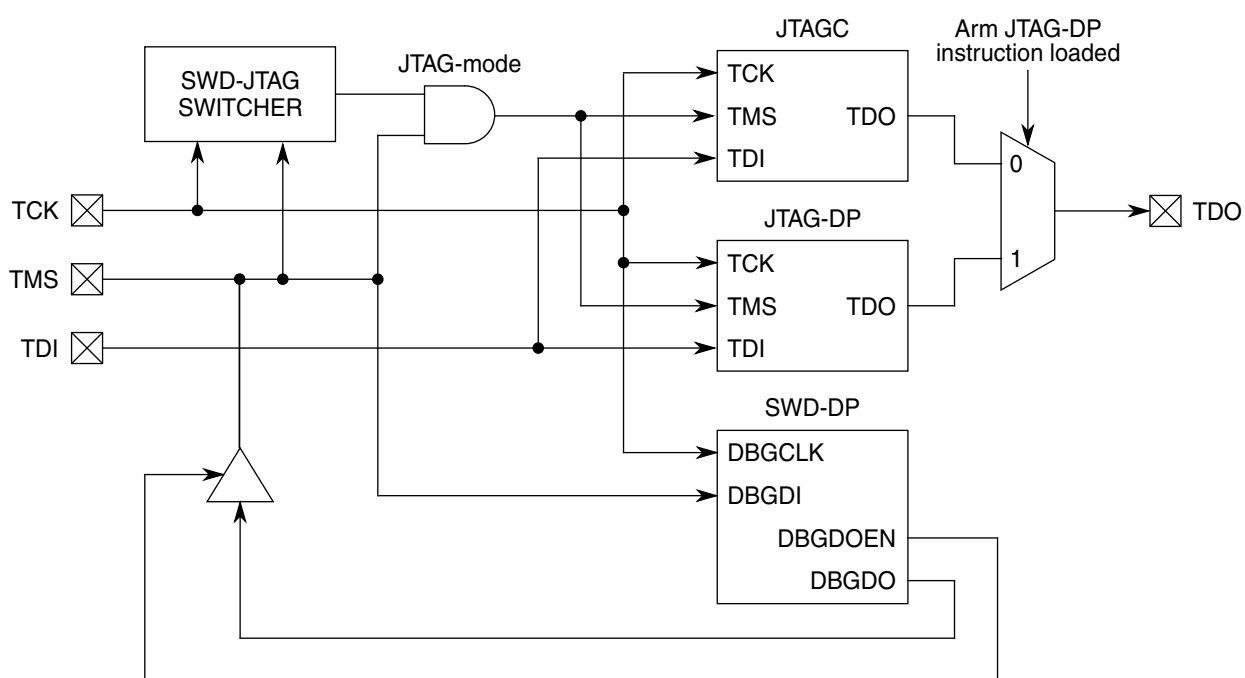
Figure 55-3. Modified debug port for CM4 core
