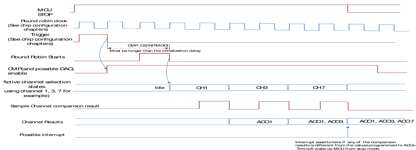
Figure 42-15. Trigger mode
