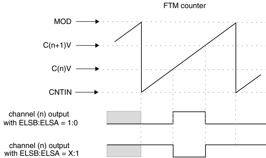
Figure 44-31. Channel (n) output if (CNTIN < C(n)V < MOD) and (CNTIN < C(n+1)V < MOD) and (C(n)V < C(n+1)V)
