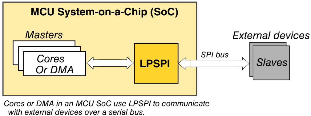
Figure 48-2. LPSPI connects masters in MCU to external slaves on PCB
