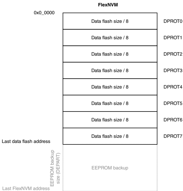
Figure 35-11. Data flash protection ( 2^n data flash sizes)
