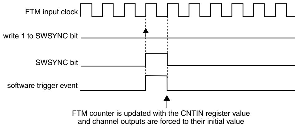
Figure 44-69. FTM counter synchronization with (SYNCMODE = 0), (REINIT = 1), (PWMSYNC = 0), and software trigger was used
