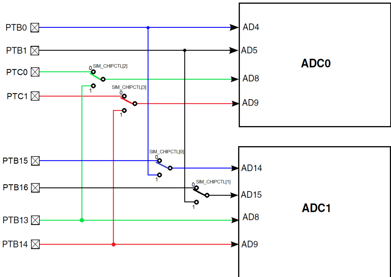
Figure 40-1. ADC0 and ADC1 hardware interleaved channels integration
