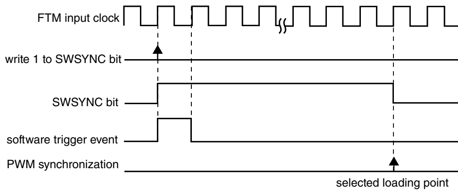
Figure 44-53. Software trigger event
