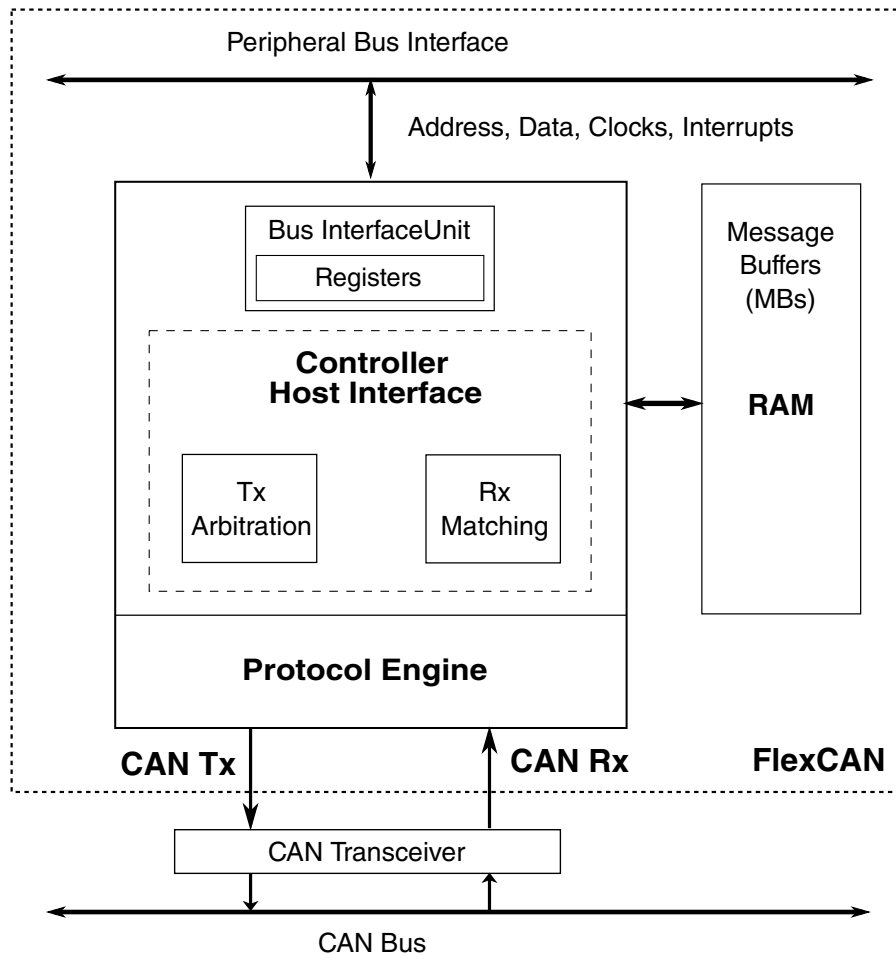
Figure 52-1. FlexCAN block diagram
