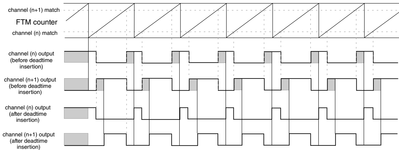
Figure 44-76. Deadtime insertion with ELSB:ELSA = X:1, POL(n) = 0, and POL(n+1) = 0
