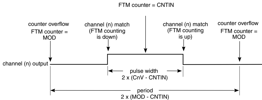
Figure 44-27. CPWM period and pulse width with ELSB:ELSA = 1:0
