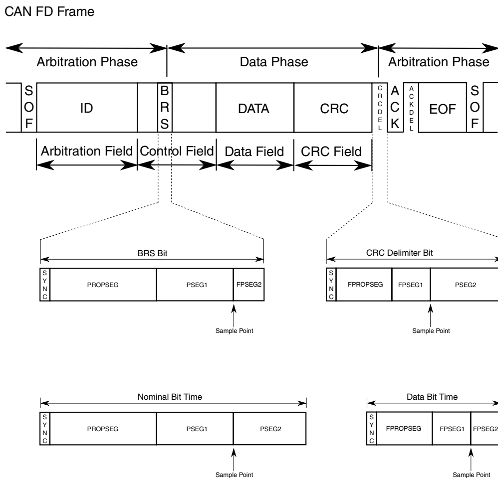
Figure 52-3. Bit rate switching mechanism for CAN FD messages
