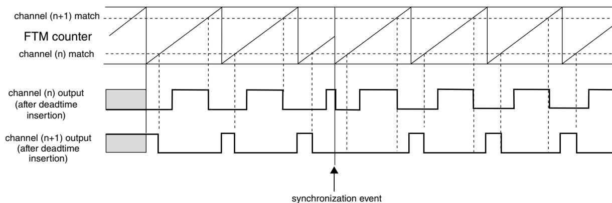
Figure 44-67. FTM counter synchronization
