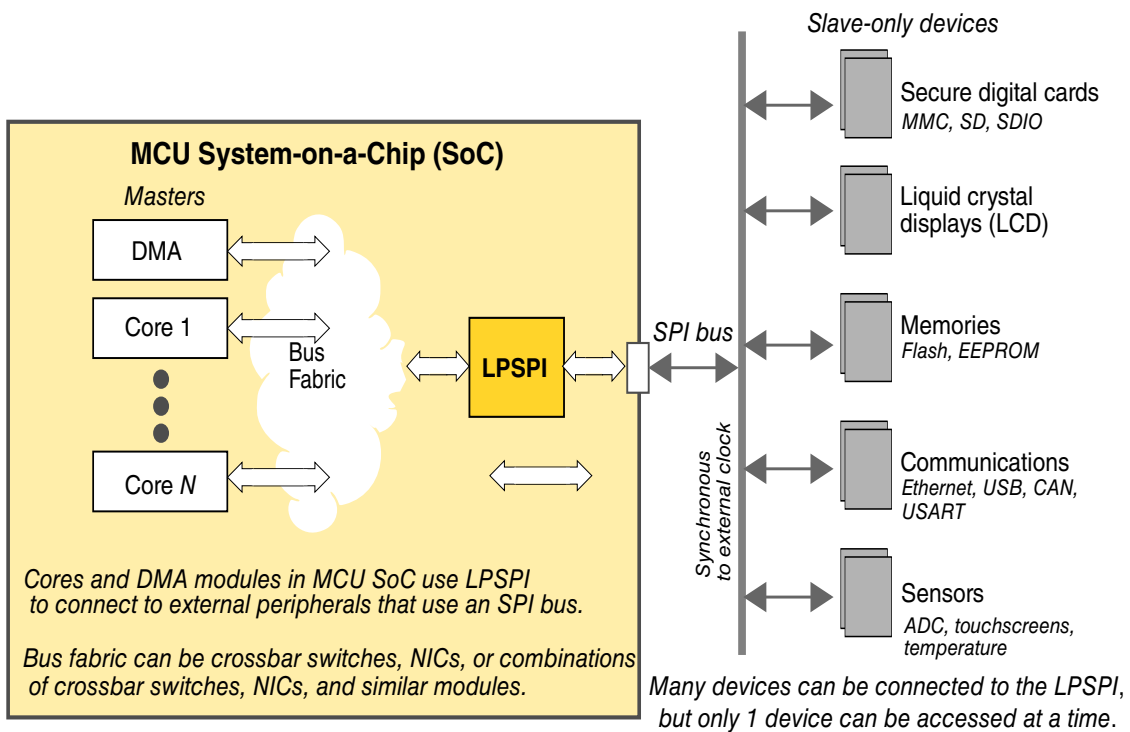
Figure 48-3. Typical LPSPI connection scheme
