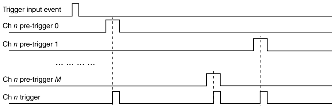
Figure 43-7. Pre-trigger and trigger outputs
