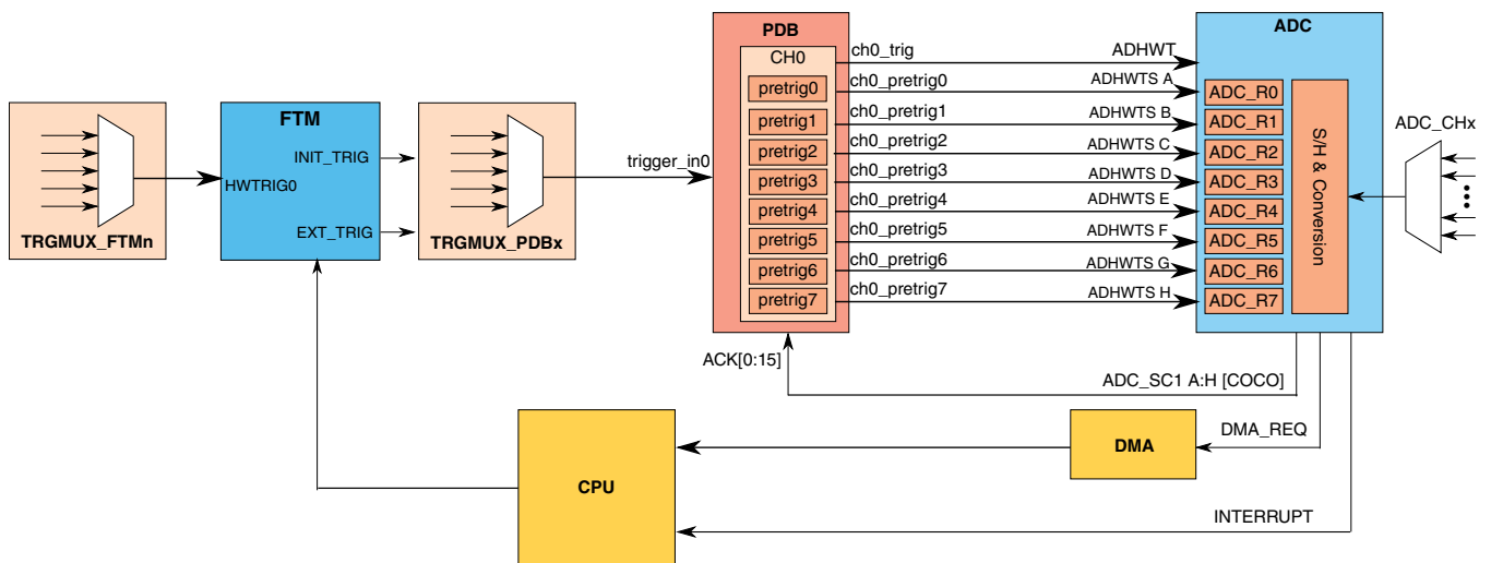
Figure 40-13. PWM Load Diagnosis – ADC Trigger Concept (block diagram)
