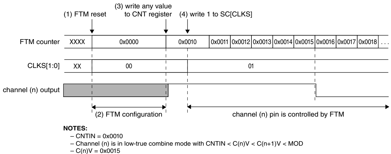
Figure 44-127. FTM behavior after reset when the channel (n) is in Combine mode
