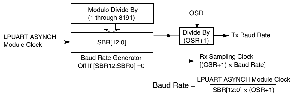
Figure 50-3. LPUART baud rate generation
