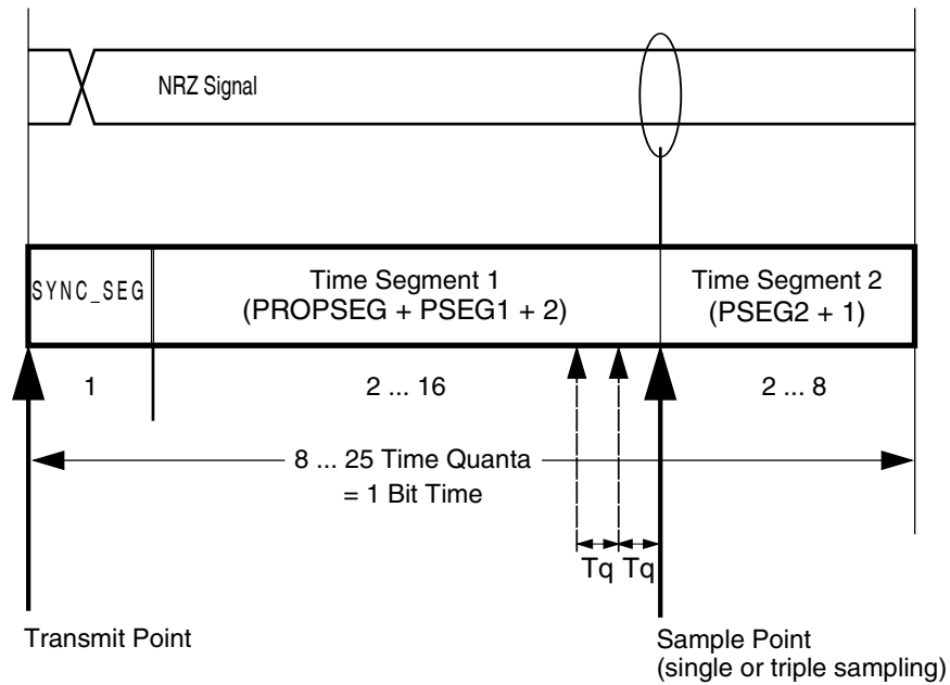
Figure 52-7. Segments within the bit time (example using CAN_CTRL1 bit timing variables for Classical CAN format)
