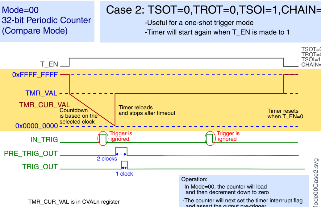
Figure 45-6. Case 2: TSOT = 0, TROT = 0, TSOI = 1, CHAIN = 0
