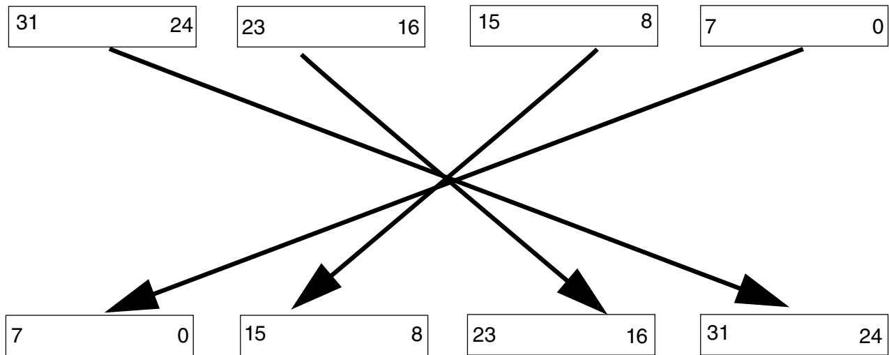
Figure 23-4. Transpose type 11
