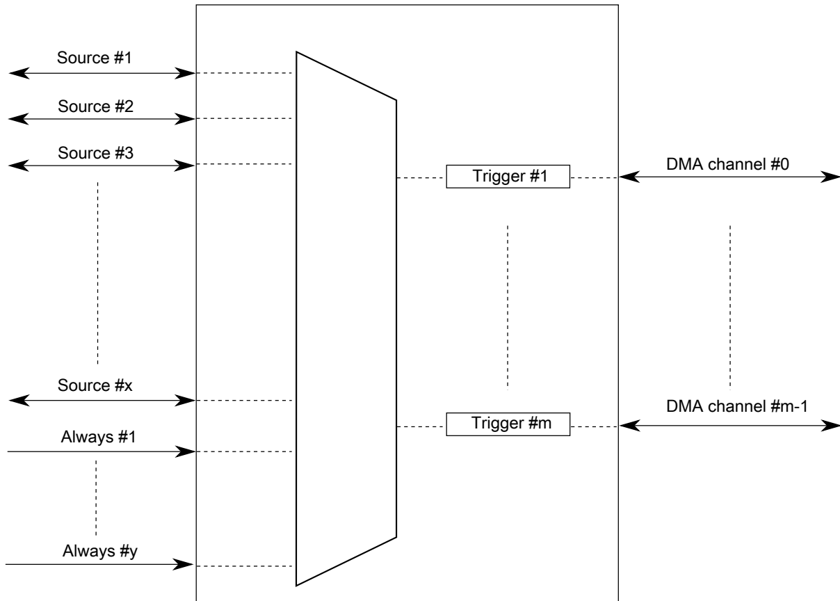
Figure 16-2. DMAMUX triggered channels
