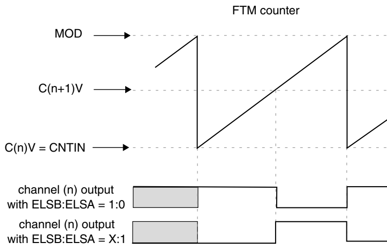
Figure 44-33. Channel (n) output if (C(n)V = CNTIN) and (CNTIN < C(n+1)V < MOD)
