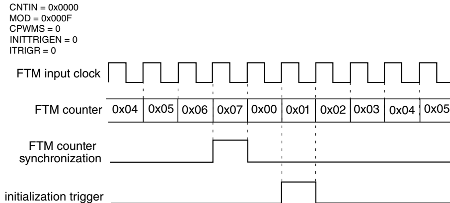
Figure 44-90. Example of the generation of the initialization trigger in the case 3.
