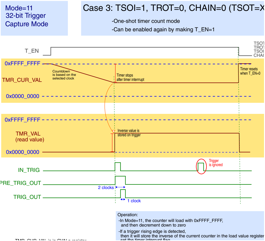
Figure 45-18. Case 3: TSOT = X, TROT = 0, TSOI = 1, CHAIN = 0
