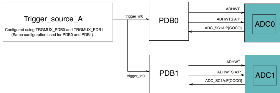
Figure 40-4. ADC triggering with same source
