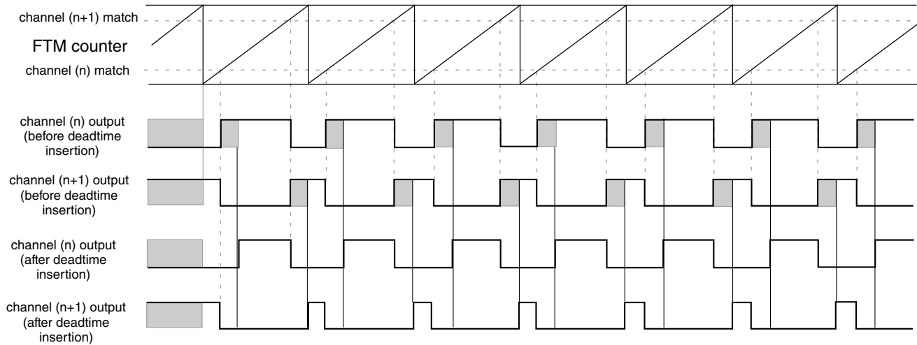
Figure 44-75. Deadtime insertion with ELSB:ELSA = 1:0, POL(n) = 0, and POL(n+1) = 0
