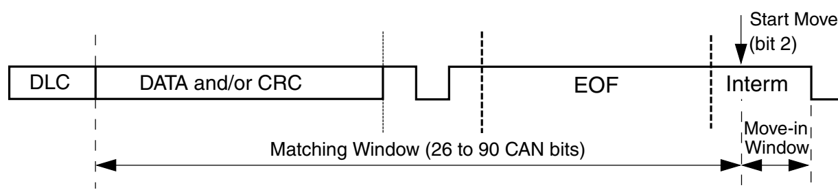
Figure 52-9. Matching and move-in time windows
