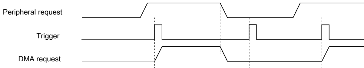
Figure 16-4. DMAMUX channel triggering: ignored trigger
