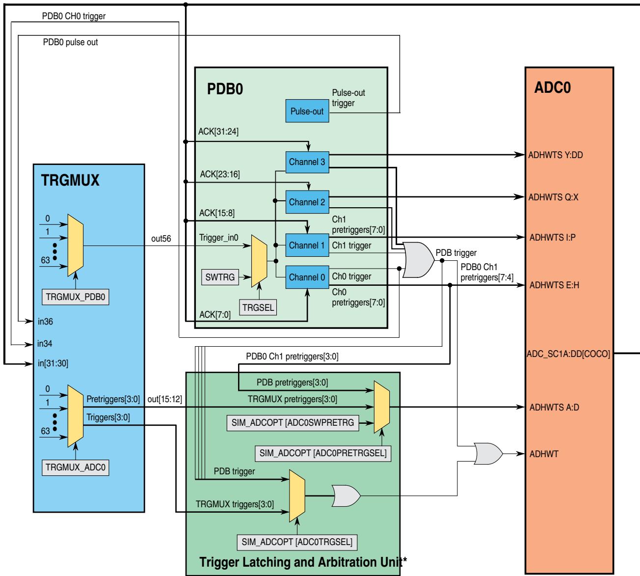
Figure 45-1. ADC triggering scheme
