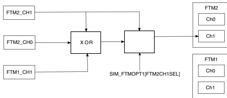
Figure 44-3. FTM Hall Sensor Configuration
