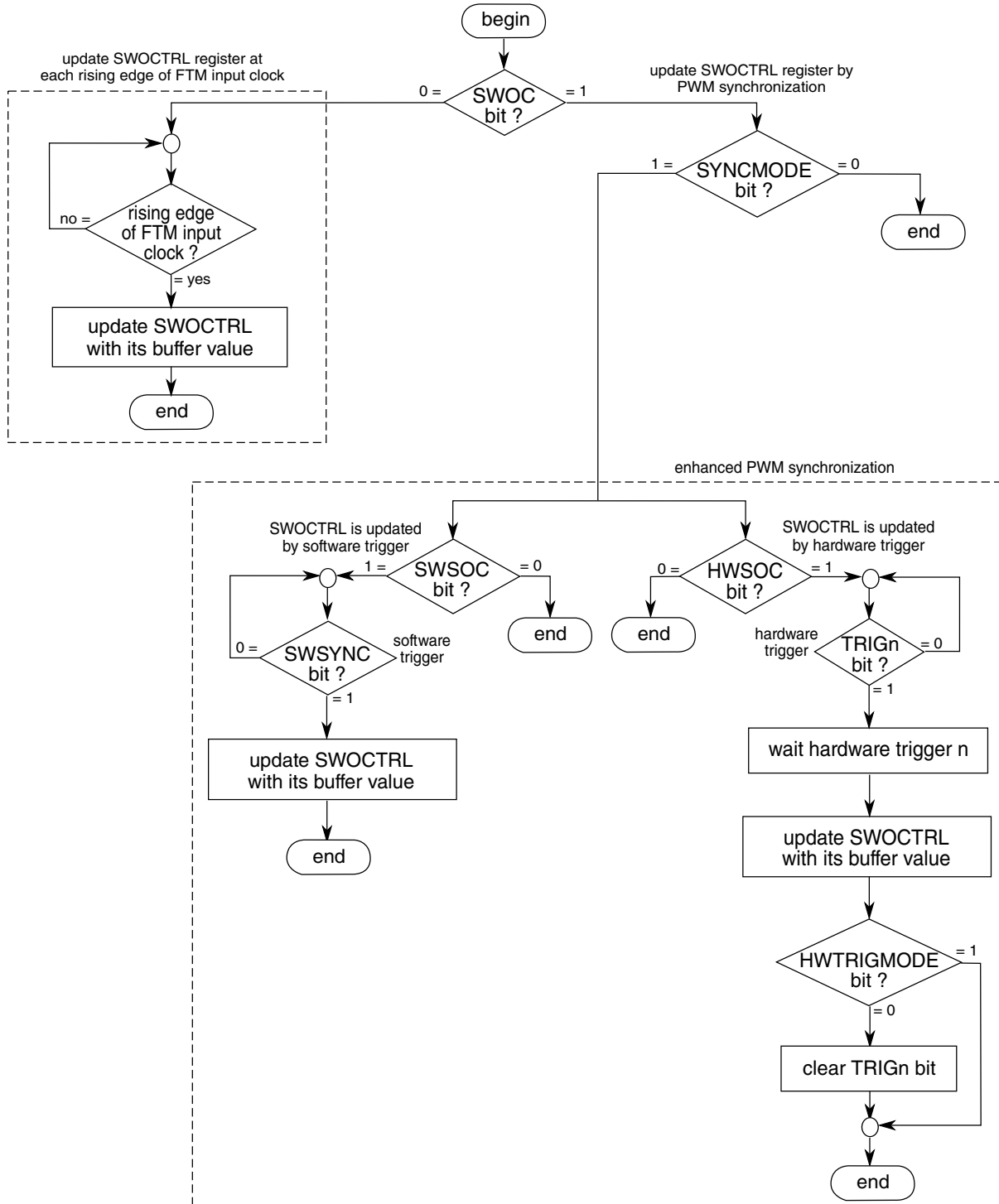
Figure 44-66. SWOCTRL register synchronization flowchart
