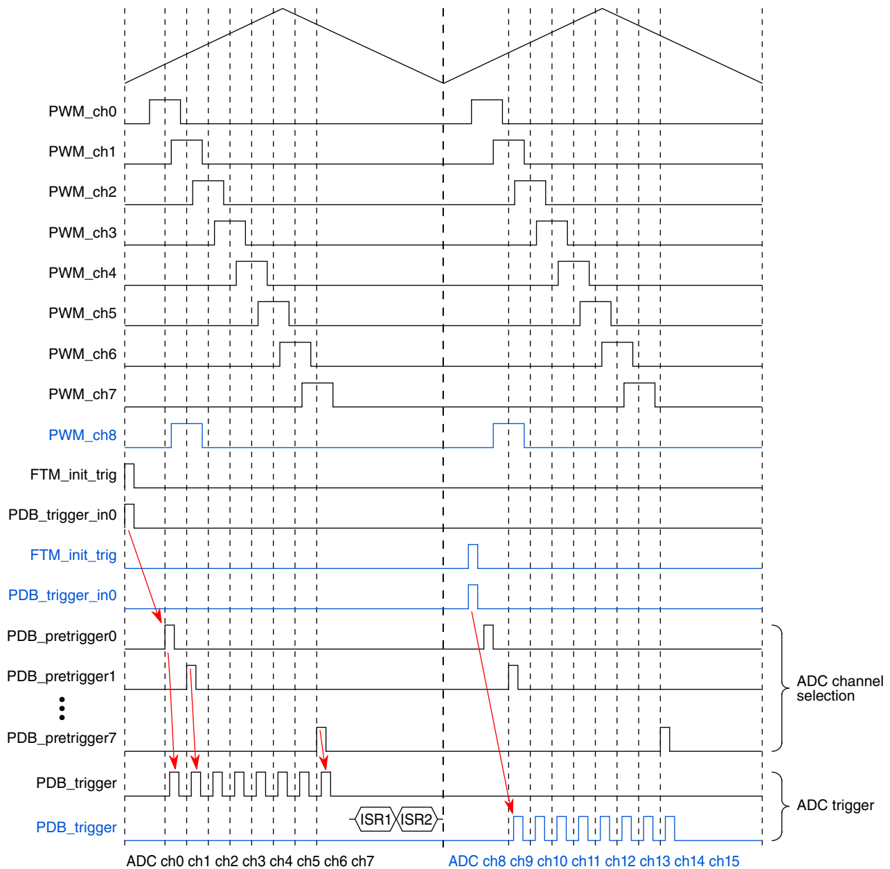
Figure 40-15. Example: PWM Load Diagnosis – ADC Trigger Concept 2 (Timing)
