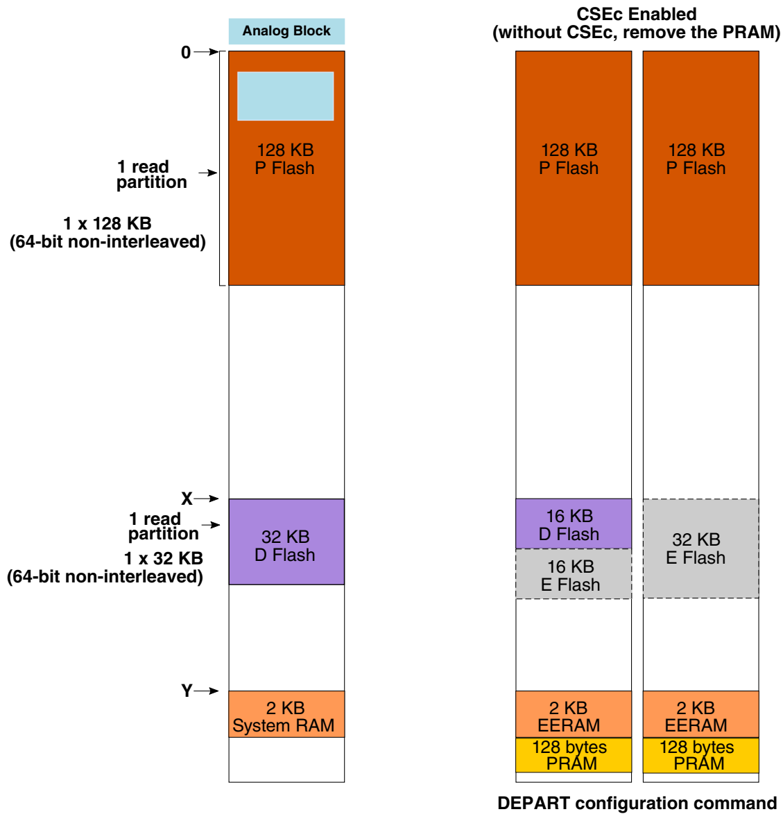
Figure 35-2. 128 KB flash memory map
