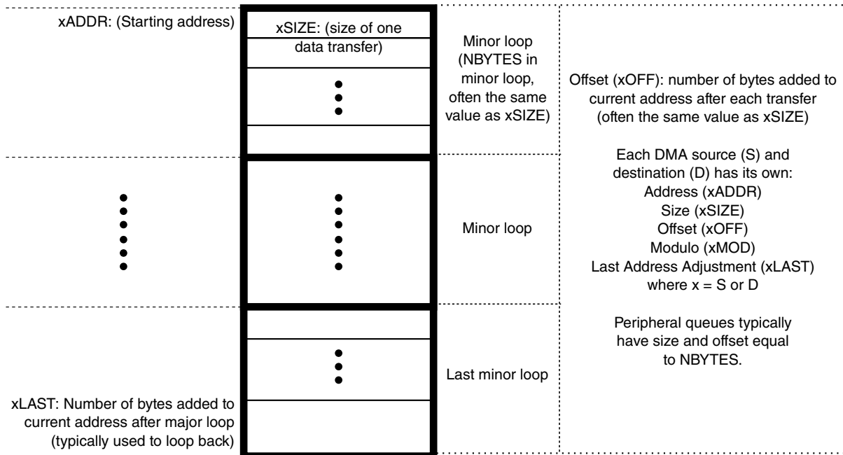
Figure 17-6. Memory array terms
