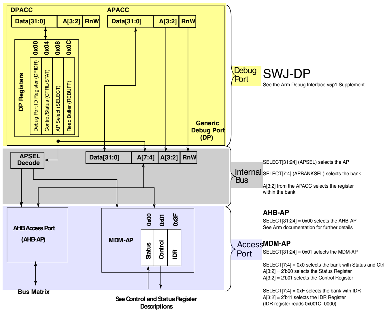
Figure 55-5. MDM AP addressing
