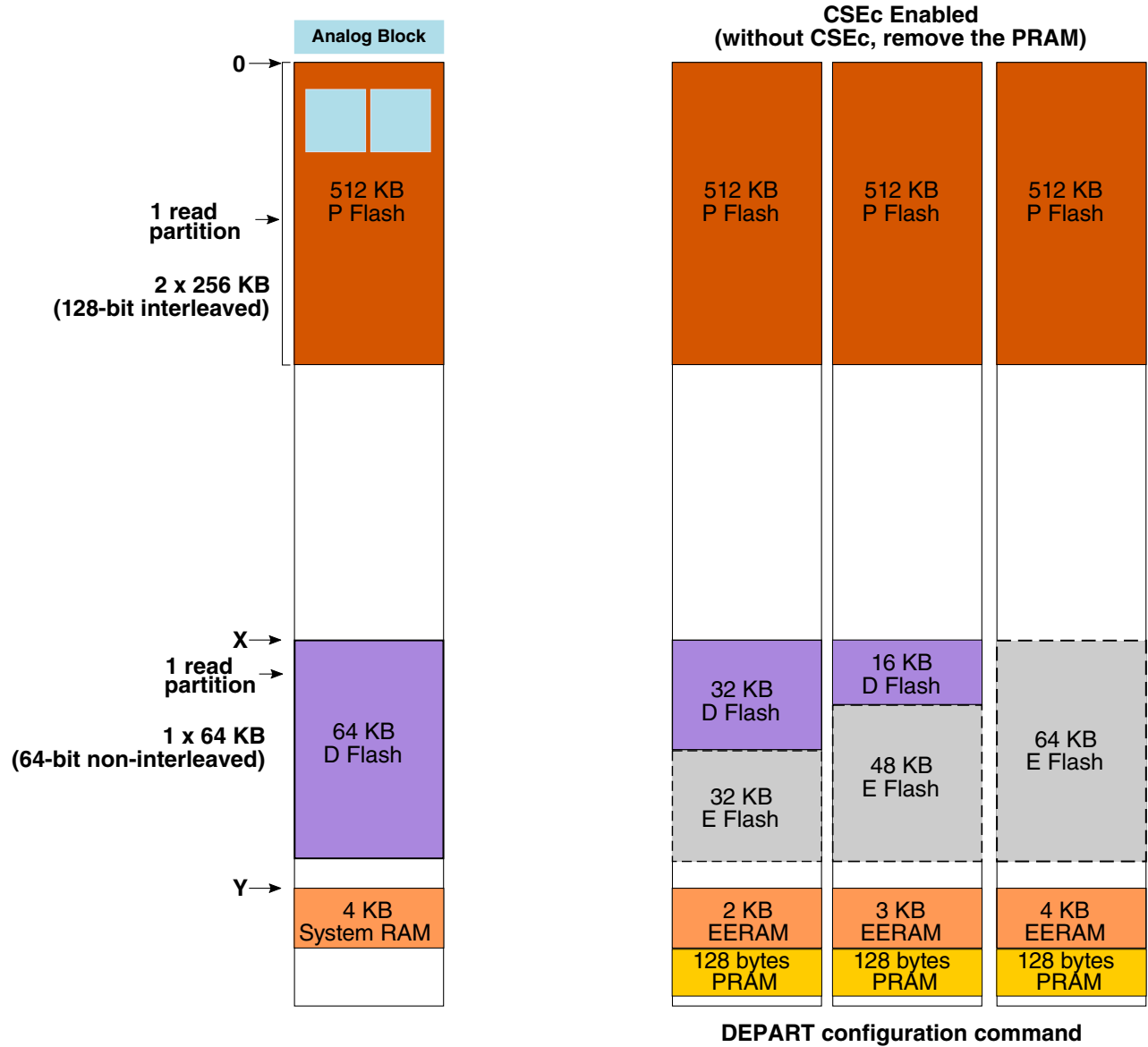
Figure 35-5. 512 KB flash memory map
