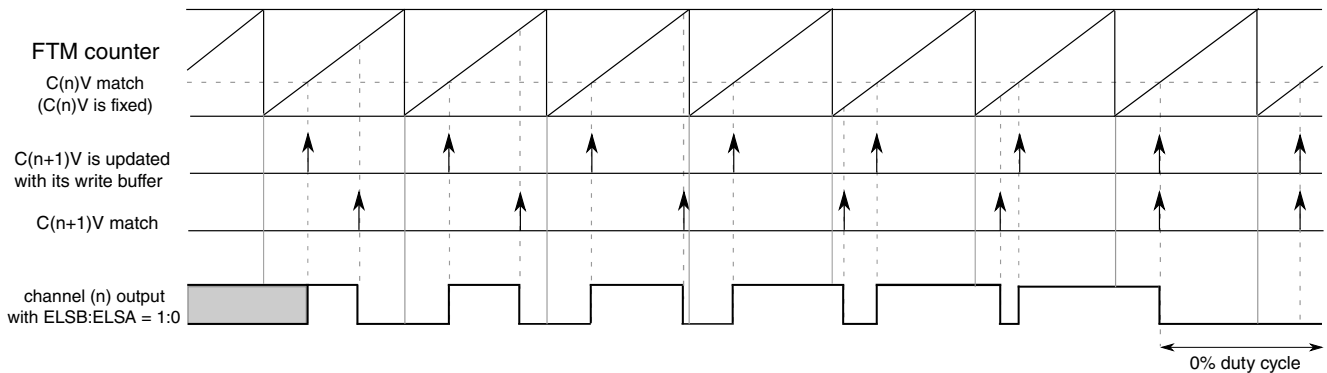
Figure 44-48. Modified Combine PWM Mode Examples
