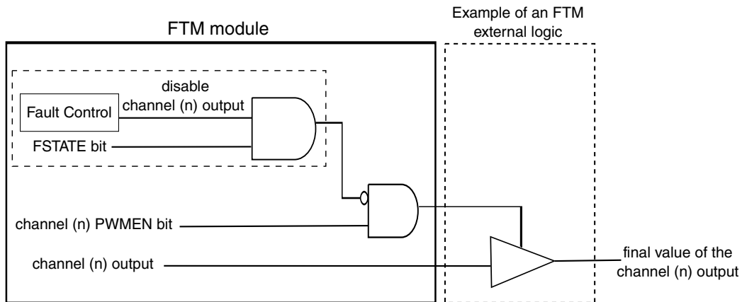
Figure 44-116. Example of the External Control of the Channel (n) Output
