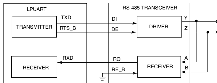
Figure 50-4. Transceiver driver enable using RTS_B
