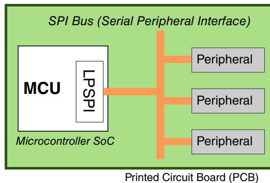
Figure 48-1. SPI bus connects MCU to peripherals on PCB
