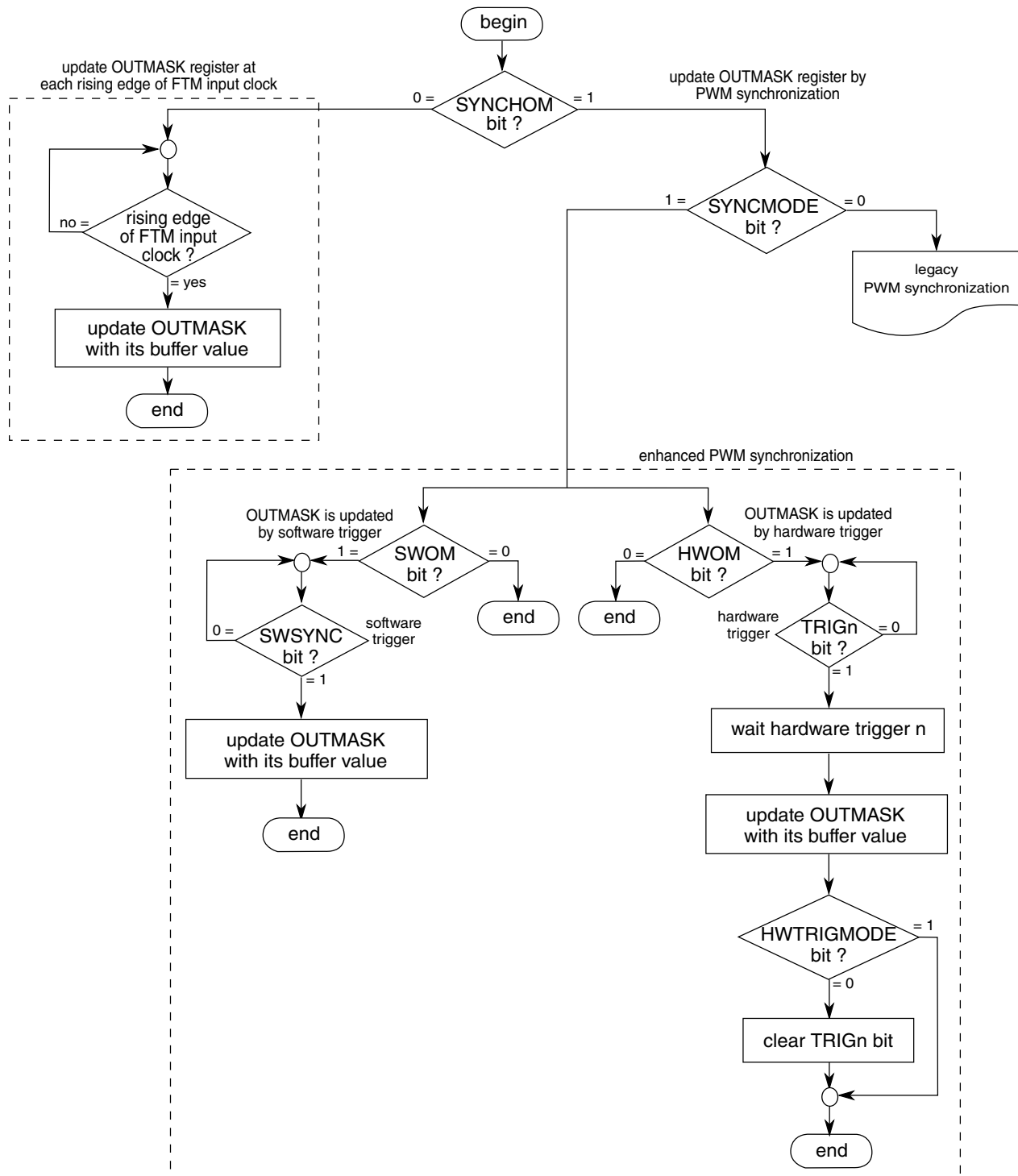
Figure 44-61. OUTMASK register synchronization flowchart
