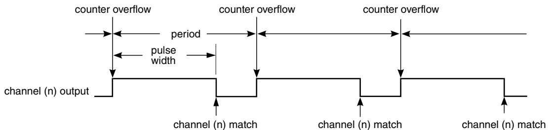
Figure 44-24. EPWM period and pulse width with ELSB:ELSA = 1:0
