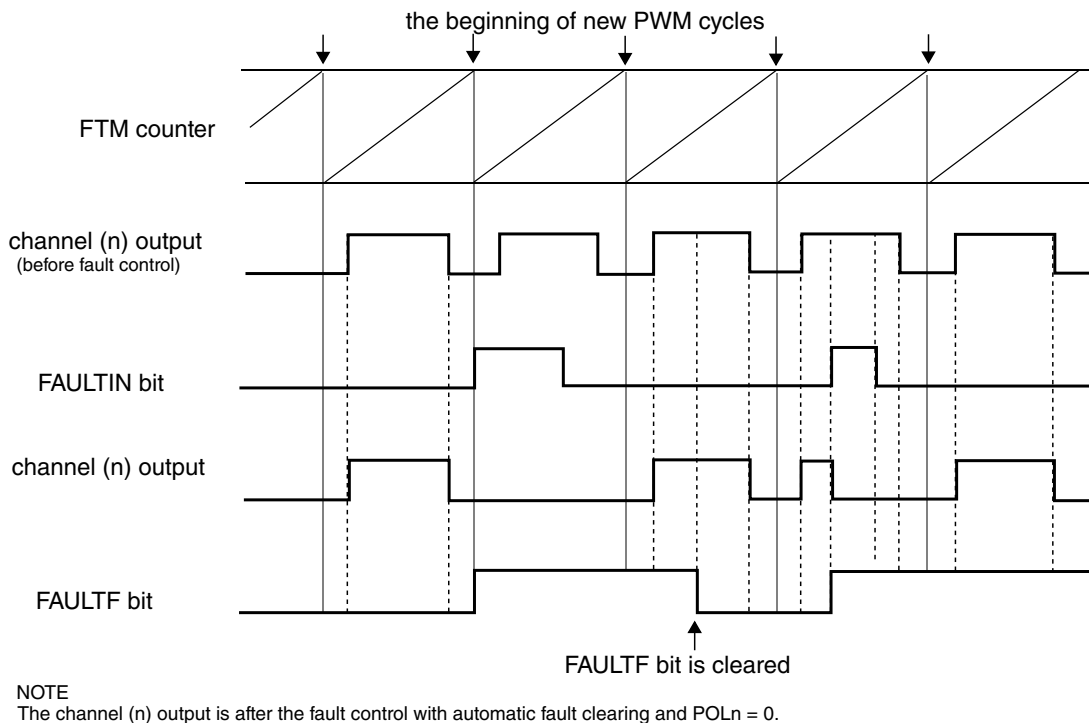
Figure 44-84. Fault control with automatic fault clearing
