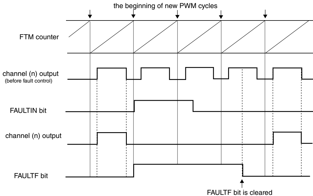
Figure 44-85. Fault control with manual fault clearing
