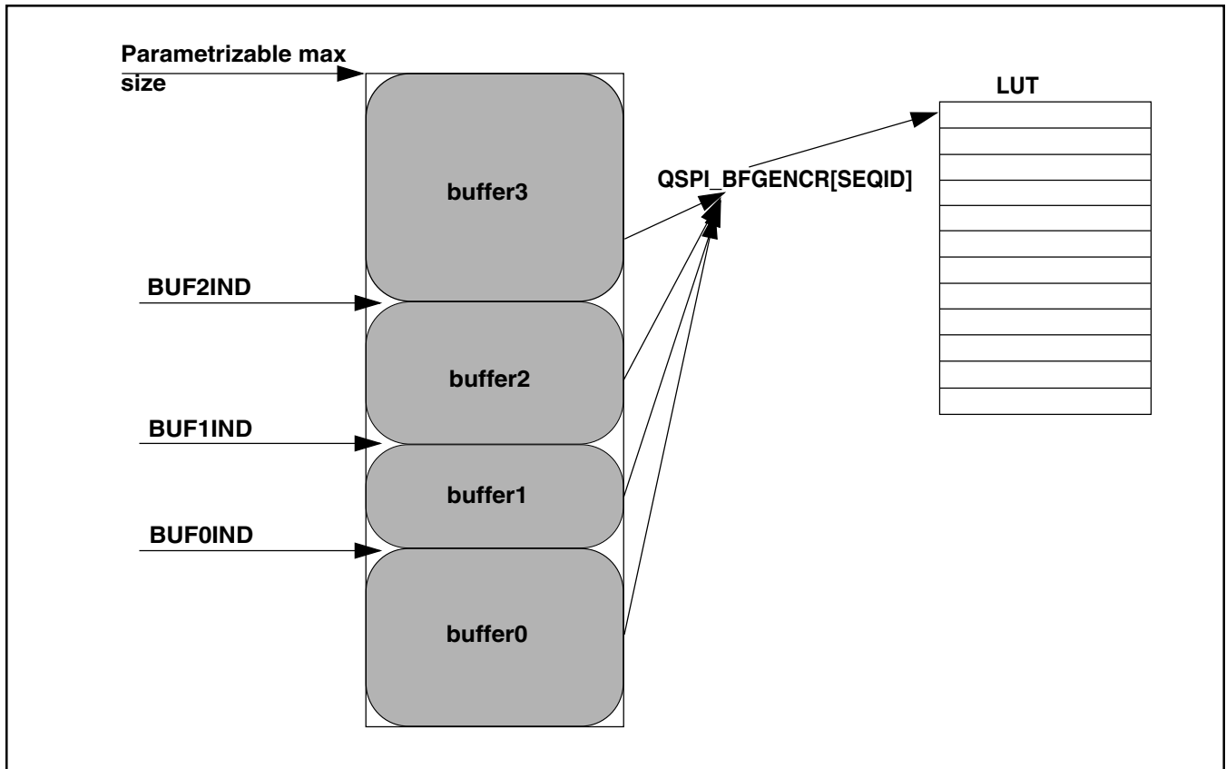
Figure 36-4. Flexible AHB Buffers
