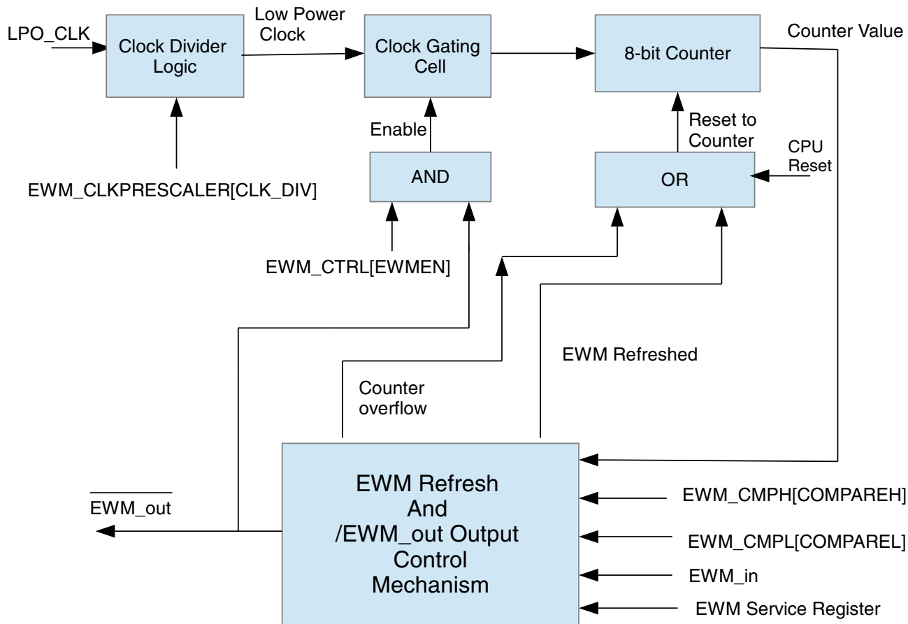
Figure 19-1. EWM Block Diagram
