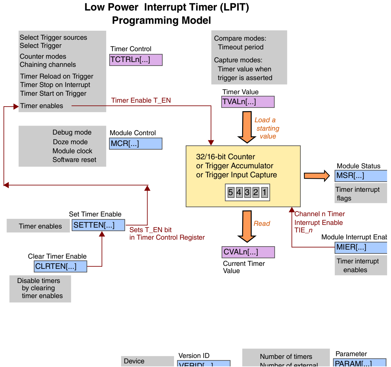
Figure 45-4. Programming Model
