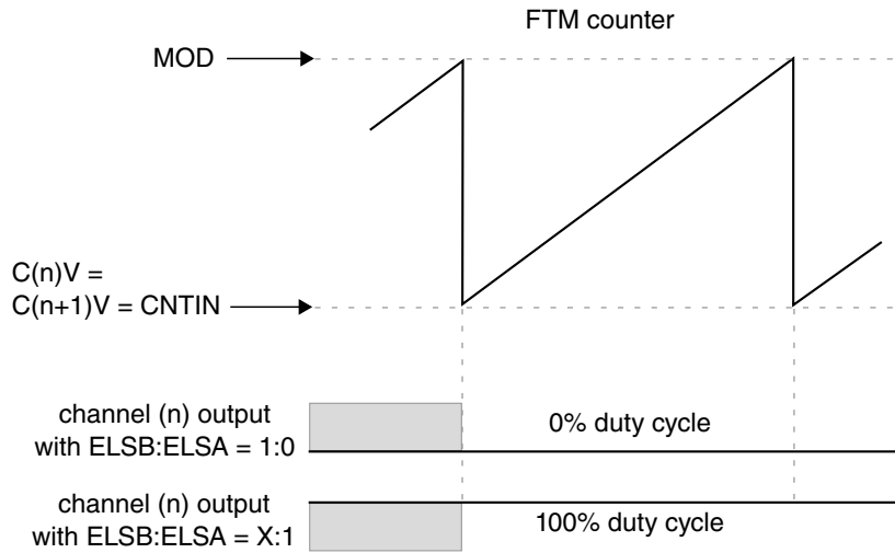
Figure 44-38. Channel (n) output if (C(n)V = C(n+1)V = CNTIN)
