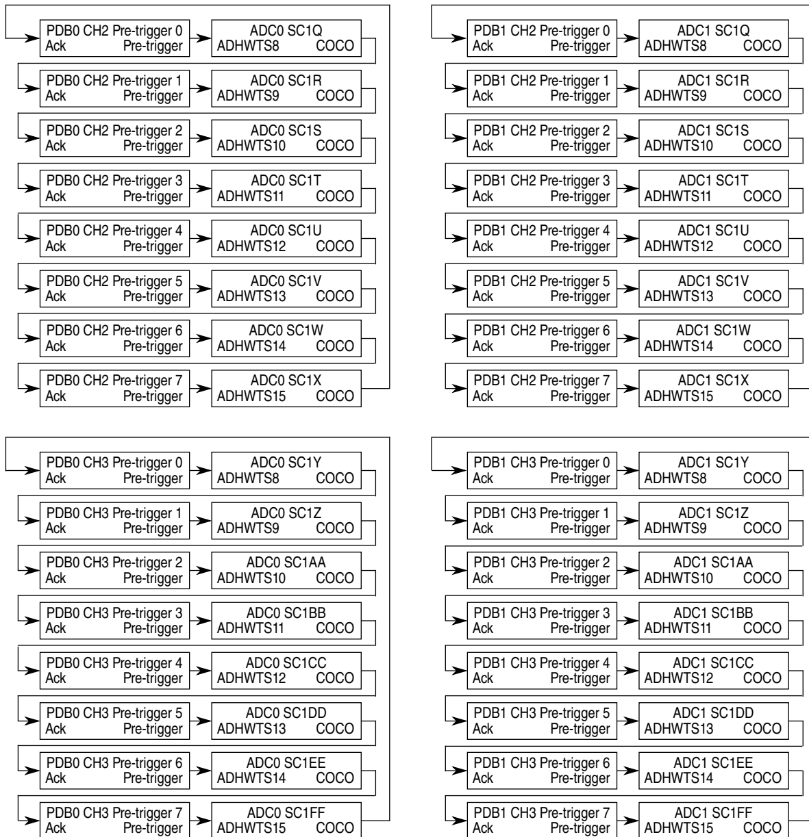
Figure 43-5. PDB-ADC back to back connection (Part 2 of 2)
