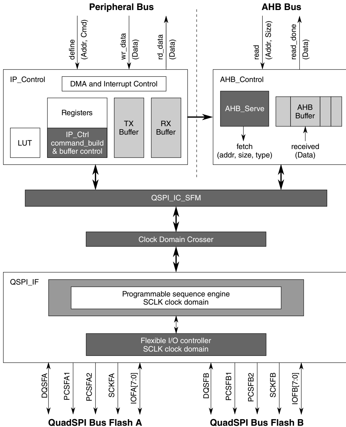
Figure 36-2. QuadSPI Block Diagram
