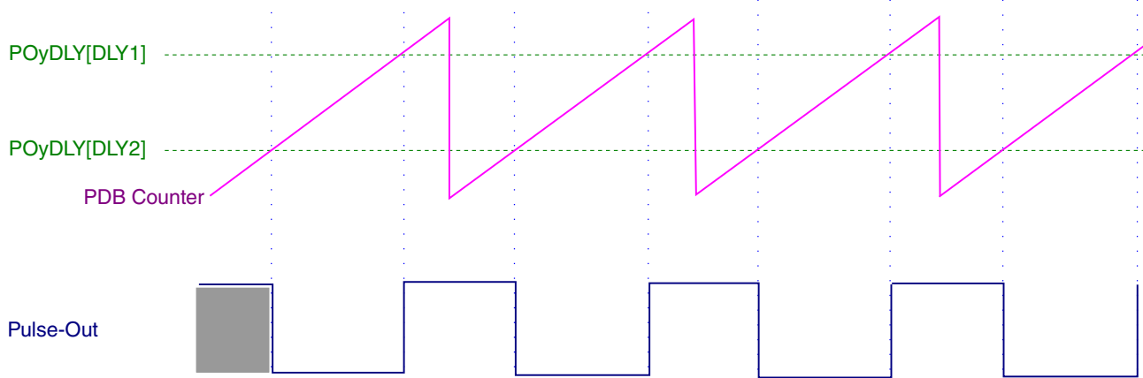
Figure 43-8. How Pulse Out is generated
