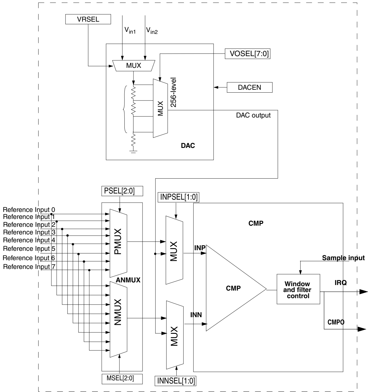
Figure 42-1. CMP high level diagram
