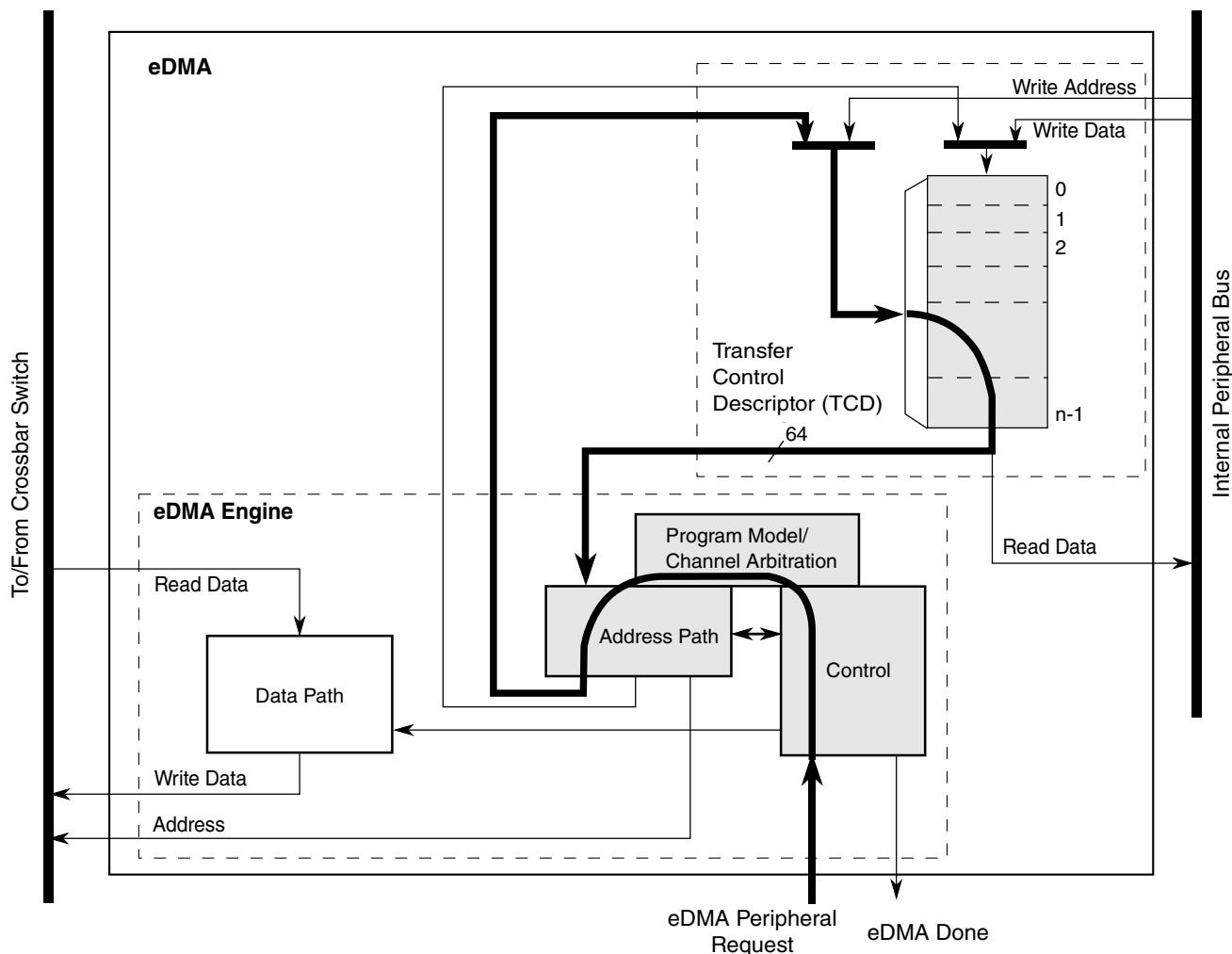
Figure 17-2. eDMA operation, part 1
