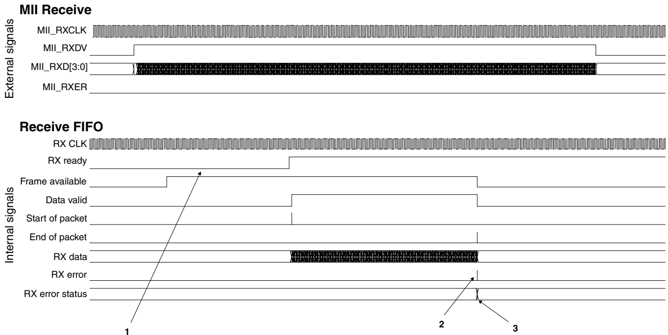
Figure 54-17. Receive FIFO overflow protection
