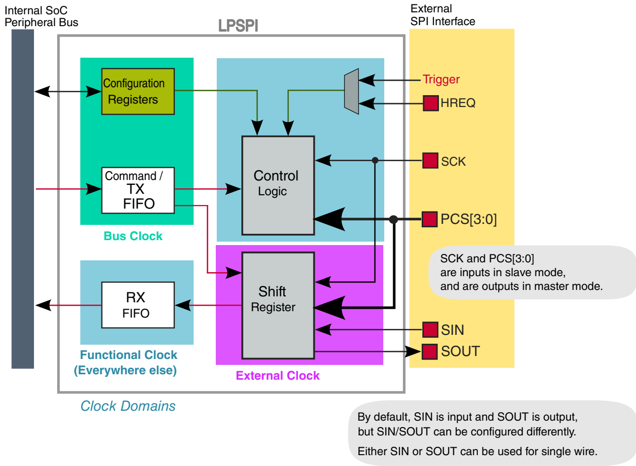
Figure 48-4. Block Diagram
