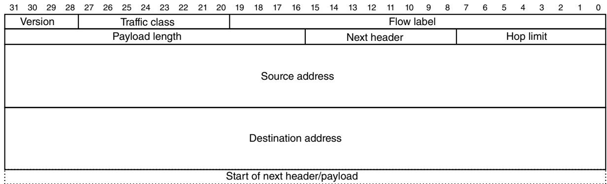
Figure 54-4. IPv6 header format
