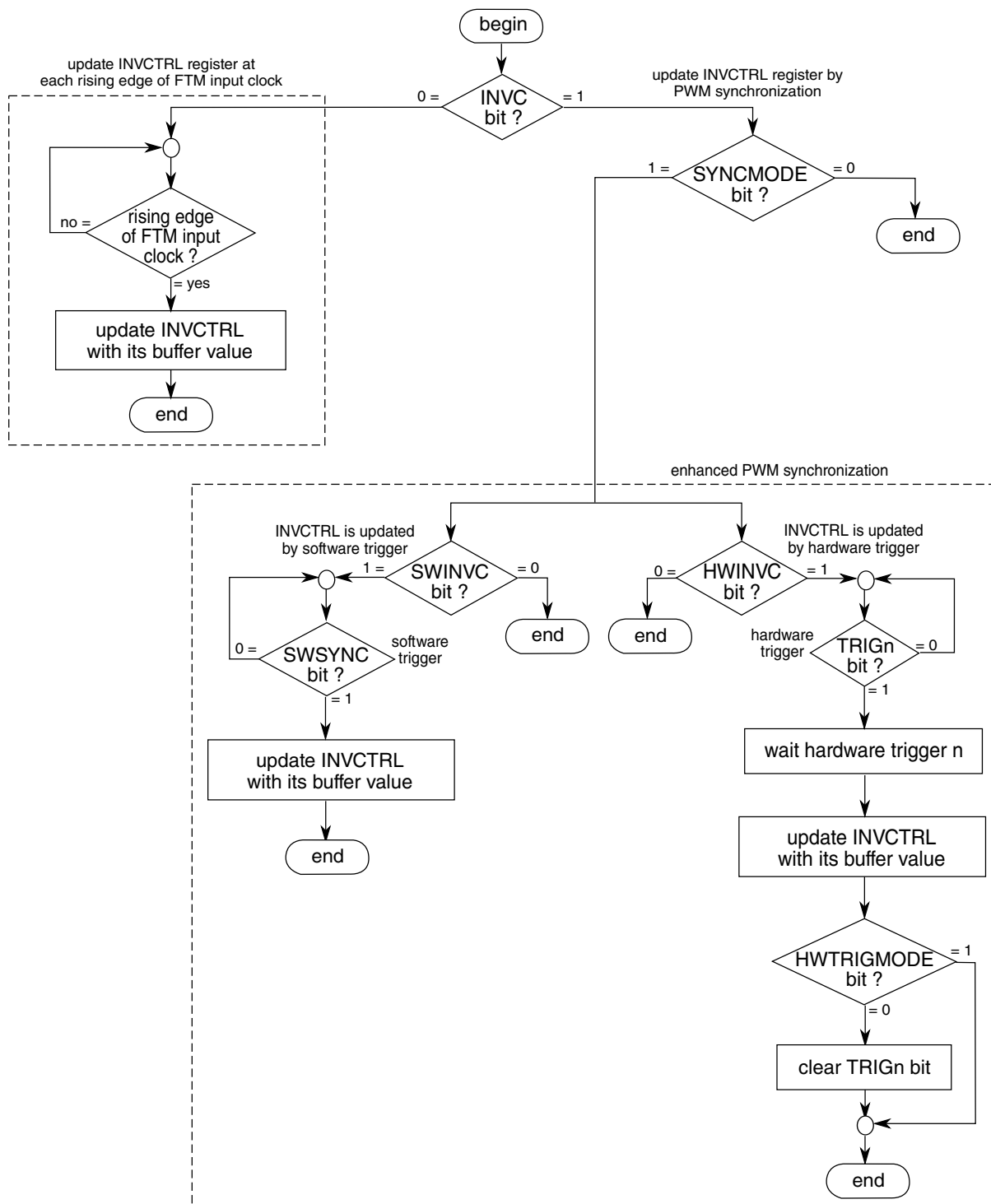
Figure 44-65. INVCTRL register synchronization flowchart
