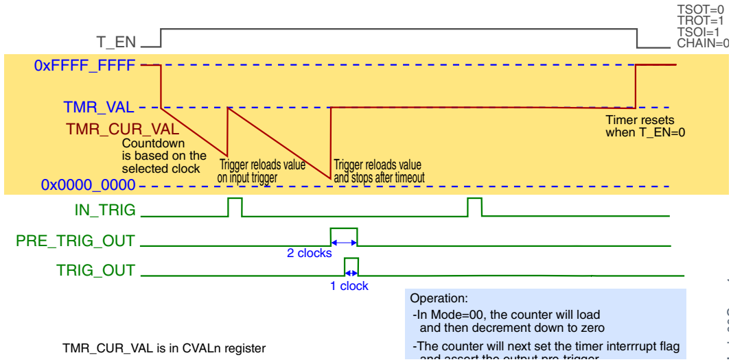
Figure 45-8. Case 4: TSOT = 0, TROT = 1, TSOI = 1, CHAIN = 0
