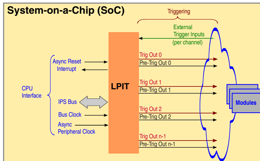
Figure 45-2. LPIT Interface in SoC
