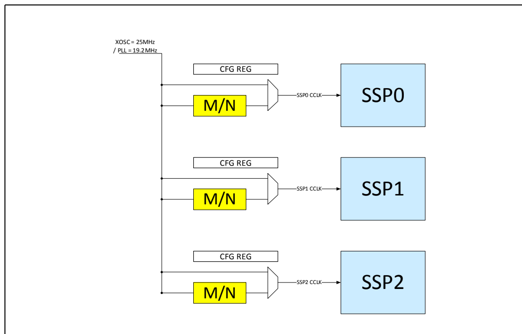
Figure 110.SSP CCLK Structure
