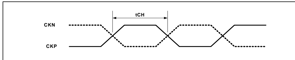
Figure 32. DDR3L CK Low Time
