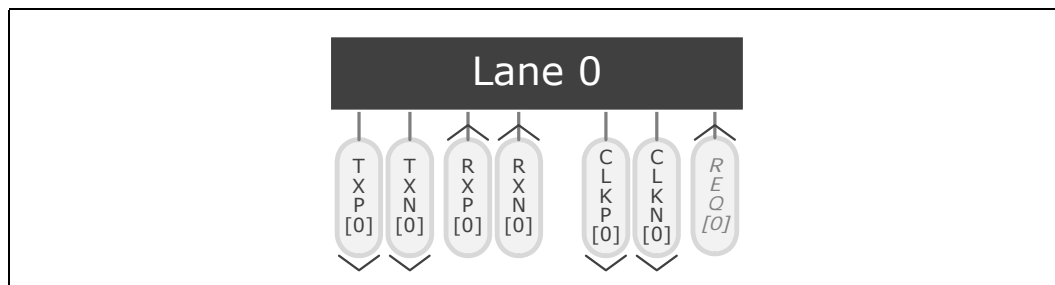
Figure 114. PCIe* 2.0 Lane 0 Signal Example
