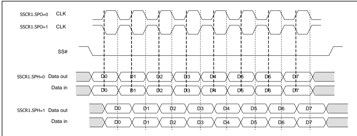
Figure 118. Clock Phase and Polarity
