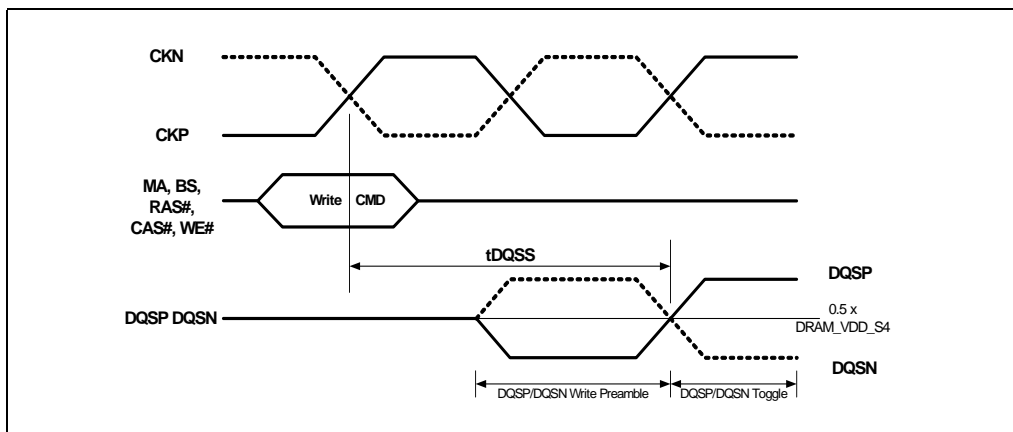
Figure 35. DDR3L CK Rising Edge Output Access Time to the 1st DQS Rising Edge
