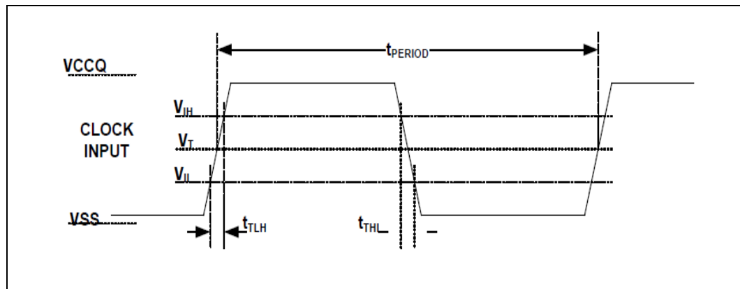
Figure 54. eMMC Clock Signal Timing Diagram (HS200 Mode)
