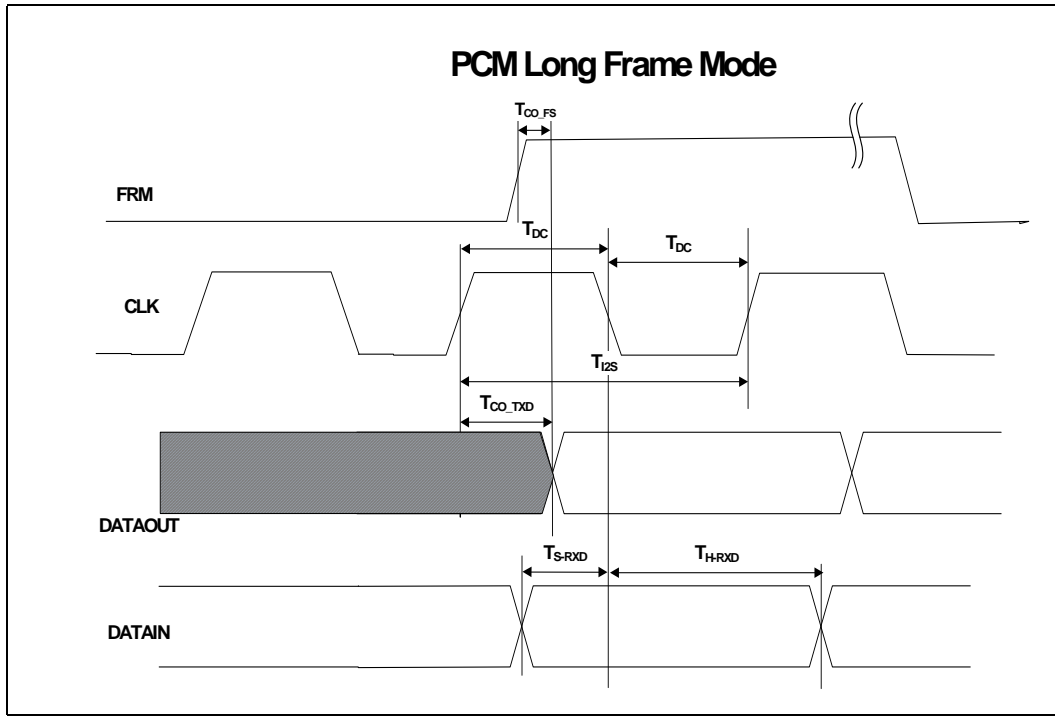
Figure 66. I 2 S Slave Port Timings in PCM Long Frame Mode
