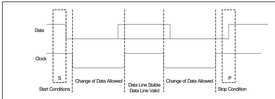
Figure 121. START and STOP Conditions
