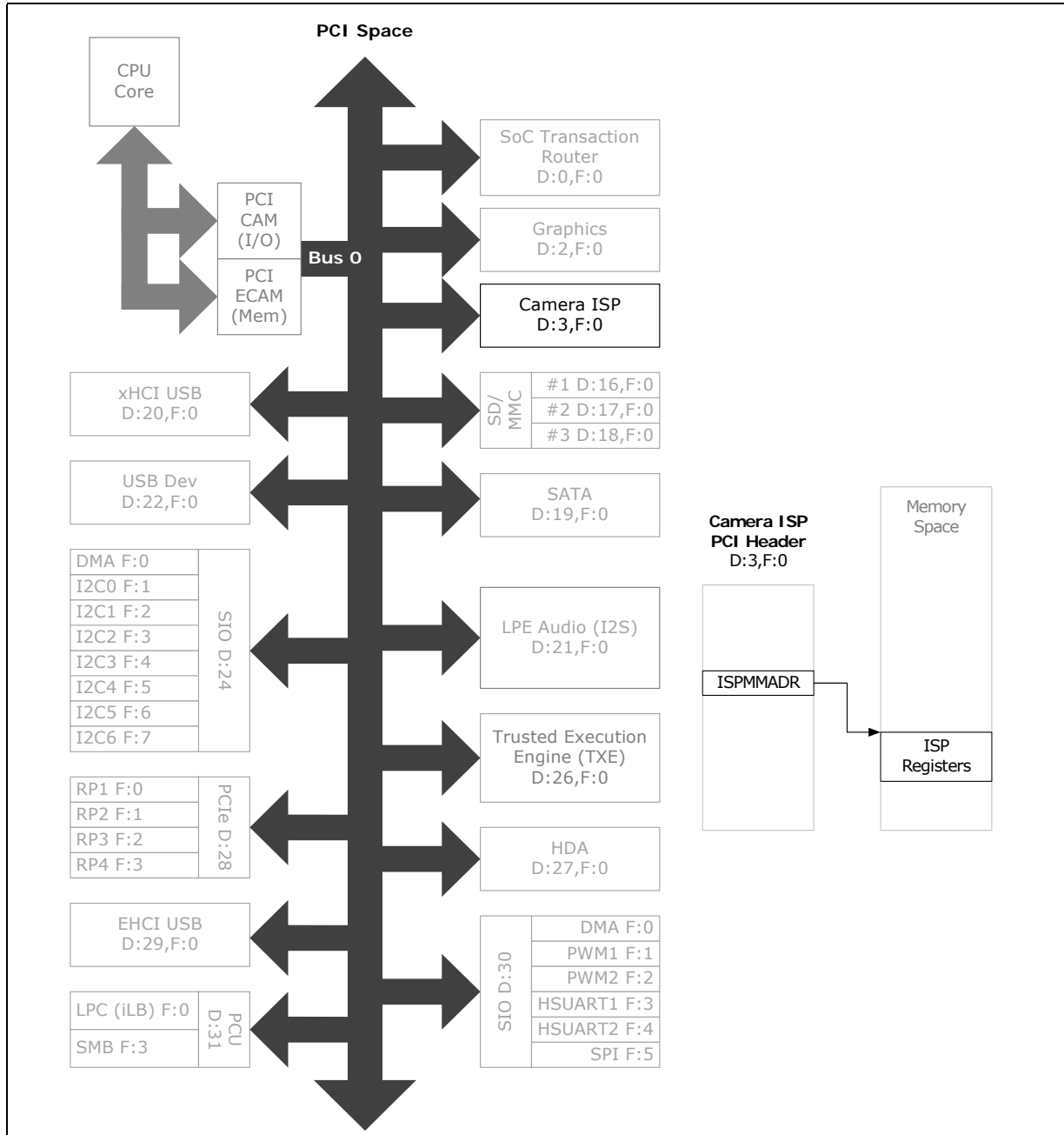
Figure 99. MIPI CSI Register Map
