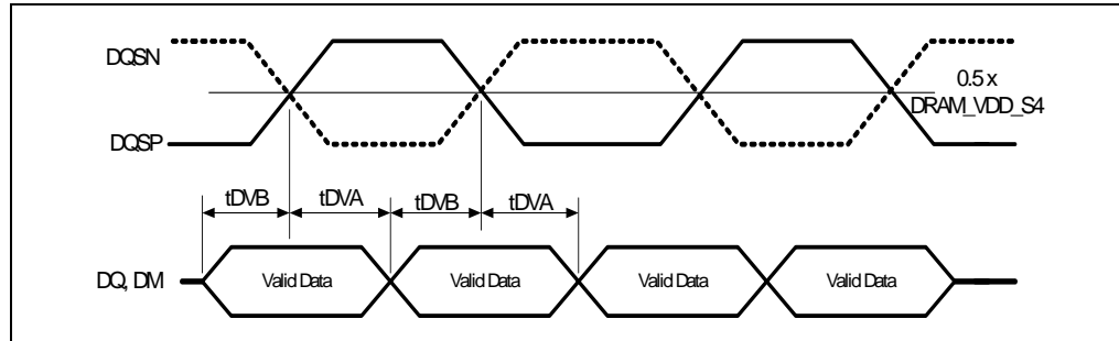
Figure 23. DDR3L Write Pre-amble Duration
