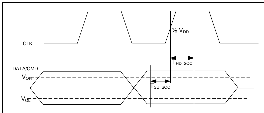
Figure 42. SD Card Input Timing Diagram (SDR12)
