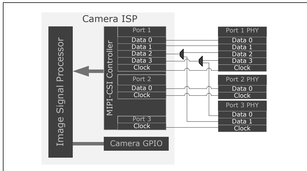
Figure 96. Camera Connectivity
