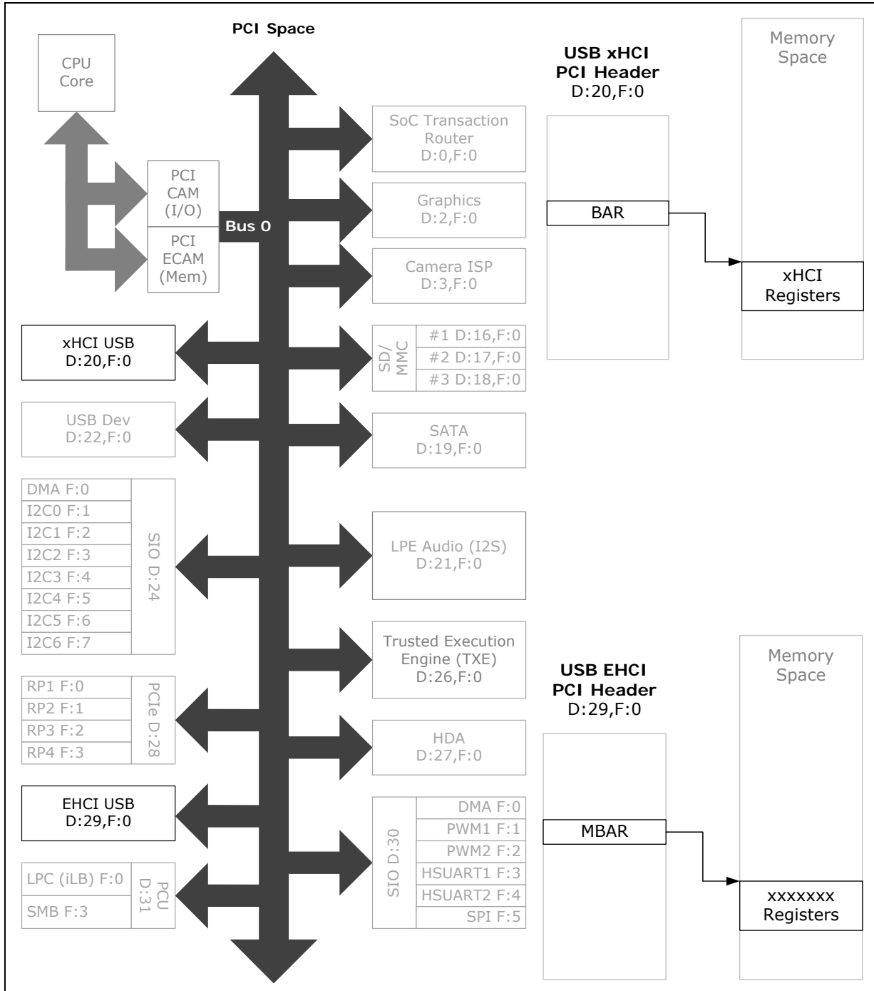
Figure 106.USB Host Controller Register Map
