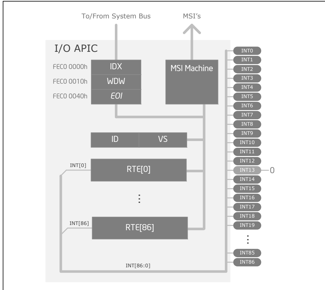
Figure 139. Detailed Block Diagram
