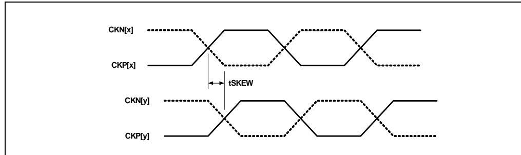
Figure 30. DDR3L Skew between System Memory Differential Clock Pairs (CKP/CKN)
