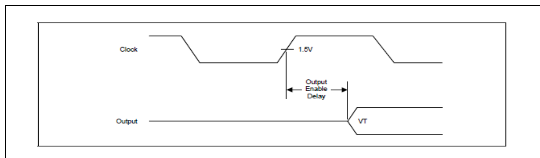
Figure 73. Output Enable Delay
