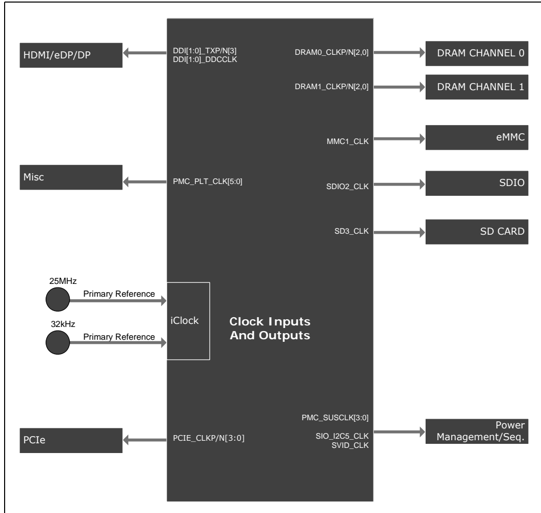
Figure 9. Clocking Example
