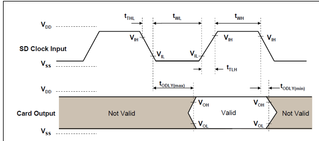
Figure 44. SD card Output Timing Diagram (Default)
