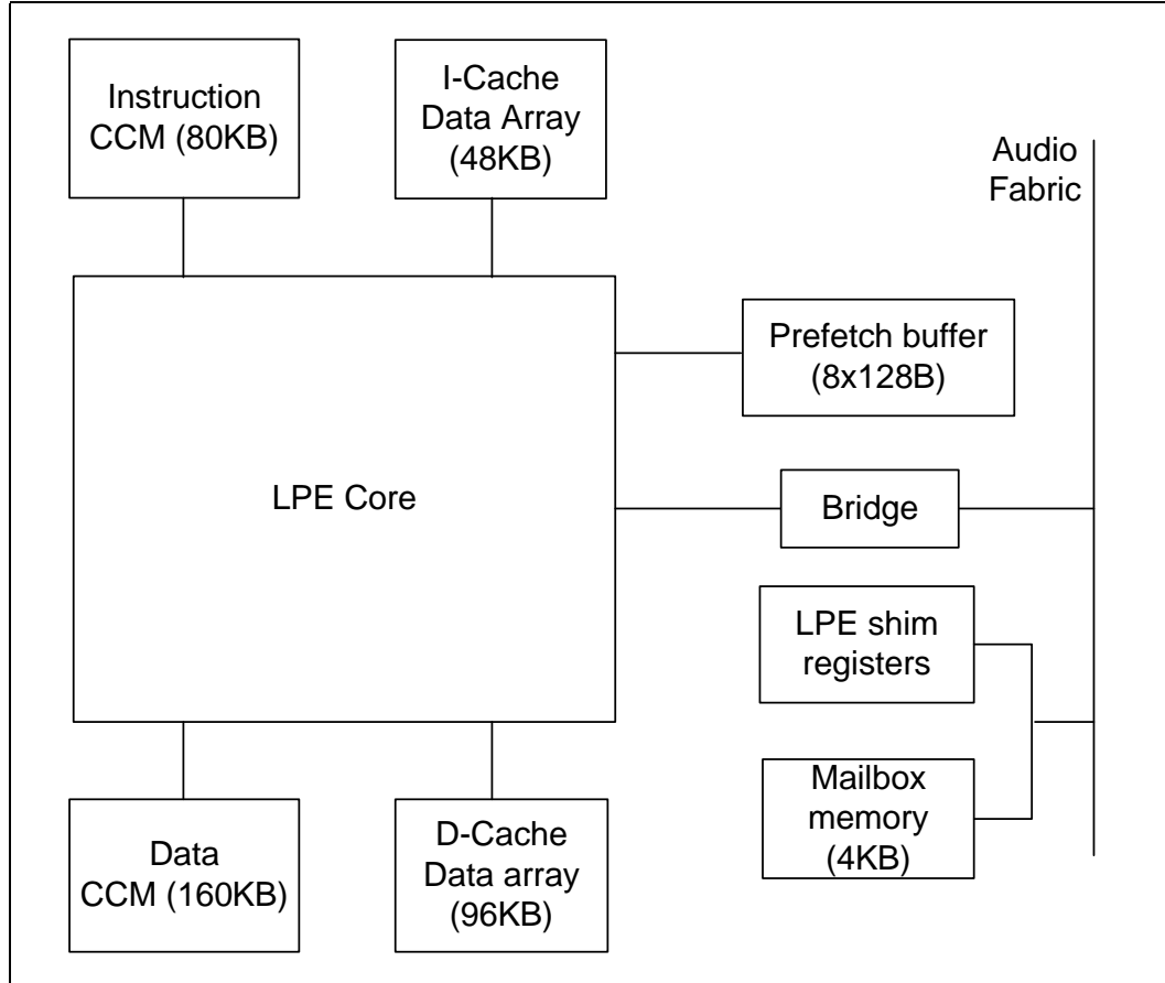
Figure 109. Memory Connections for LPE
