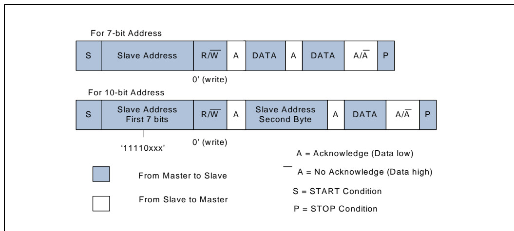
Figure 124. Master Transmitter Protocol
