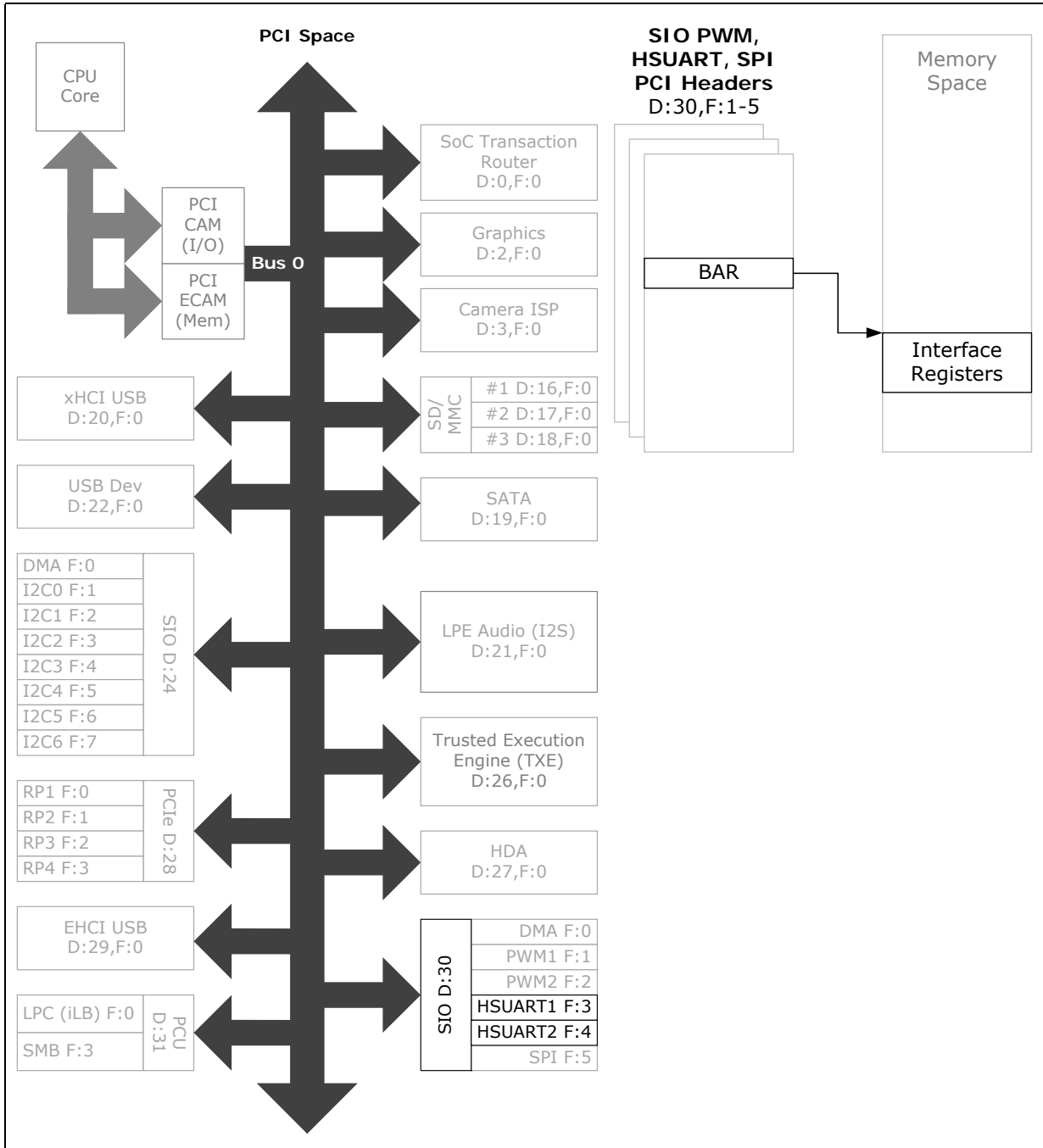
Figure 129.SIO - HSUART Register Map
