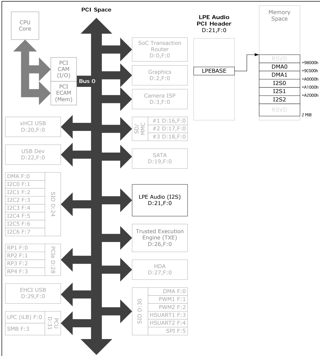
Figure 113. Low Power Engine for Audio Register Map
