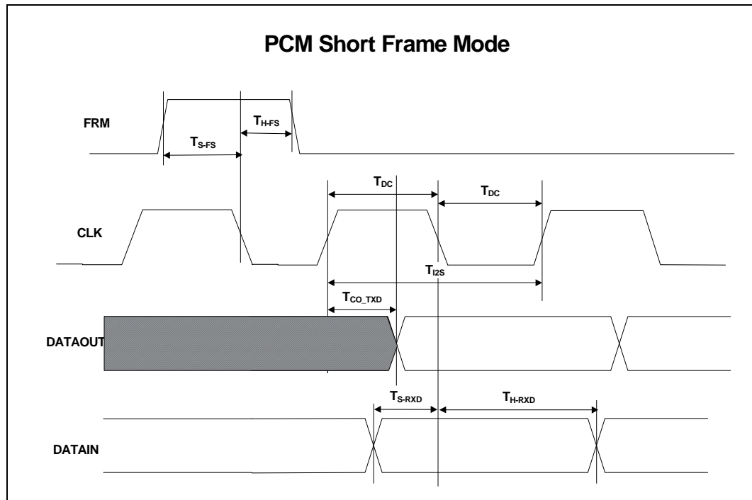
Figure 65. I 2 S Slave Port Timings in PCM Short Frame Mode
