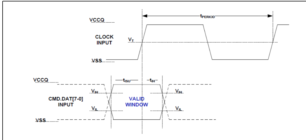
Figure 55. eMMC Input Timing Diagram (HS200 Mode)
