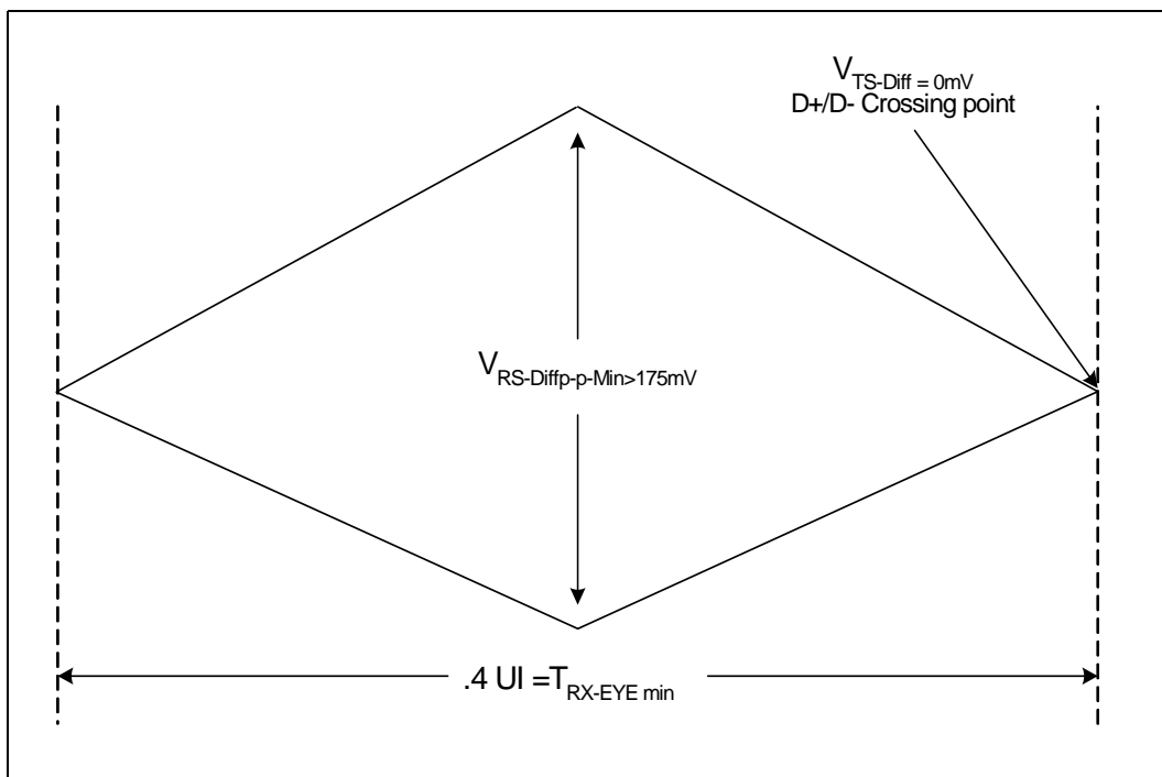
Figure 68. PCI Express* Receiver Eye
