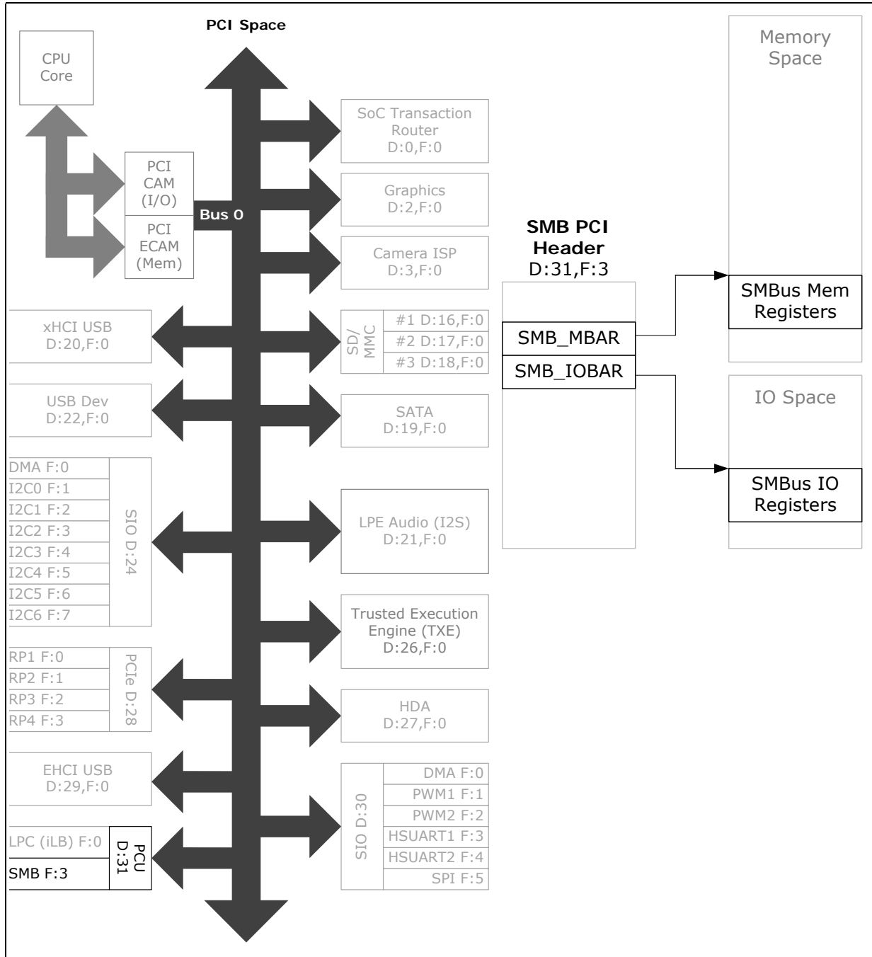
Figure 135.PCU - SMBus Register Map
