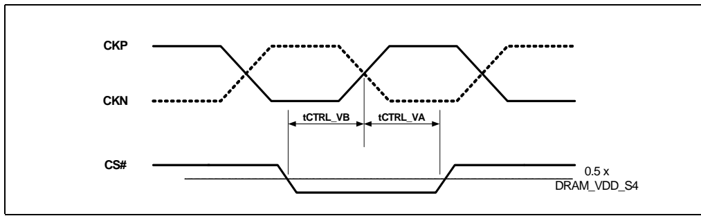
Figure 28. DDR3L ODT Valid before CK Rising Edge
