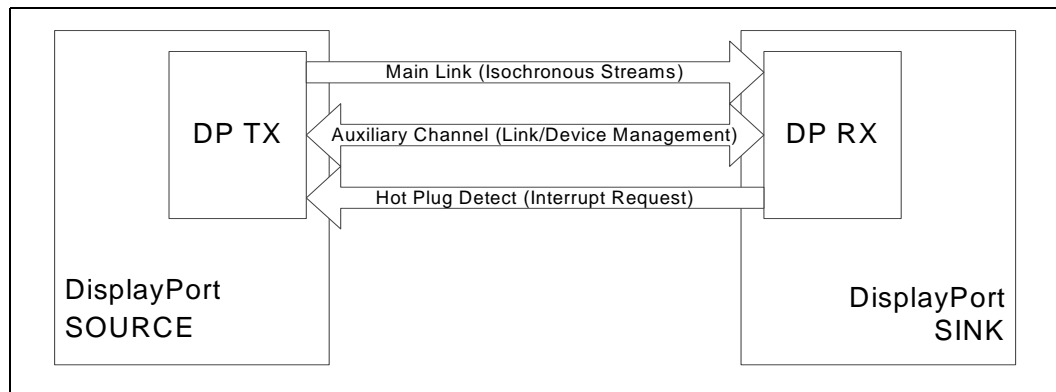
Figure 94. DisplayPort* Overview
