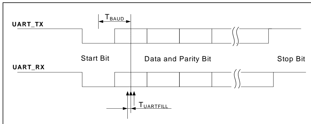
Figure 78. UART Timing Diagram
