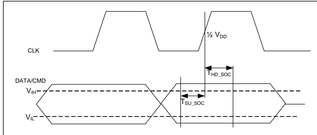
Figure 50. SDIO Input Timing Diagram (SDR12/25)
