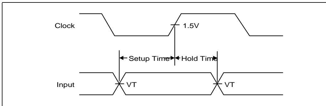
Figure 85. Setup and Hold Times
