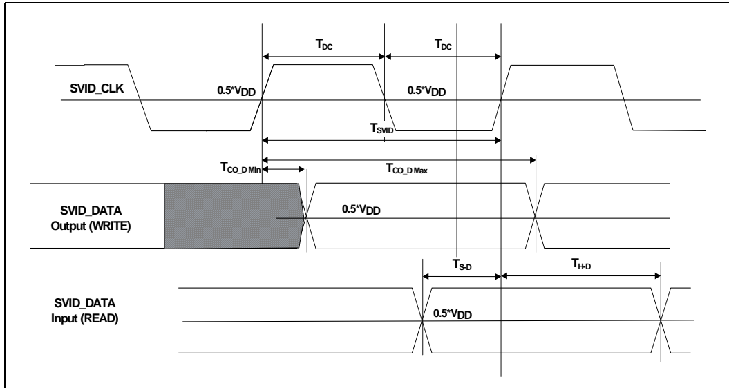
Figure 20. SVID Timing Diagram
