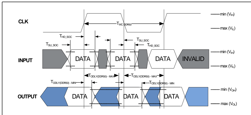
Figure 40. SD Card Timing Diagram (DDR50)
