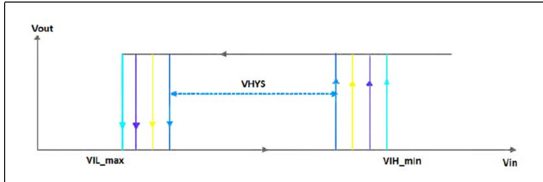
Figure 18. Definition of VHYS in Table 169
