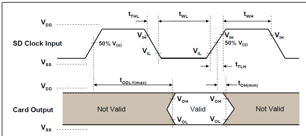
Figure 46. SD card Output Timing Diagram (High Speed)
