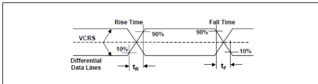
Figure 56. USB Rise and Fall Times
