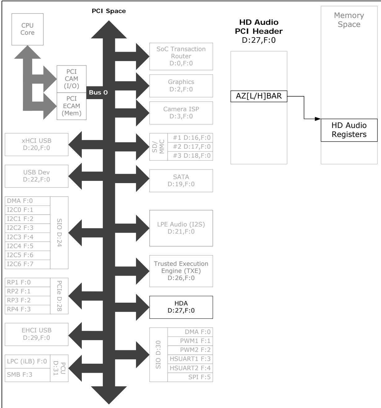
Figure 107. Intel® HD Audio Register Map
