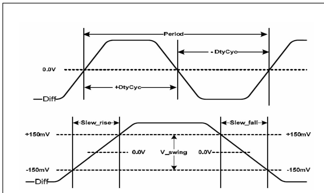
Figure 90. Differential Clock Waveform (Using Differential Probe for Measurement)
