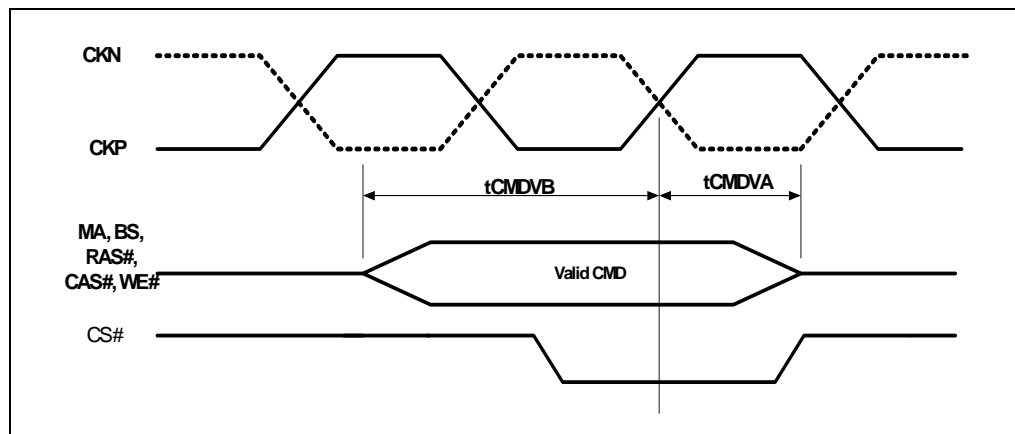
Figure 25. DDR3L Command Signals Valid before and after CK Rising Edge
