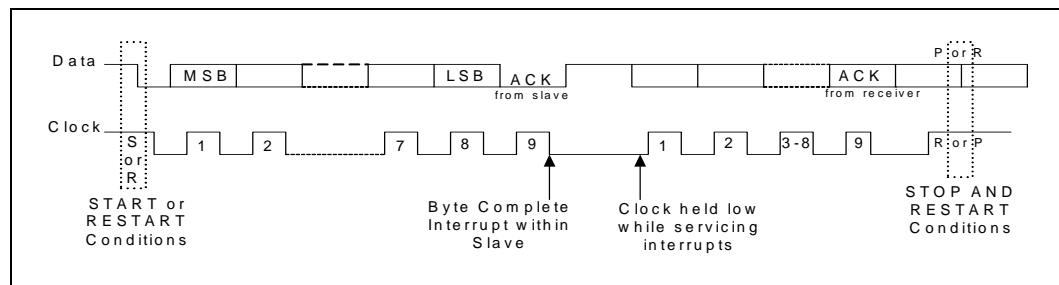
Figure 120. Data Transfer on the I 2 C Bus
