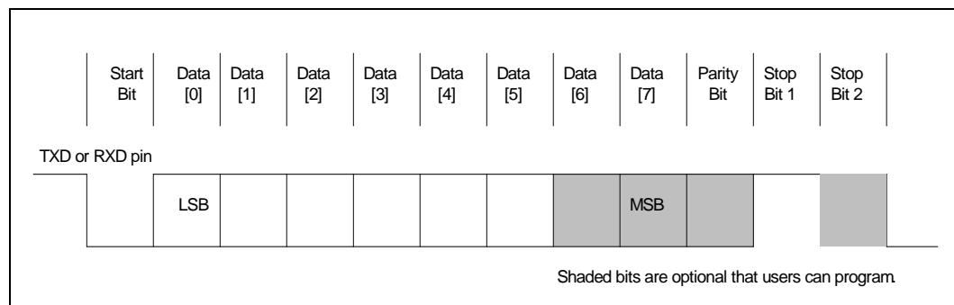
Figure 128. UART Data Transfer Flow
