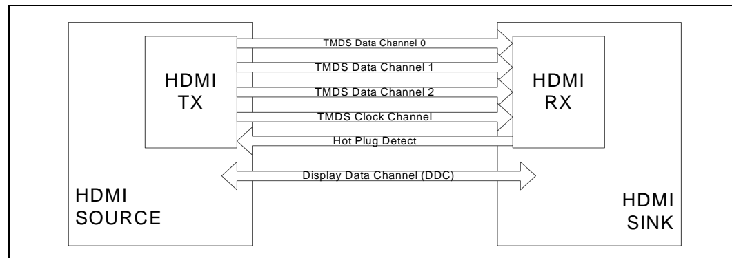
Figure 93. HDMI Overview
