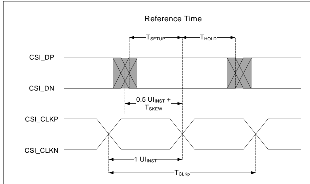
Figure 39. MIPI-CSI-2 Data to Clock Timing Definitions
