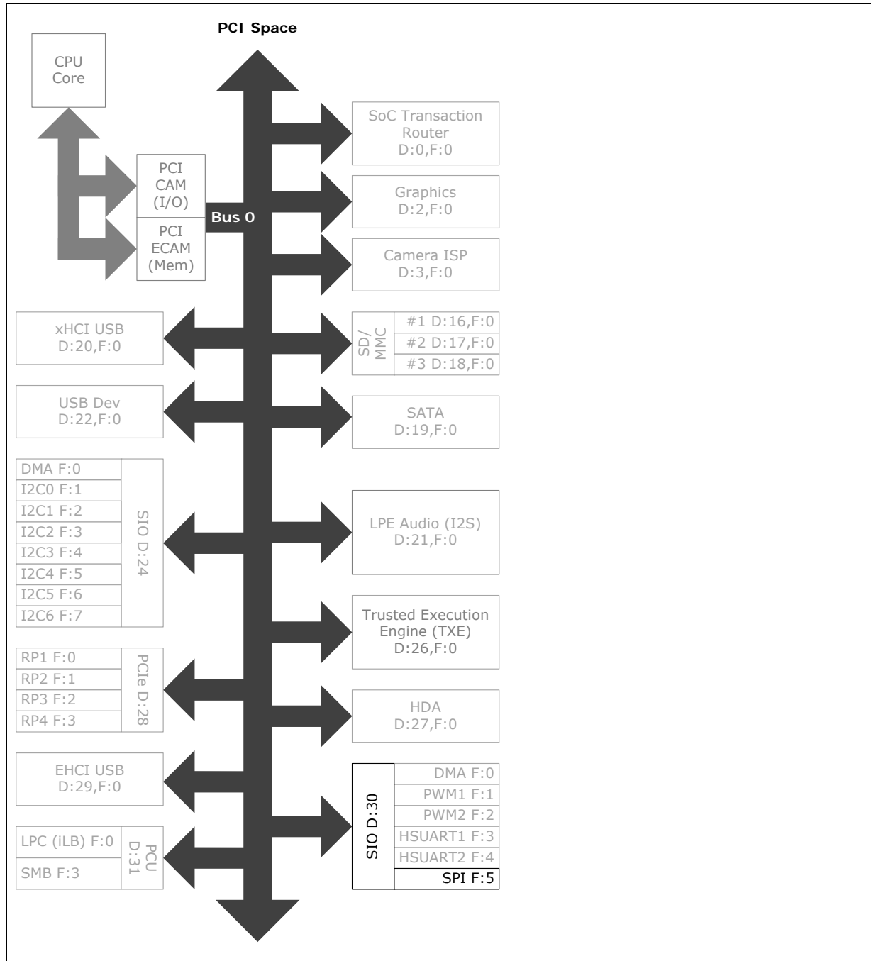
Figure 119.SIO - SPI Register Map
