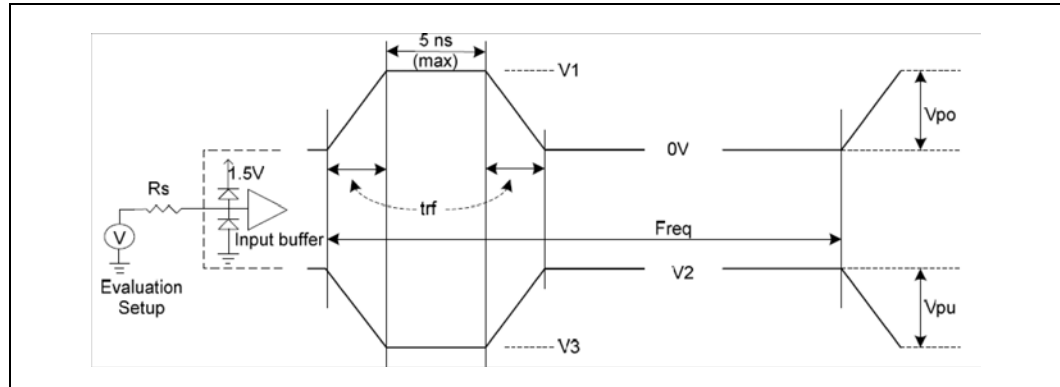
Figure 63. Maximum AC Waveforms for 1.5 V Signaling
