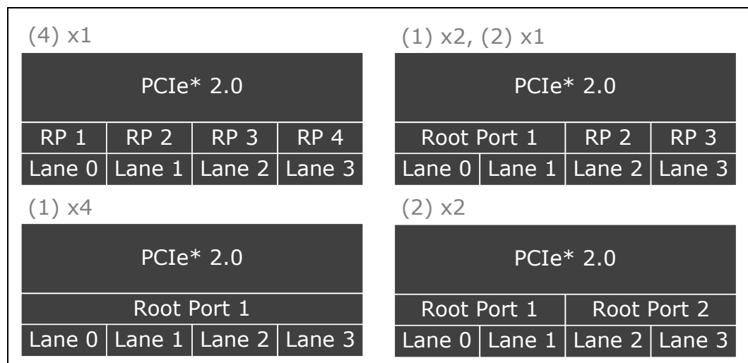
Figure 115. Root Port Configuration Options
