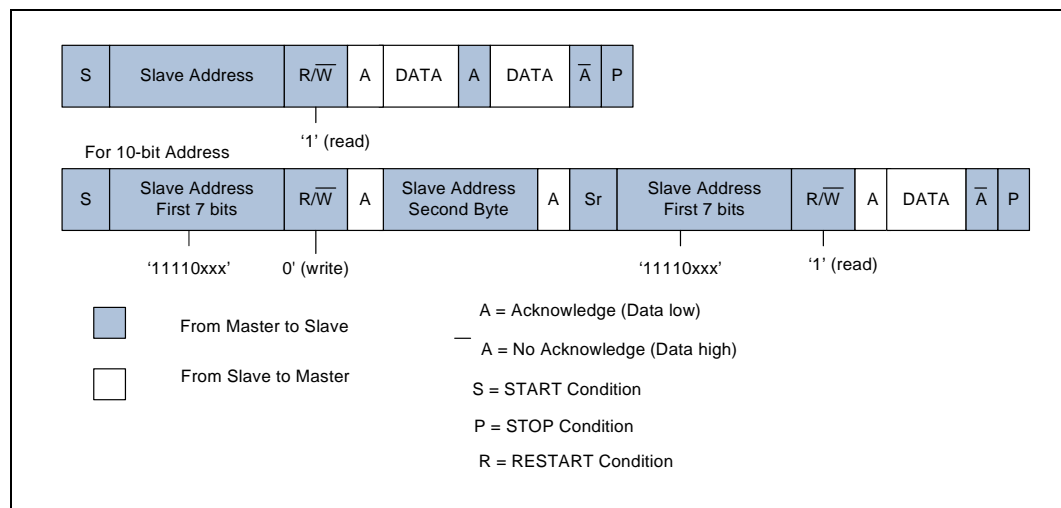
Figure 125. Master Receiver Protocol
