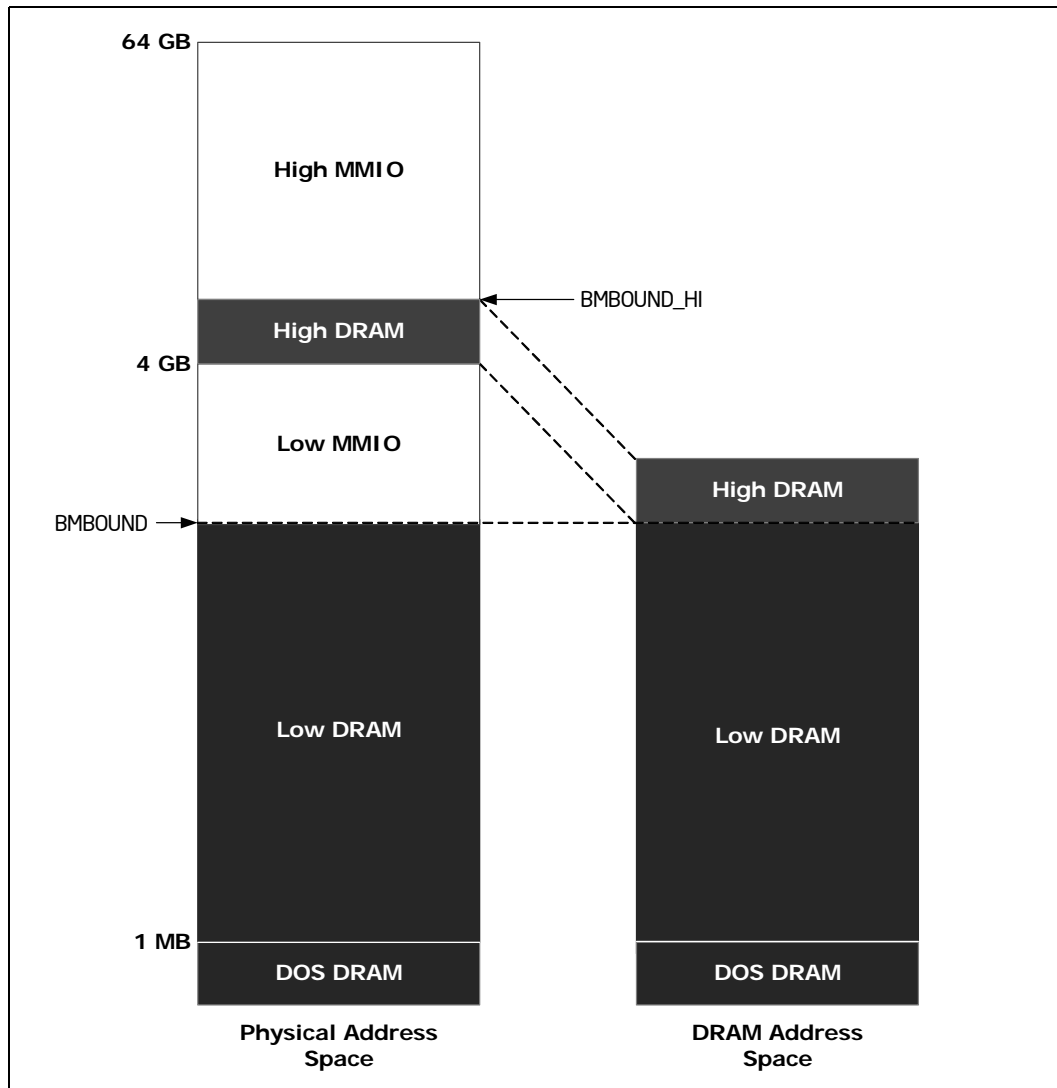
Figure 4. Physical Address Space - DRAM & MMIO
