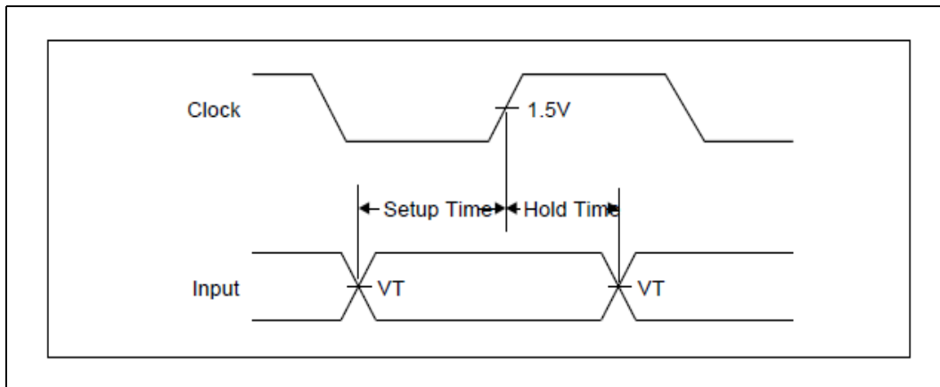
Figure 75. Setup and Hold Times
