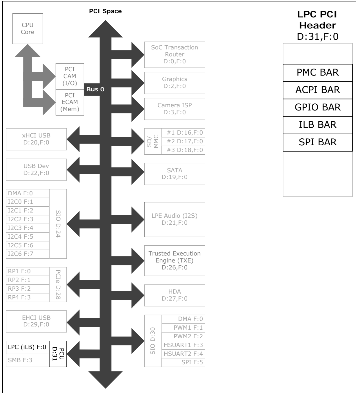
Figure 137. PCU - iLB - LPC Register Map
