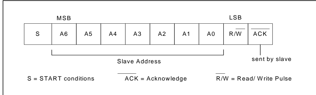
Figure 122. Seven-Bit Address Format
