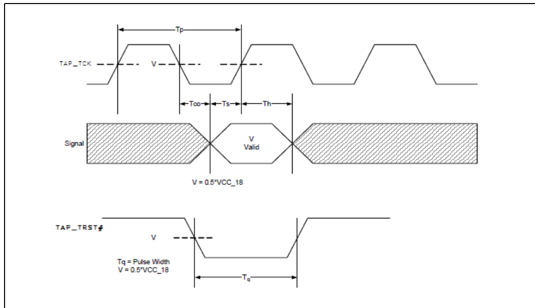
Figure 79. JTAG Timing Diagram
