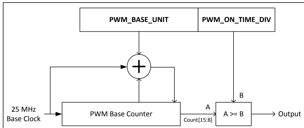
Figure 131. PWM Block Diagram
