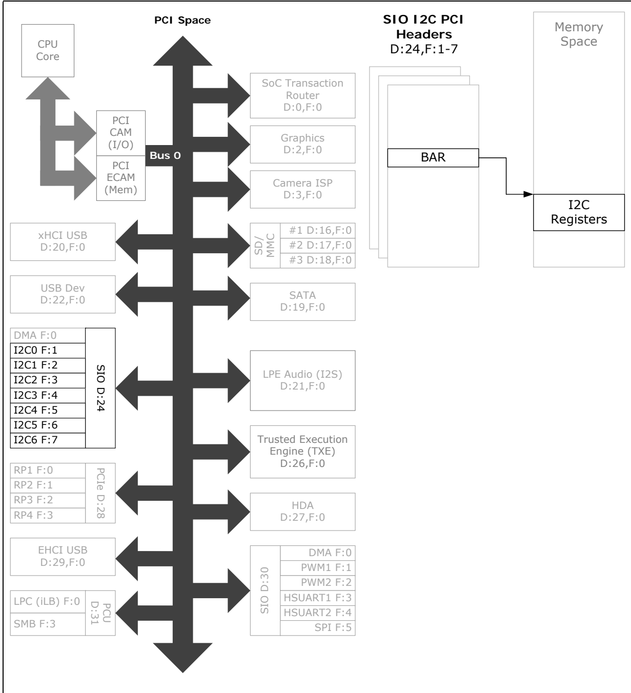
Figure 127.SIO - I 2 C Register Map
