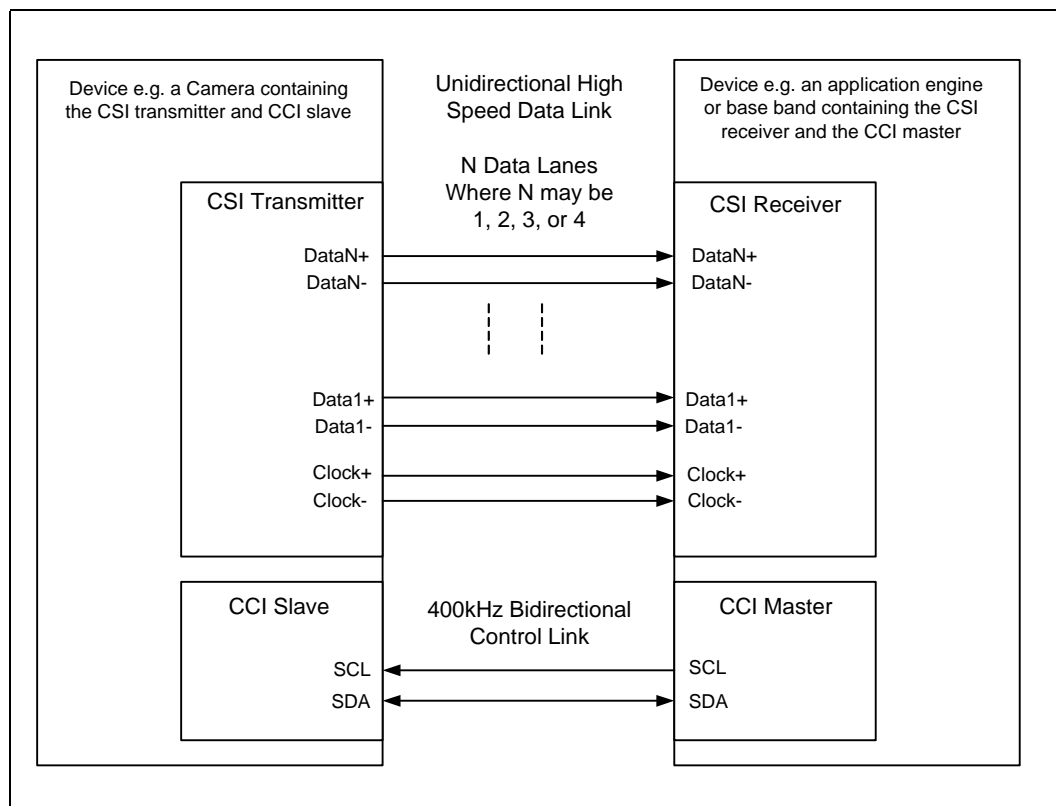
Figure 98. MIPI-CSI Bus Block Diagram
