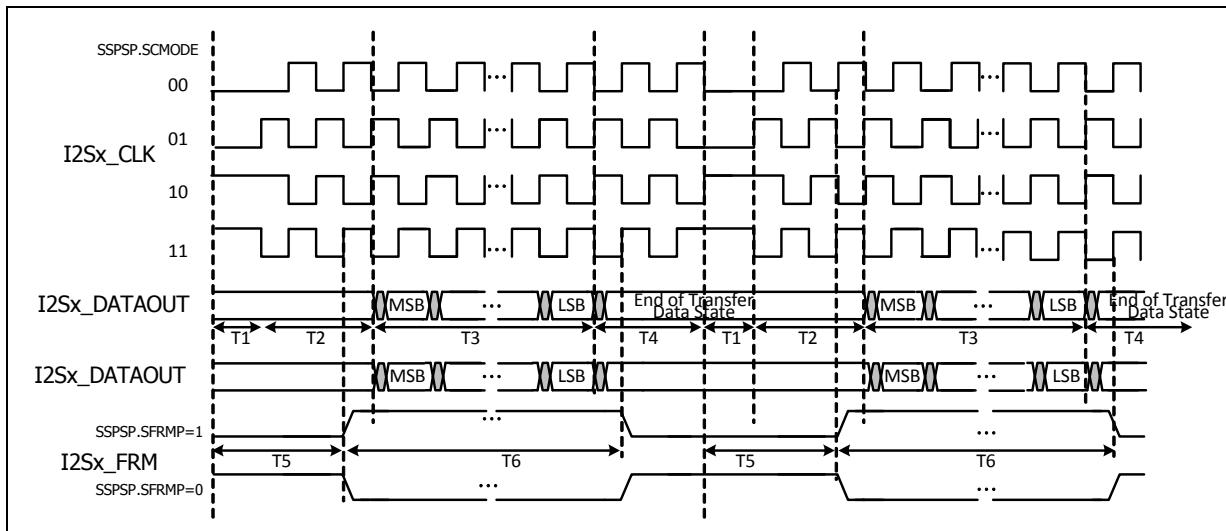
Figure 112. Programmable Serial Protocol Format (Consecutive Transfers)
