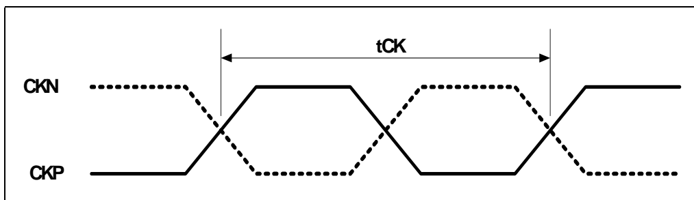
Figure 29. DDR3L Clock Cycle Time
