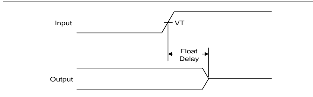
Figure 87. Pulse Width
