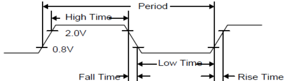
Figure 19. Crystal Clock Timing
