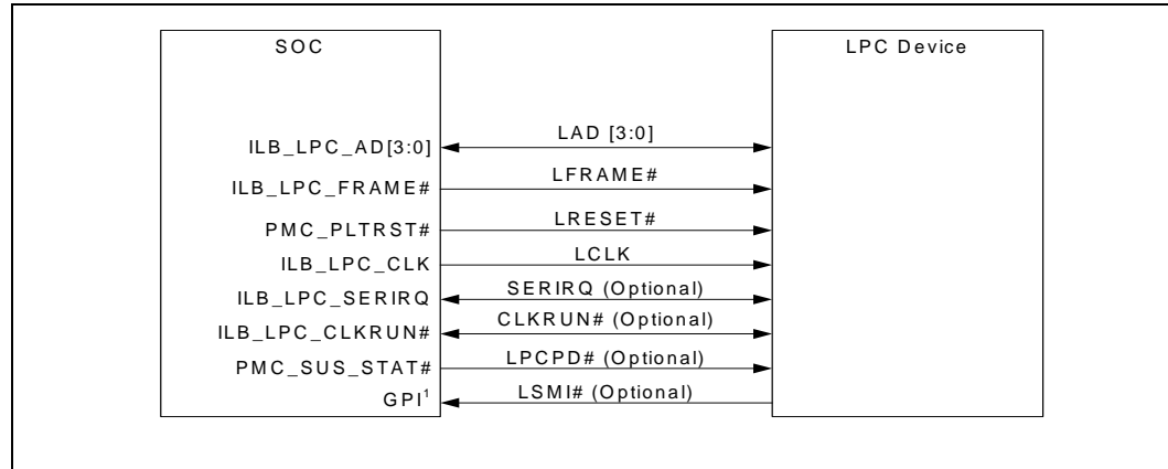
Figure 136.LPC Interface Diagram
