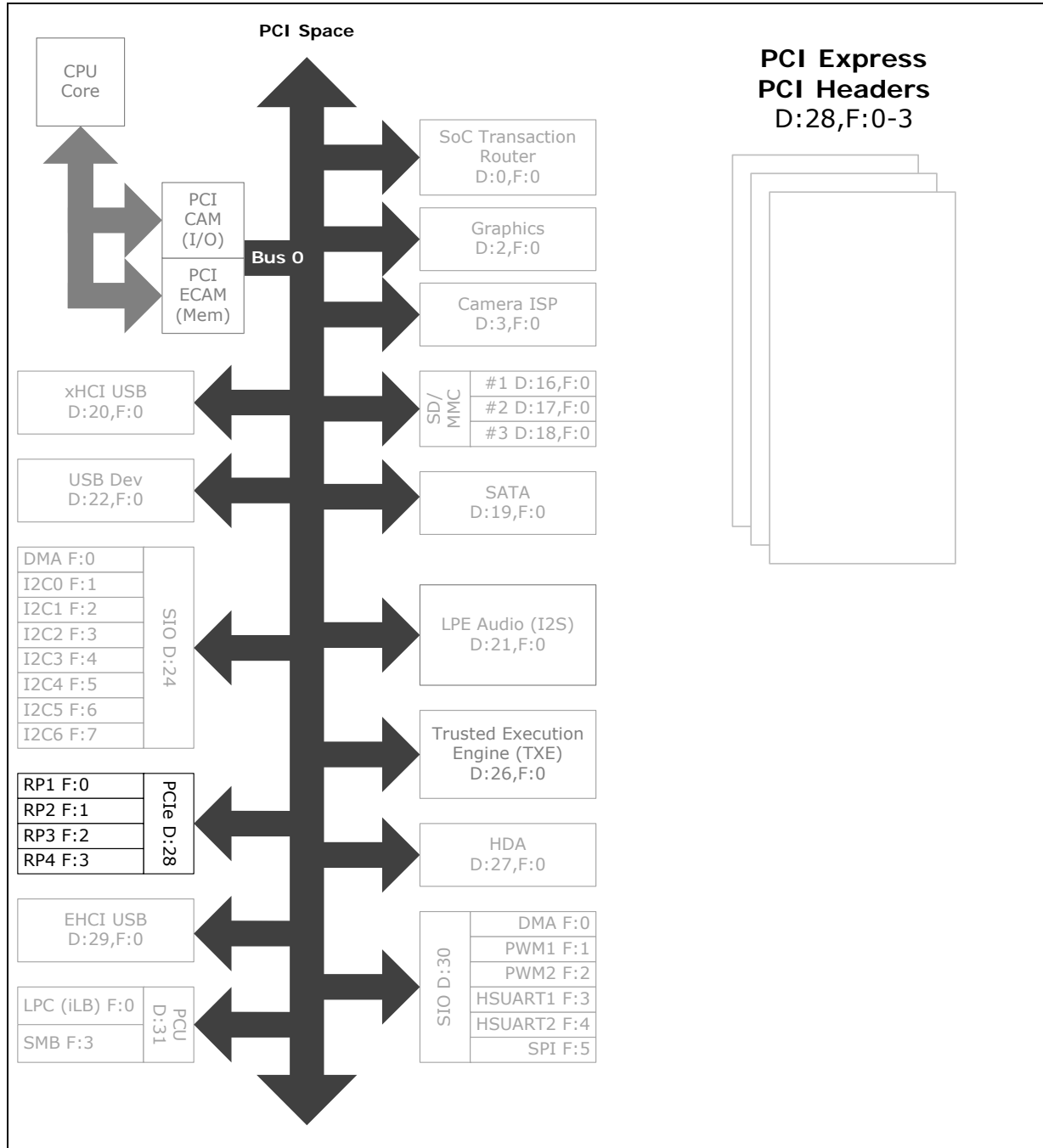
Figure 116. PCI Express Register Map
