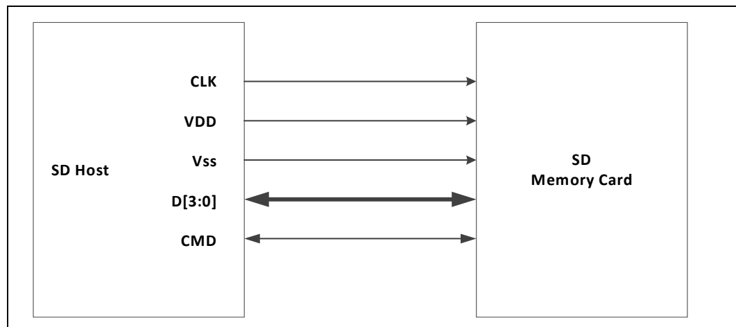
Figure 100. SD Memory Card Bus Topology
