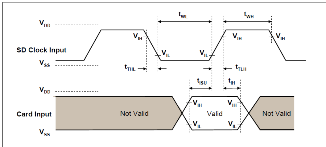
Figure 43. SD Card Input Timing Diagram (Default)
