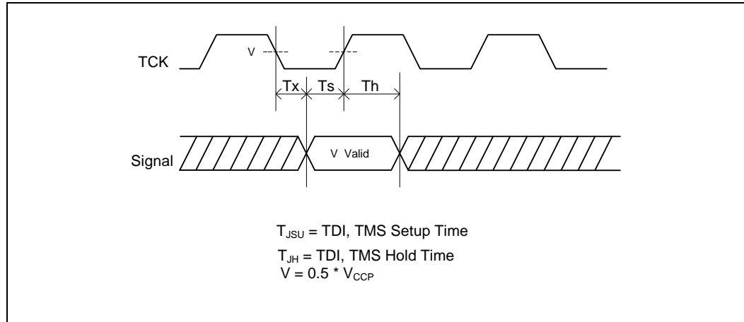
Figure 80. TAP Valid Delay Timing Waveform
