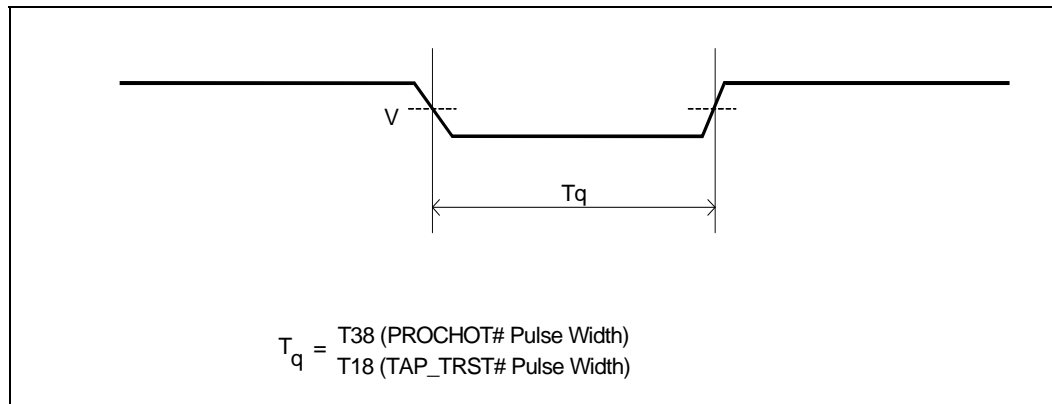
Figure 81. Test Reset (TAP_TRST#), Async GTL Input and PROCHOT# Timing Waveform
