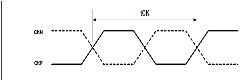
Figure 83. Clock Timing
