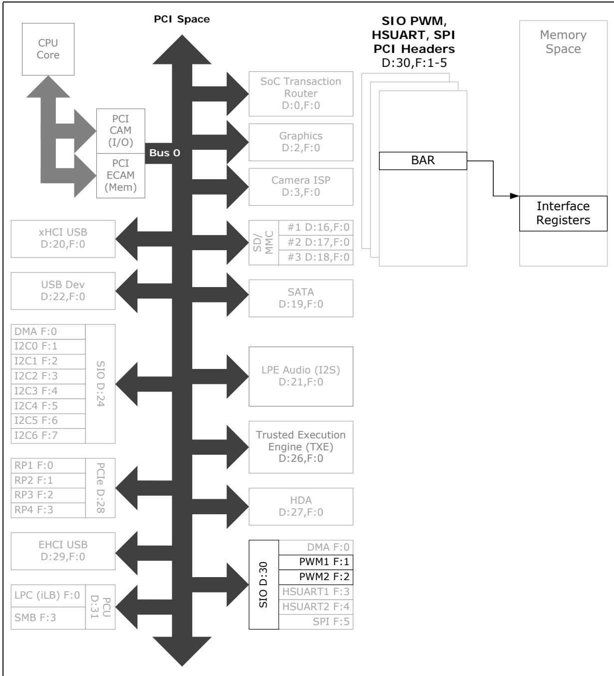
Figure 132.SIO - PWM Register Map
