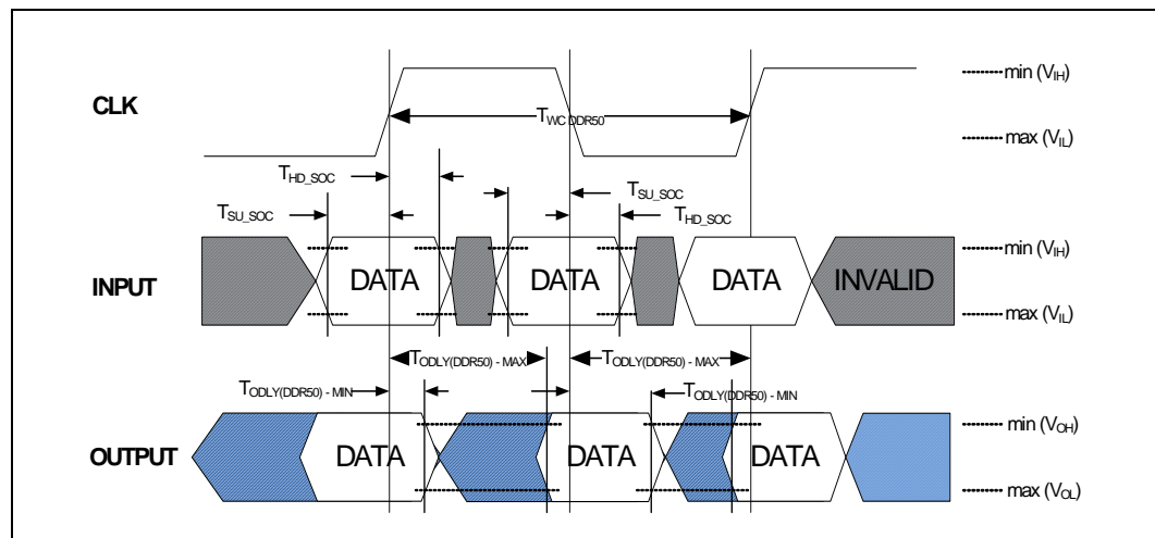
Figure 47. SDIO Timing Diagram (DDR50)
