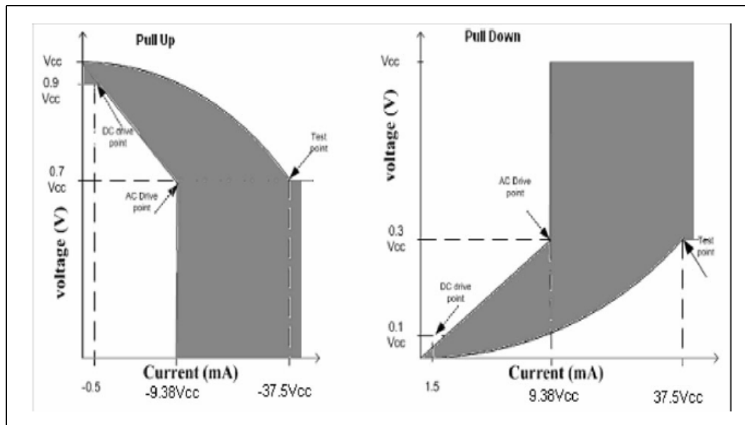
Figure 62. V/I Curves for HDA_SDO buffers
