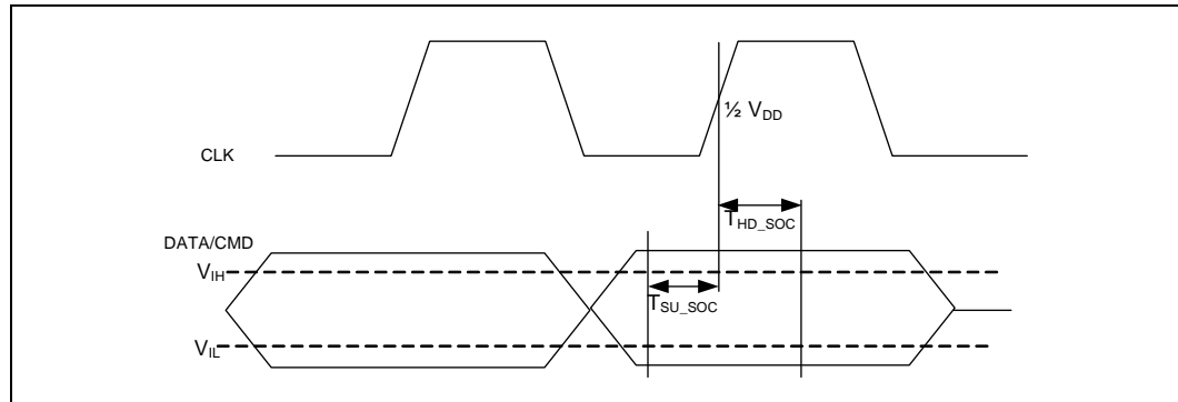
Figure 53. eMMC* Input Timing Diagram (High Speed Mode)
