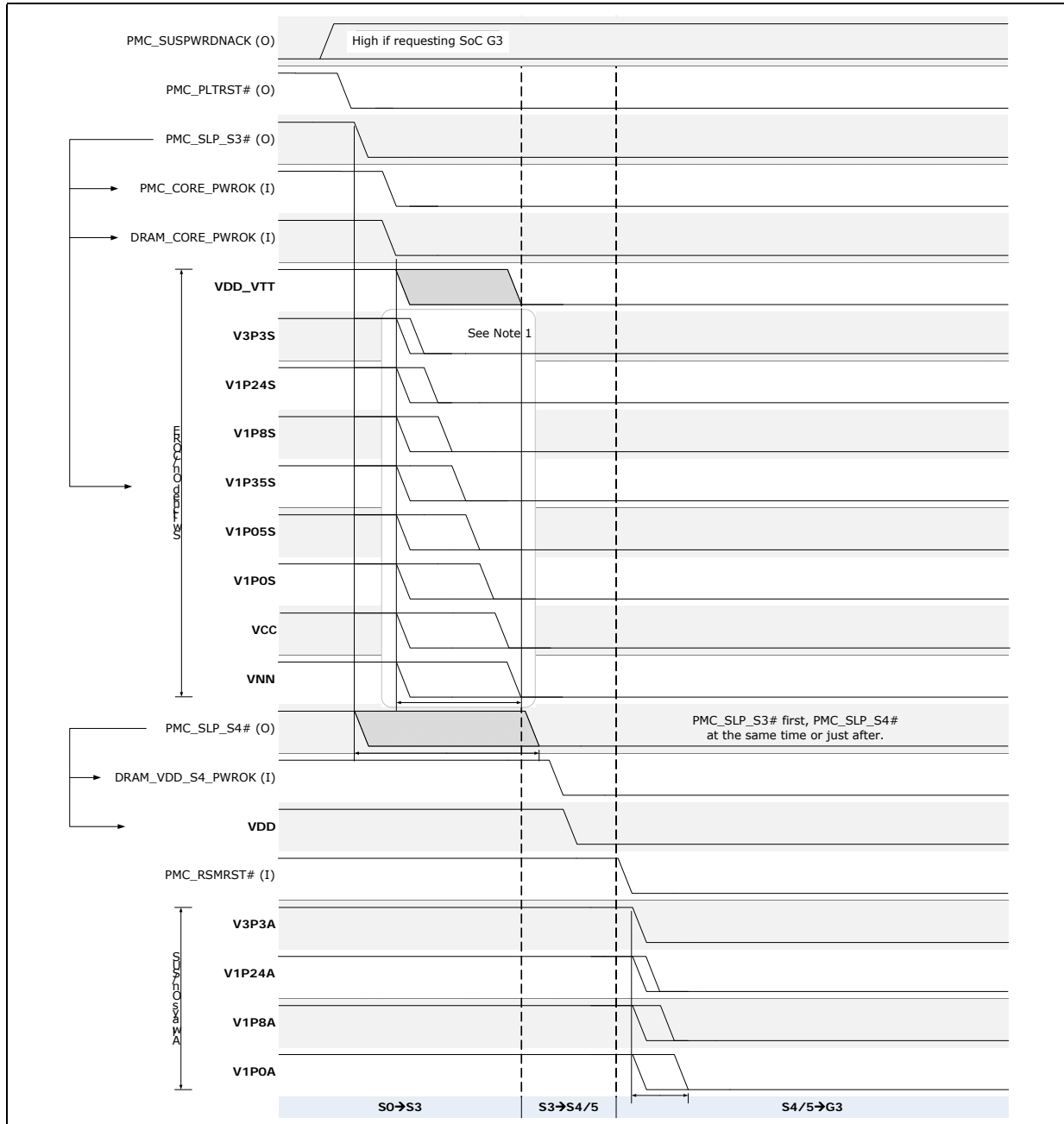
Figure 14. S0 to S3 to S4/S5 (Power Down) Sequence without S0ix
