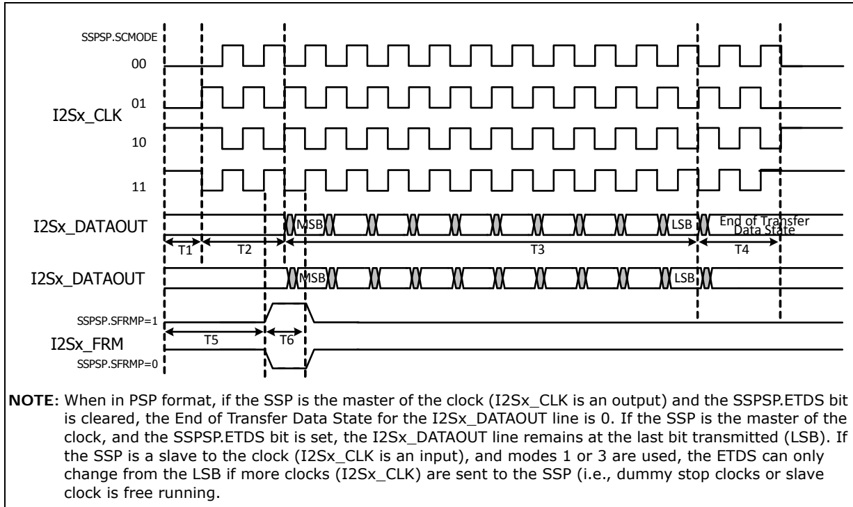
Figure 112. Programmable Serial Protocol Format (Consecutive Transfers)
