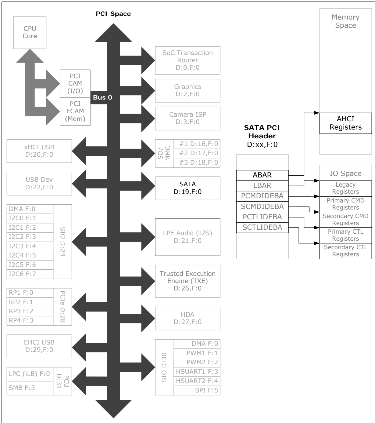
Figure 104.SATA Register Map
