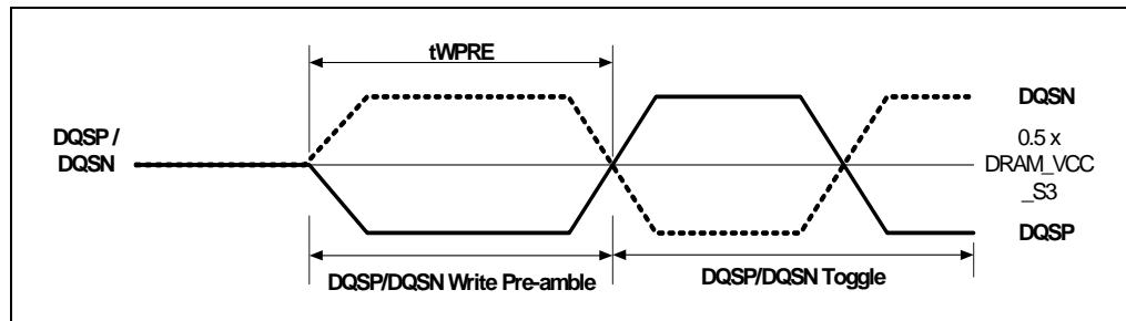
Figure 24. DDR3L Write Post-amble Duration
