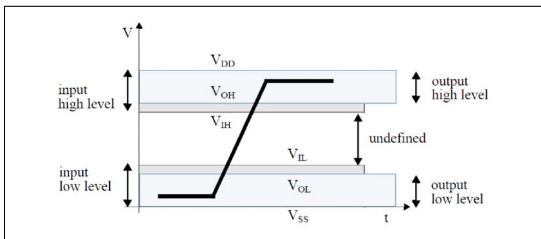
Figure 17. eMMC DC Bus signal level
