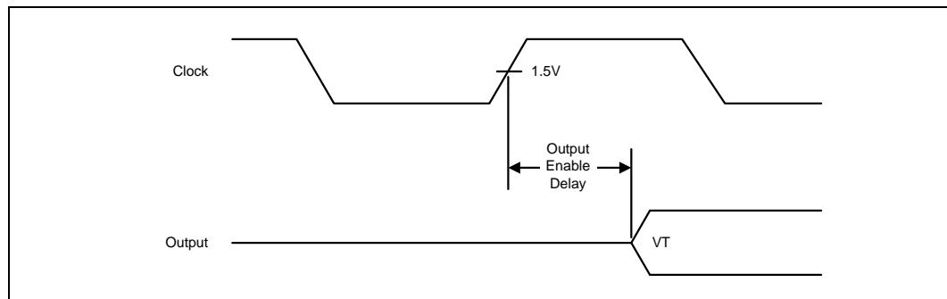
Figure 88. Output Enable Delay
