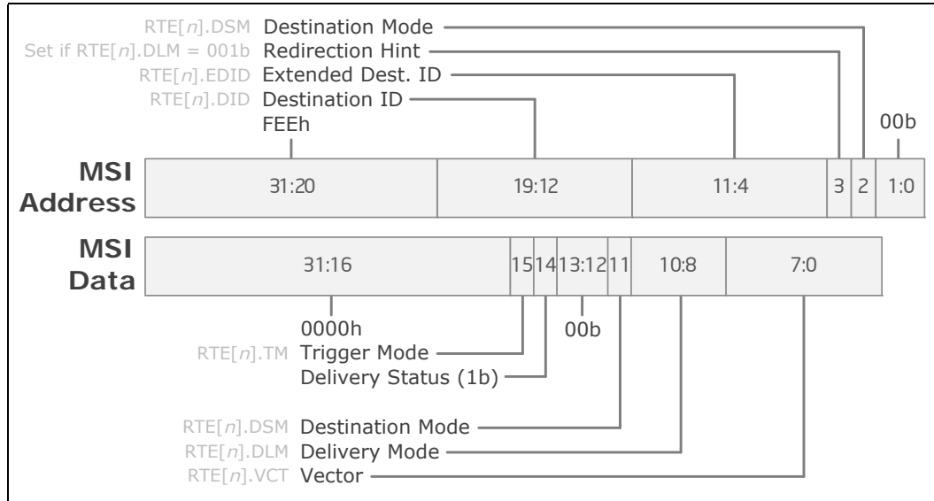
Figure 140.MSI Address and Data
