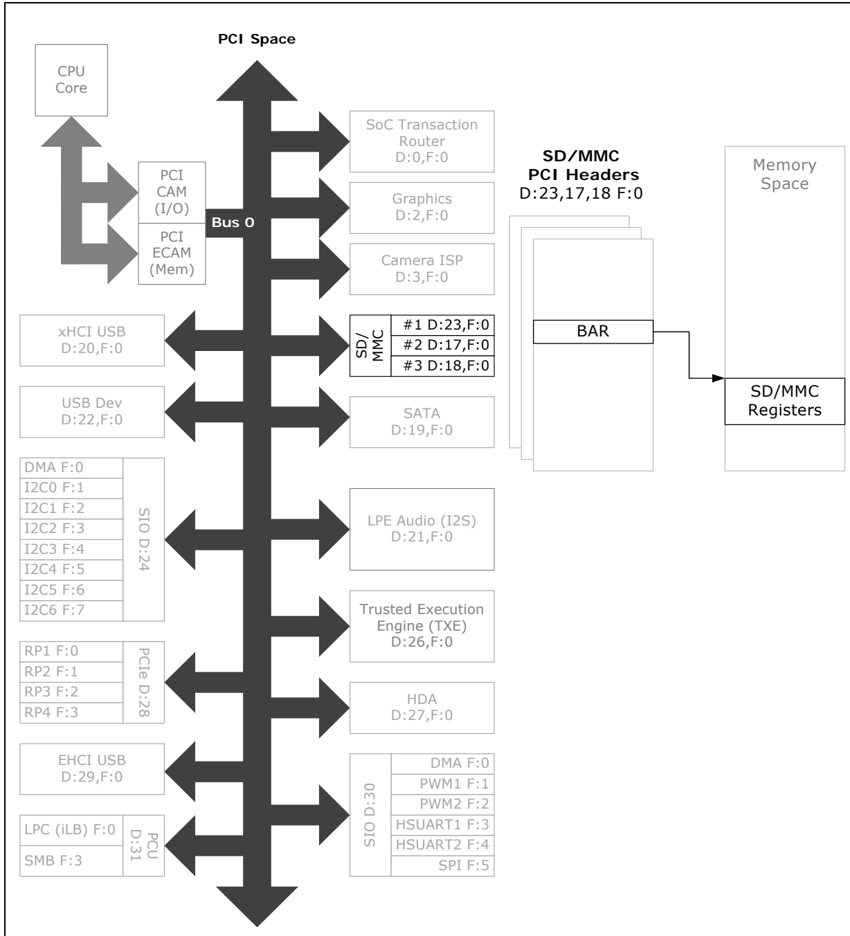
Figure 103.Storage Control Cluster Register Map
