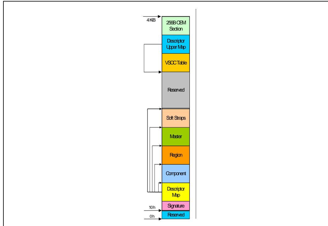
Figure 133. Flash Descriptor Sections
