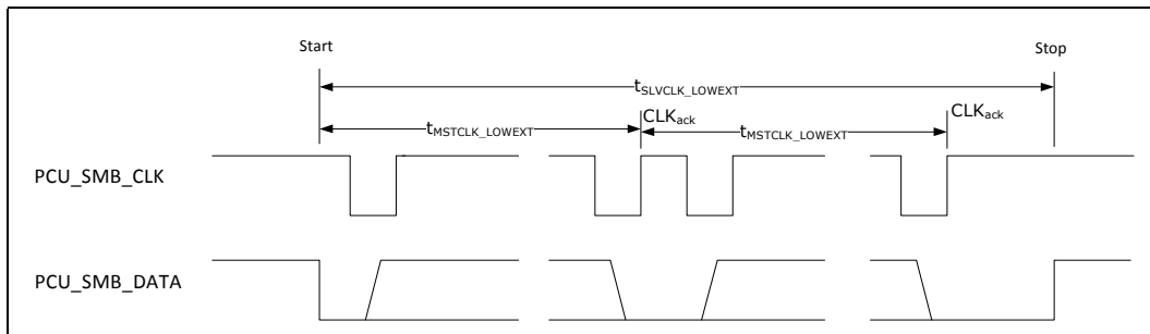
Figure 71. SMBus Timeout
