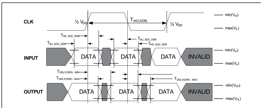
Figure 52. eMMC* DDR Timings
