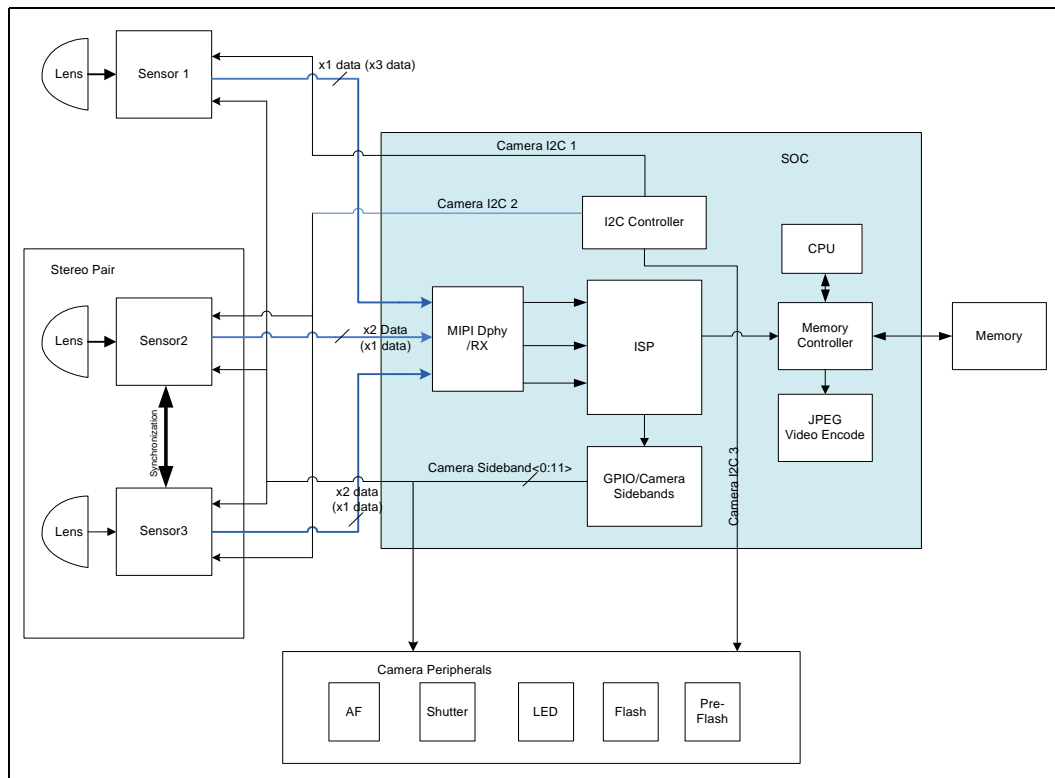
Figure 97. Image Processing Components
