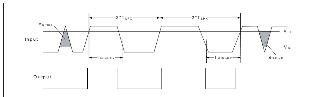
Figure 37. Input Glitch Rejection of Low-Power Receivers
