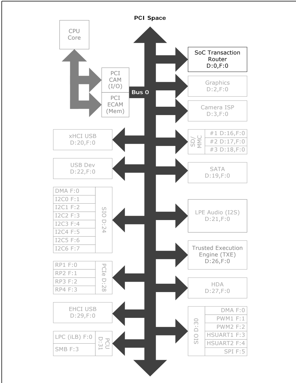
Figure 92. Soc Transaction Router Register Map
