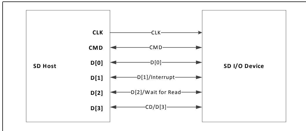
Figure 101. SDIO Device Bus Topology
