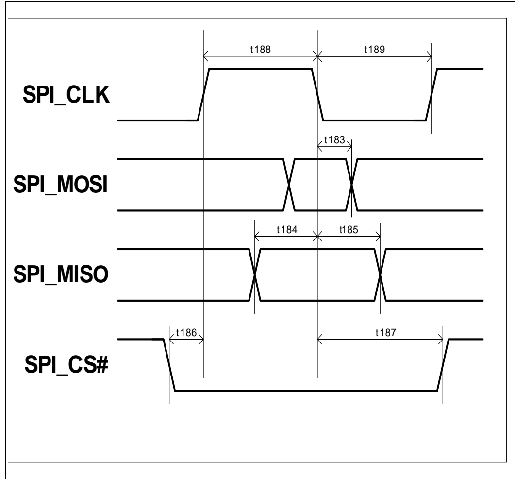
Figure 69. SPI NOR timing
