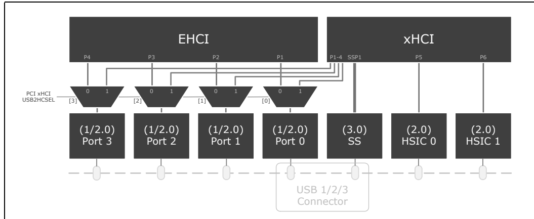
Figure 105.xHCI and EHCI Port Mapping
