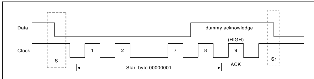
Figure 126. START Byte Transfer
