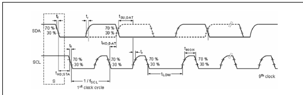
Figure 36. VGA_DDCDATA, and VGA_DDCCLK Timing Diagram
