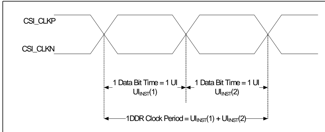
Figure 38. MIPI-CSI-2 Clock Definition
