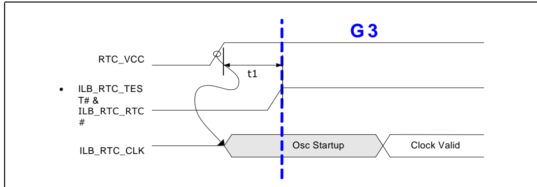
Figure 12. RTC Power Well Timing Diagrams
