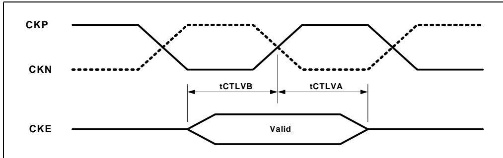
Figure 27. DDR3L CS# Valid before and after CK Rising Edge
