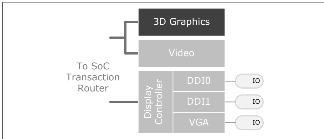
Figure 95. 3D Graphics Block Diagram
