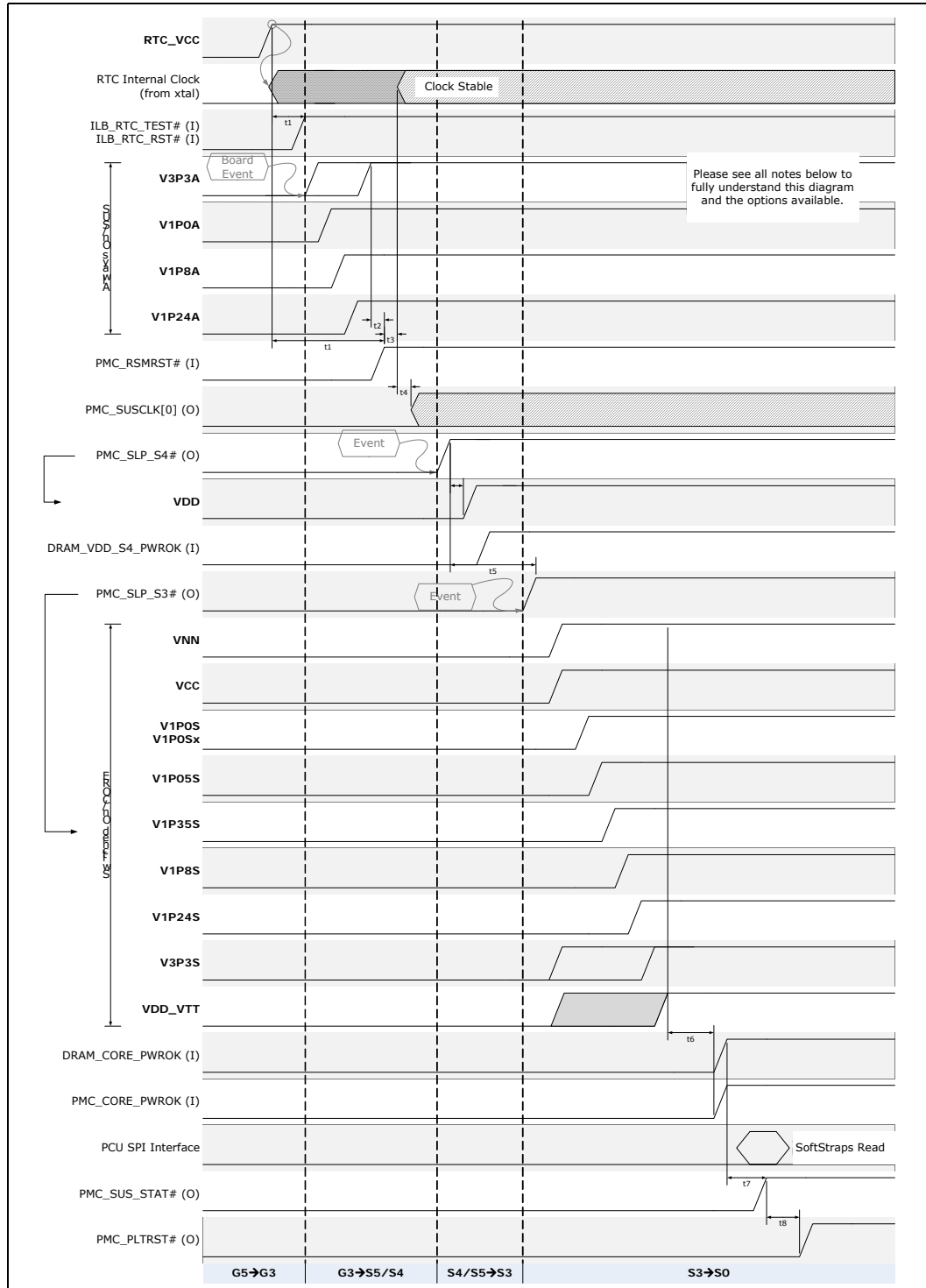
Figure 13. G3/S5 to S0 Cold Boot Sequence
