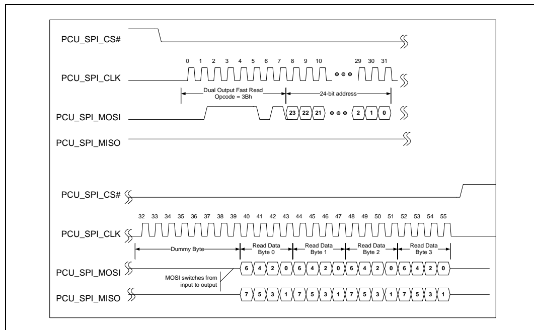
Figure 134. Dual Output Fast Read Timing
