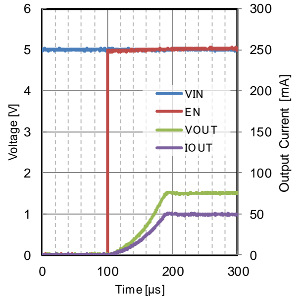
Figure 83. Start Up Waveform V_{OUT} = 1.5\text{ V} , I_{OUT} = 50\text{ mA} V_{IN} = 5.0\text{ V} , C_{OUT} = 10\ \mu\text{F} T_j = 25\text{ }^\circ\text{C}
