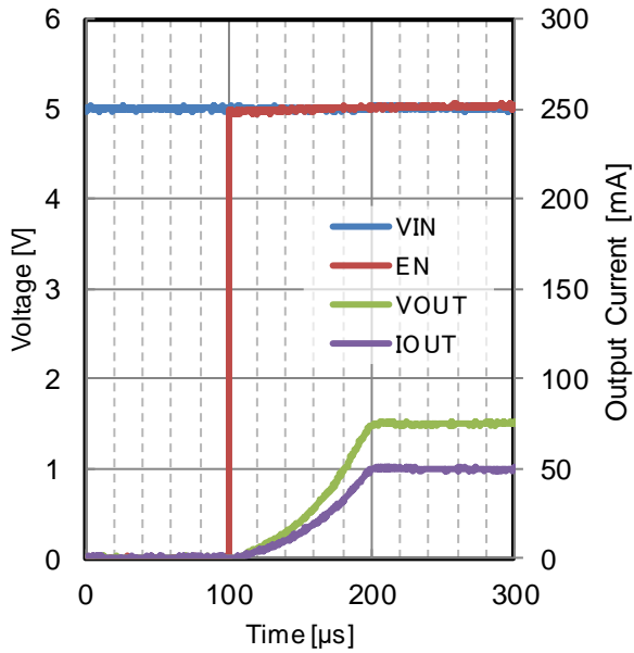
Figure 82. Start Up Waveform V_{OUT} = 1.5\text{ V} , I_{OUT} = 50\text{ mA} V_{IN} = 5.0\text{ V} , C_{OUT} = 10\ \mu\text{F} T_j = -40\text{ }^\circ\text{C}
