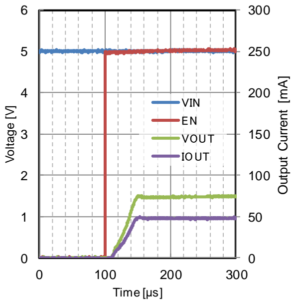
Figure 84. Start Up Waveform V_{OUT} = 1.5\text{ V} , I_{OUT} = 50\text{ mA} V_{IN} = 5.0\text{ V} , C_{OUT} = 10\ \mu\text{F} T_j = 150\text{ }^\circ\text{C}
