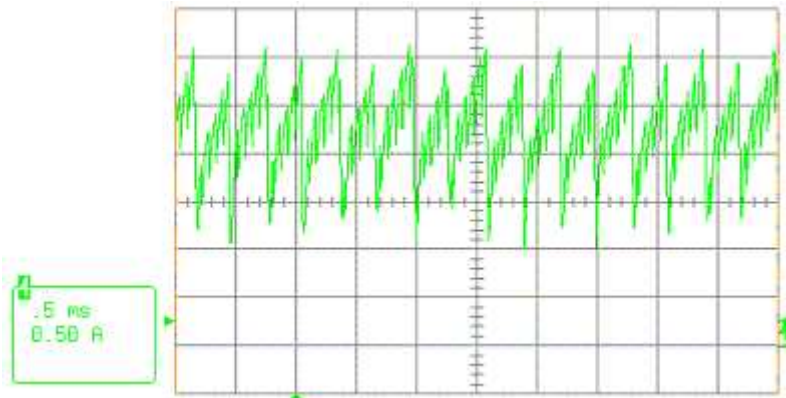
Typical running current @ 48 V, free blowing, 11.000 1/min
