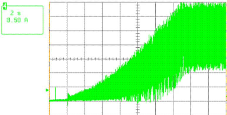
Start-up current @ 48 V, 0 - 11.000 1/min
