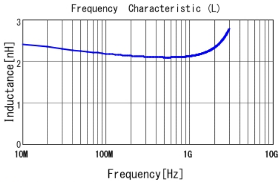
■ LQG15HS2N2S02 L
