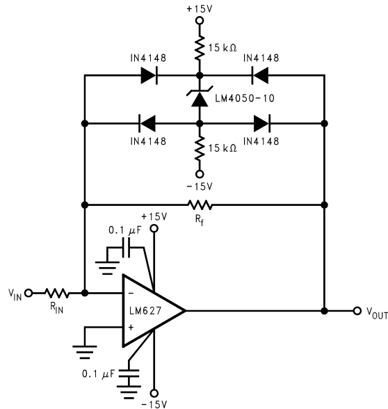
Figure 12. Bounded Amplifier
