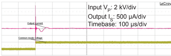
Figure 11: Typical common mode perturbation (2000 V step with 6 kV/μs R_M = 100 \Omega )
