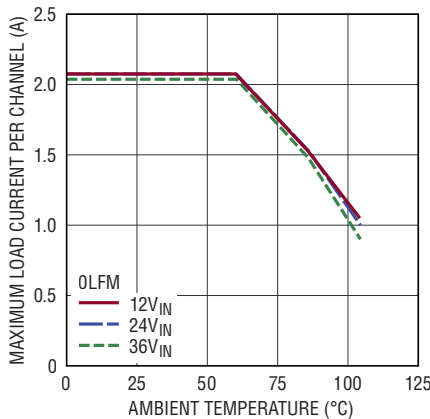
Derating, V_{OUT} = 1.2\text{V} \text{BIAS} = 5\text{V} , DC2777A Demo Board Both Channels at Same Load
