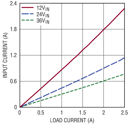
Input vs Load Current V_{OUT} = 10\text{V}
