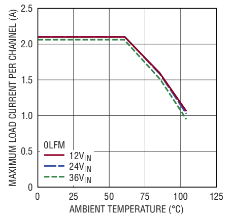
Derating, V_{OUT} = 1.0\text{V} , \text{BIAS} = 5\text{V} , DC2777A Demo Board Both Channels at Same Load
