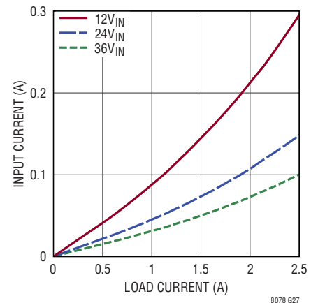
Input vs Load Current V_{OUT} = 0.8\text{V}
