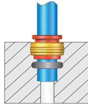
Assembly
