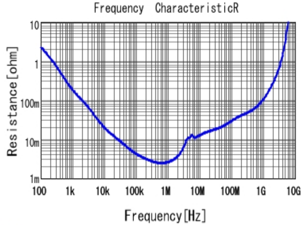
■ GRM21BR61C106KE15 R DCOV, 25degC
