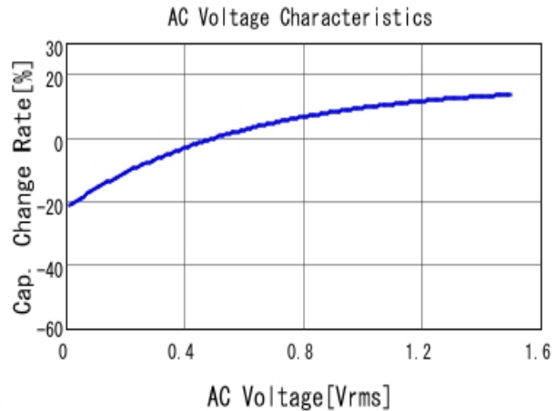
■ GRM21BR61C106KE15 C-AC Voltage capchange, DCOV, 25.0d
