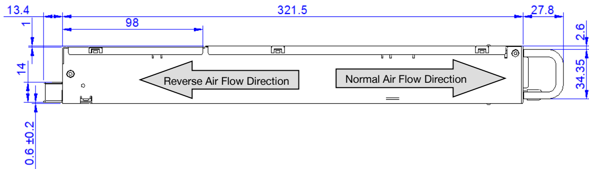
Figure 42. Side View 1
