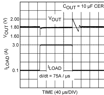
Figure 19. Load Transient Response: 10\ \mu\text{F} Ceramic, 75\text{A}/\mu\text{s} di/dt
