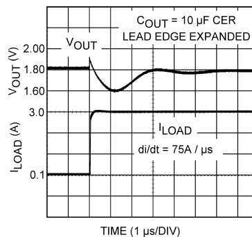
Figure 20. Rising Edge, 10\ \mu\text{F} Ceramic, 75\text{A}/\mu\text{s} di/dt
