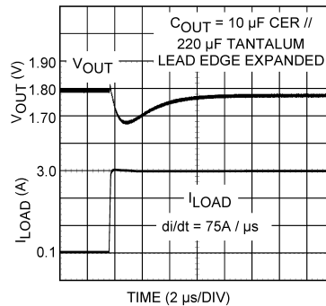
Figure 24. 10 \mu\text{F} Ceramic Paralleled By 220 \mu\text{F} Tantalum
