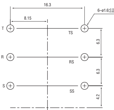
PCB LAYOUT (±0.1) (Bottom View)
