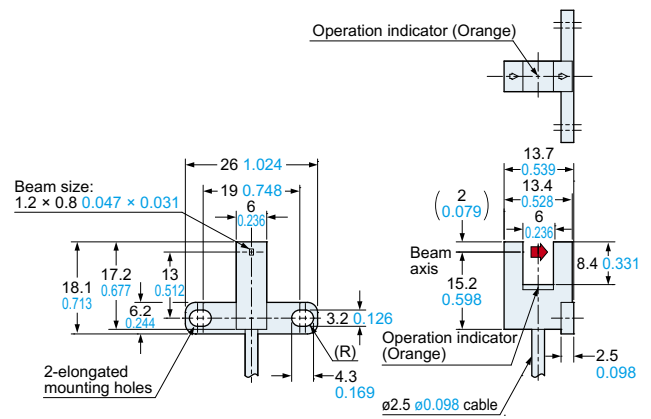
PM-T45□ Sensor
