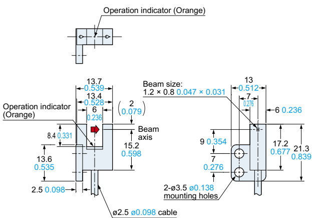
PM-F45□ Sensor
