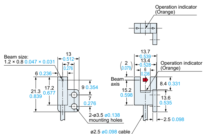
PM-R45□ Sensor
