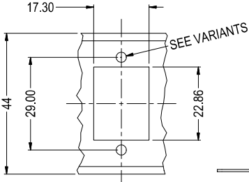
HOLE DETAIL
