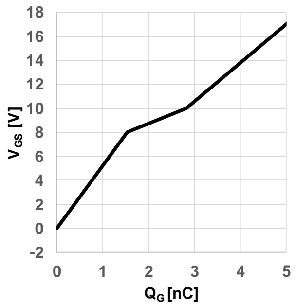
Figure 10 Typical gate charge ( V_{GS} = f(Q_G), I_{DS} = 2A, V_{DS} = 800V , turn-on pulse)
