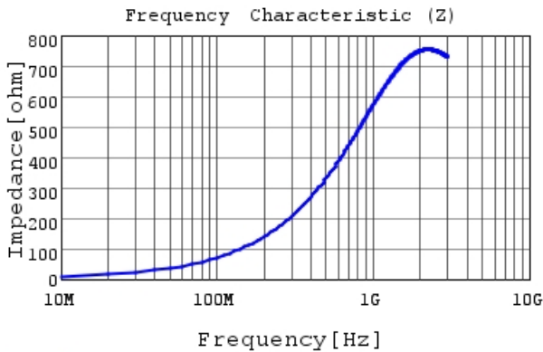
LQW18CNR12J0H |Z|
