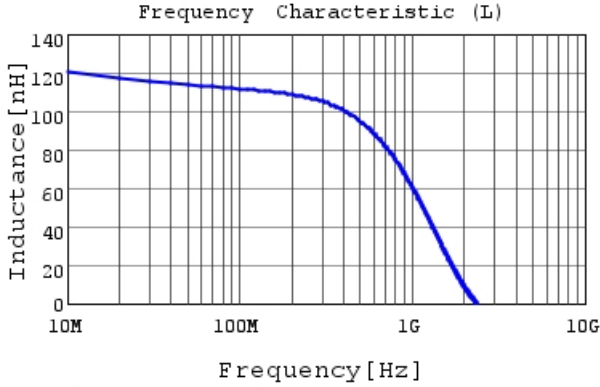
LQW18CNR12J0H L
