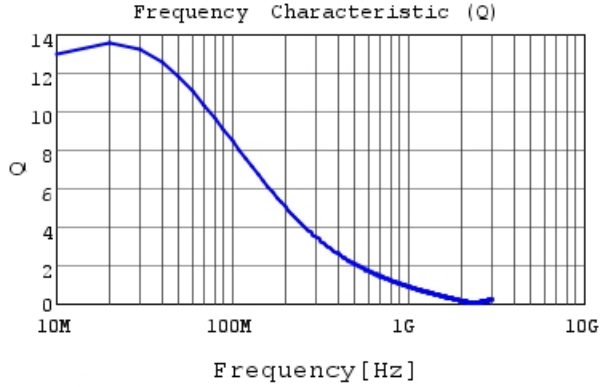
LQW18CNR12J0H Q
