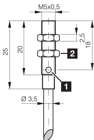
1) LED 2) Width over flats 7 mm BK: black BN: brown BU: blue
