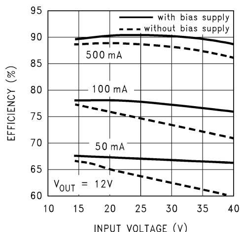
Figure 44. Effects of Bias Supply Feature on 12V Regulator Efficiency
