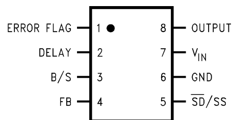
Figure 3. 8-Lead Surface Mount (D) Top View See Package Number D0008A
