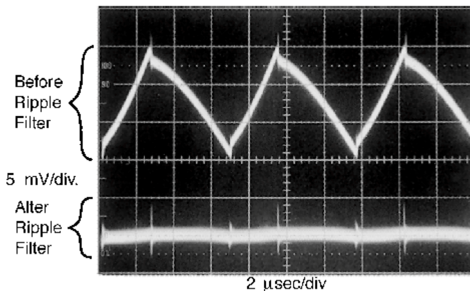
Figure 39. Post Ripple Filter Waveform
