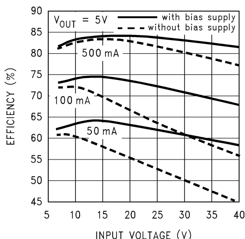
Figure 43. Effects of Bias Supply Feature on 5V Regulator Efficiency
