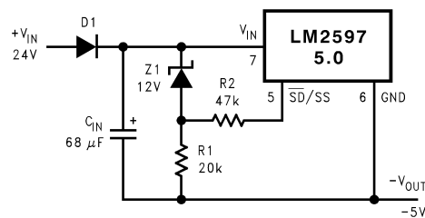
Figure 52. Undervoltage Lockout With Hysteresis for an Inverting Regulator
