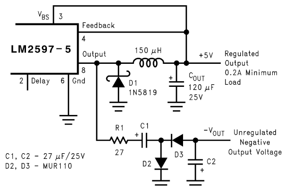
Figure 53. Charge Pump for Generating a Low Current, Negative Output Voltage
