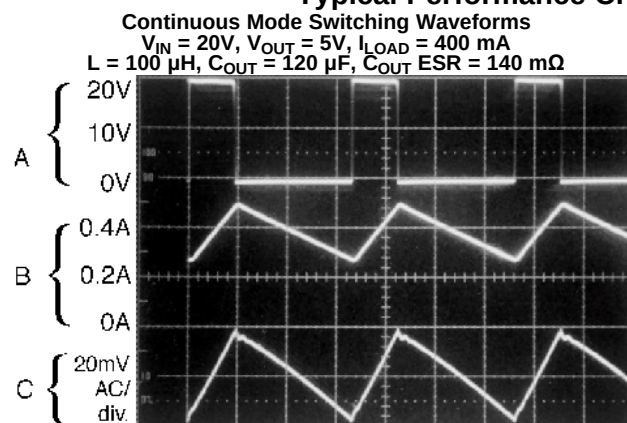
Figure 22. Horizontal Time Base: 2 \mu\text{s} /div.
