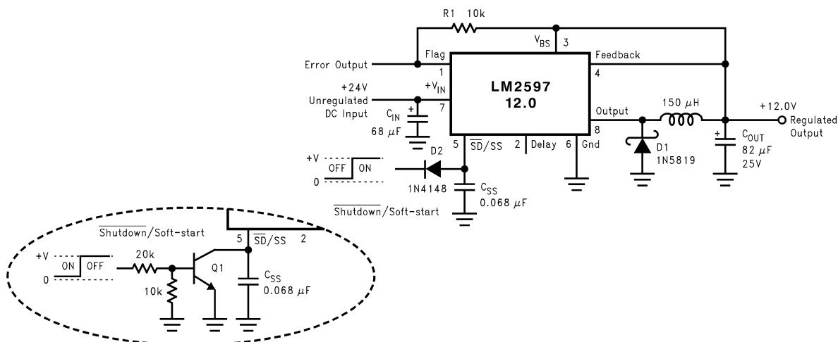
Figure 47. Typical Circuit Using Shutdown /Soft-start and Error Flag Features
