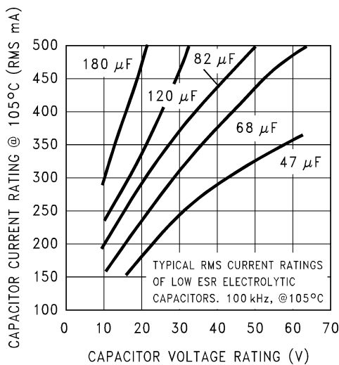
Figure 35. RMS Current Ratings for Low ESR Electrolytic Capacitors (Typical)
