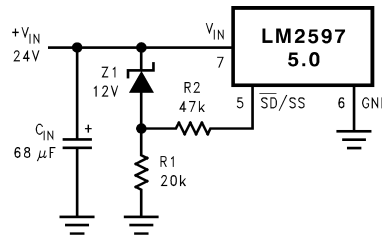
Figure 50. Undervoltage Lockout for a Buck Regulator
