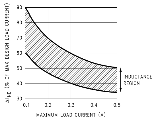
Figure 38. ( \Delta I_{IND} ) Peak-to-Peak Inductor Ripple Current (as a Percentage of the Load Current) vs Load Current
