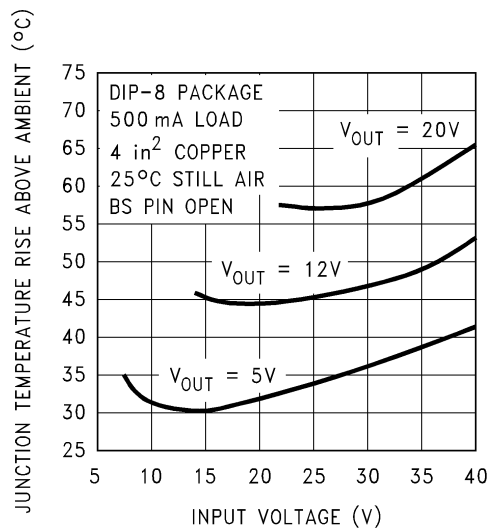
Figure 41. Junction Temperature Rise, PDIP-8
