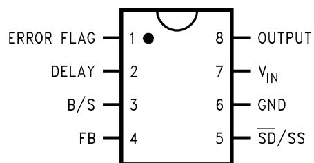
Figure 2. 8-Lead PDIP (P) Top View See Package Number P0008E
