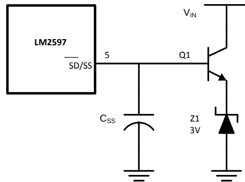
Figure 34. External 3.7V Soft-Start Clamp
