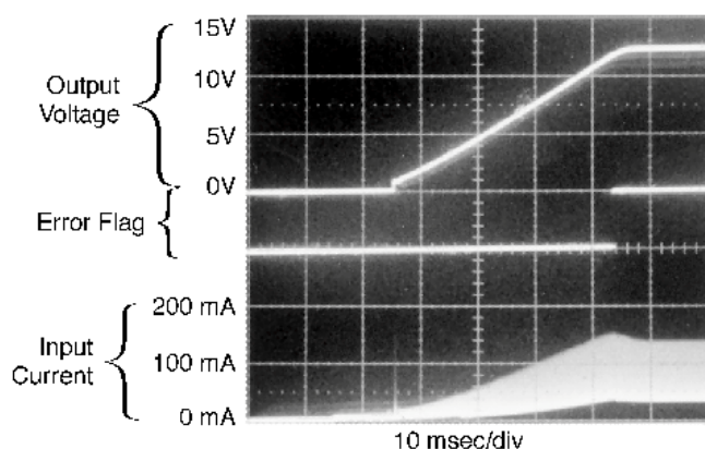
Figure 45. Output Voltage, Input Current, Error Flag Signal, at Start-Up, WITH Soft-start
