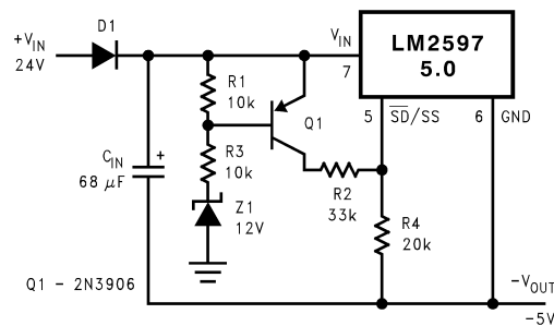
Figure 51. Undervoltage Lockout Without Hysteresis for an Inverting Regulator
