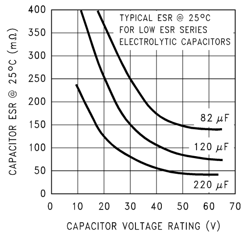
Figure 36. Capacitor ESR vs Capacitor Voltage Rating (Typical Low ESR Electrolytic Capacitor)
