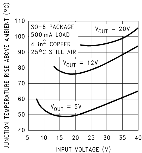
Figure 42. Junction Temperature Rise, SOIC-8
