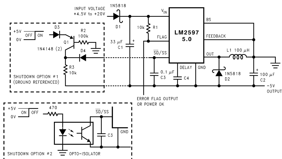
Figure 48. Inverting -5V Regulator With Shutdown and Soft-start
