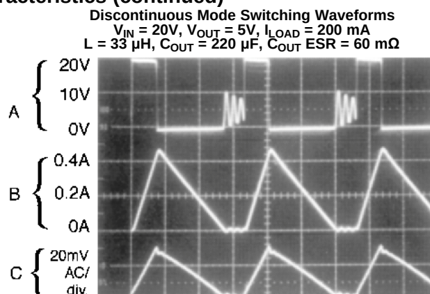
Figure 23. Horizontal Time Base: 2 \mu\text{s} /div.
