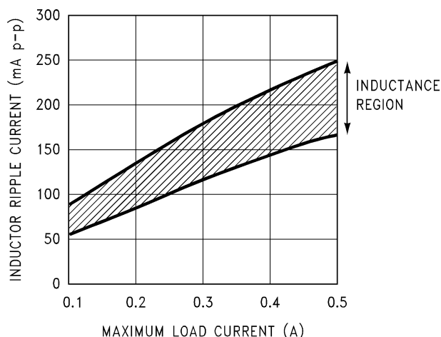
Figure 40. Peak-to-Peak Inductor Ripple Current vs Load Current
