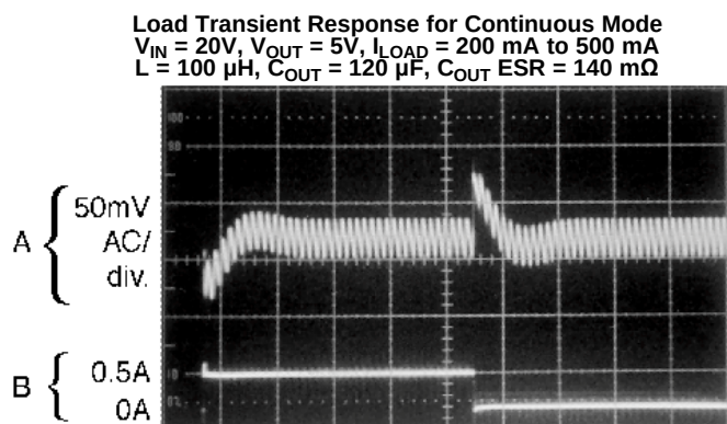
Figure 22. Horizontal Time Base: 2 \mu\text{s} /div.
