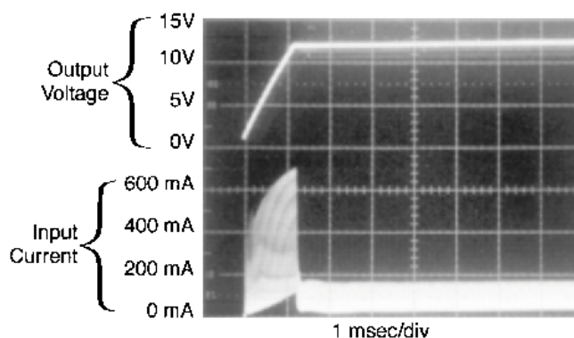
Figure 46. Output Voltage, Input Current, at Start-Up, WITHOUT Soft-start
