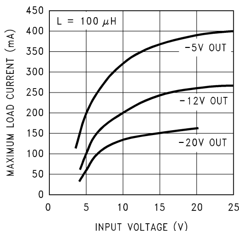
Figure 49. Maximum Load Current for Inverting Regulator Circuit
