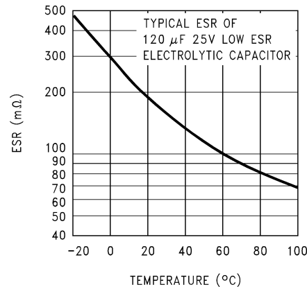
Figure 37. Capacitor ESR Change vs Temperature
