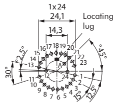
Drilling diagram 15° for indexing angle
