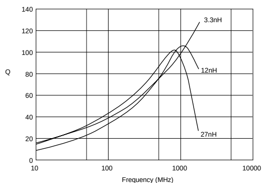
LQW2BH_03
