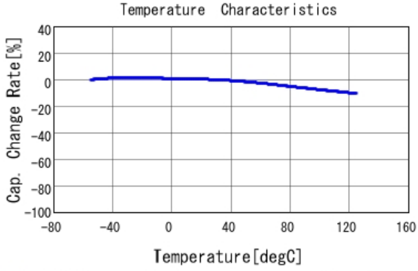
■ KRM55WR72A226MH01 C-Temp. capchange, DCOV, ACO. 5Vrms
