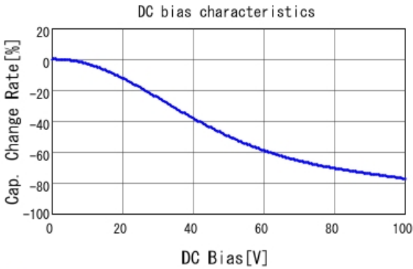
■ KRM55WR72A226MH01 C-DC bias capchange, 25.0degC, AC0.
