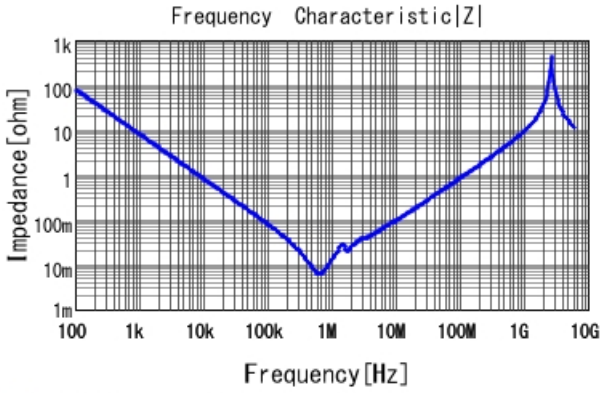
■ KRM55WR72A226MH01 |Z| DCOV, 25degC
