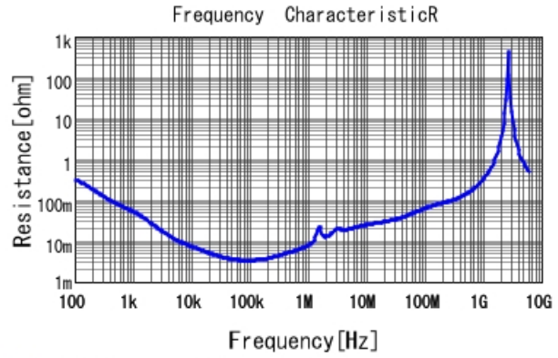
■ KRM55WR72A226MH01 R DCOV, 25degC
