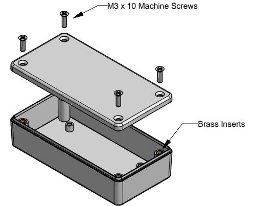
EXPLODED VIEW OF ENCLOSURE
