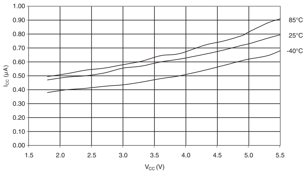
Figure 29-53. Oscillator Current vs. V_{CC} (32 kHz Watch Crystal)
