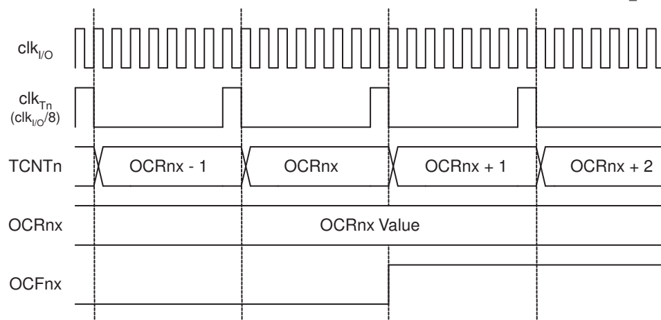
Figure 15-11. Timer/Counter Timing Diagram, Setting of OCF1x, with Prescaler ( f_{\text{clk}_{I/O}}/8 )
