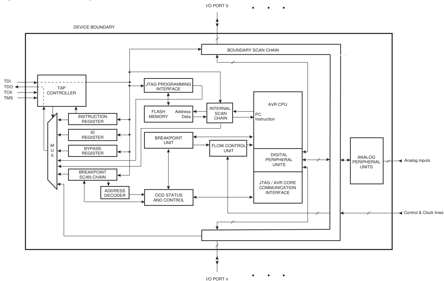
Figure 24-1. Block Diagram
