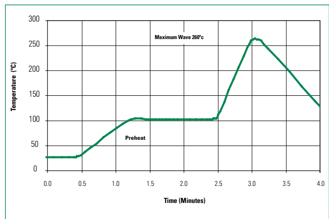
Soldering Profile
