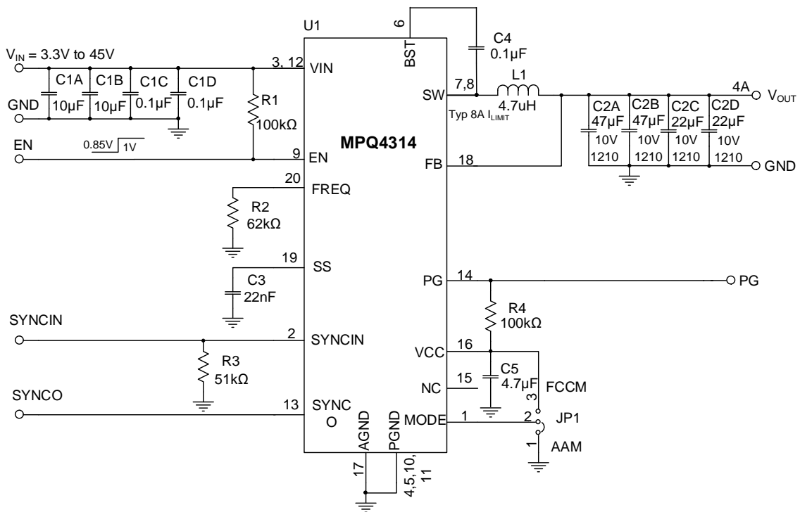
Figure 15: Typical Application Circuit ( f_{sw} = 470\text{kHz} , 3.3V Fixed Output)
