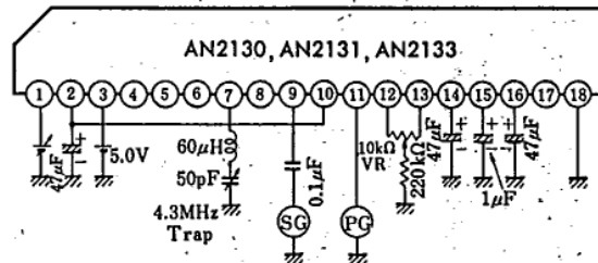
Test Circuit 5 ( A_{11(Fade)} )
