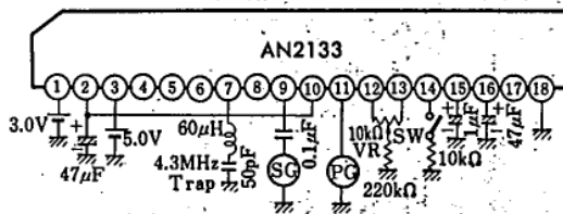
Test Circuit 9 ( v_{max.1} , v_{max.2} )
