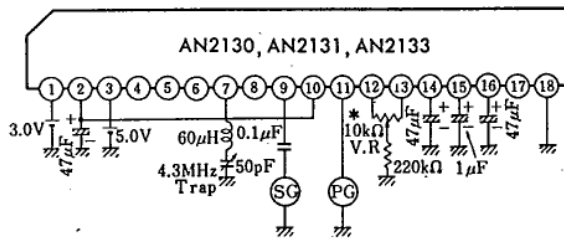
Test Circuit 4 ( v_{O(AGC)} , \Delta v_{O(AGC-1)} , \Delta v_{O(AGC-2)} )
