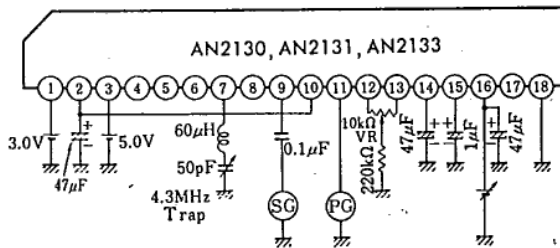
Test Circuit 6 ( v_{O(r1)} , v_{O(r2)} )
