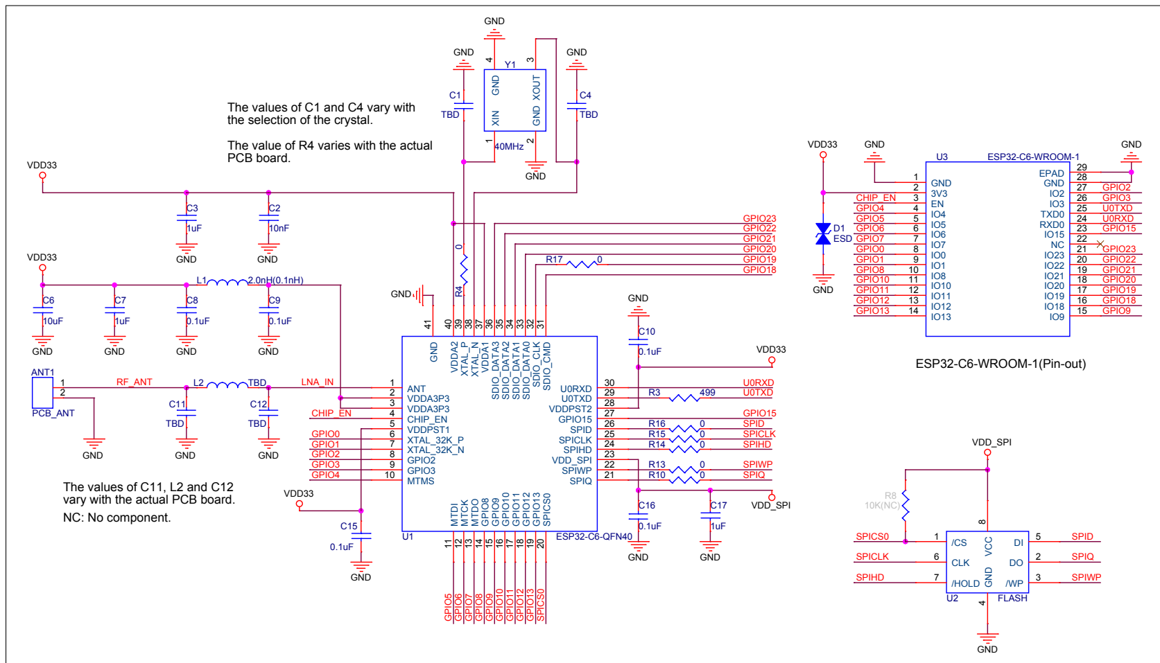
Figure 5: ESP32-C6-WROOM-1 Schematics
