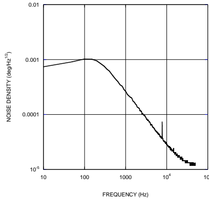
Noise Spectrum at 50mT FW = 10
