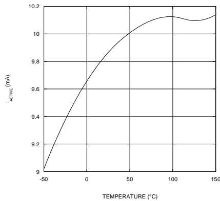
Supply Current Active mode, VDD = 3.3V
