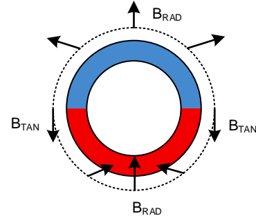
Figure 23: Side-Shaft Field
