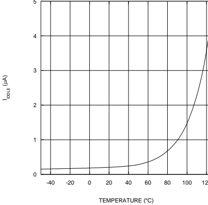
Supply Current Idle mode, VDD = 3.3V
