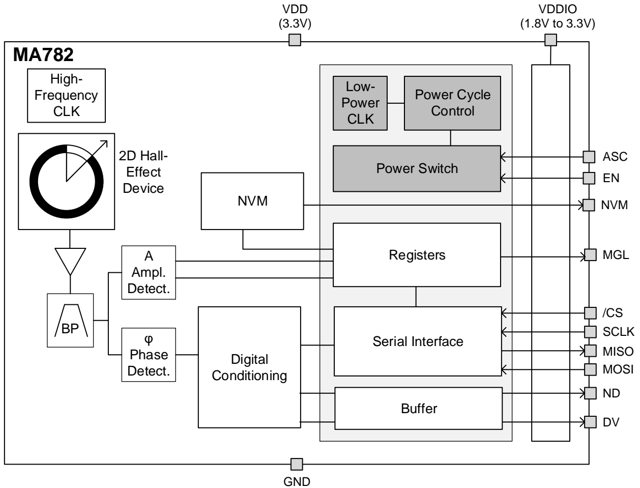
Figure 1: Functional Block Diagram (Gray Area Operates in Idle Mode)
