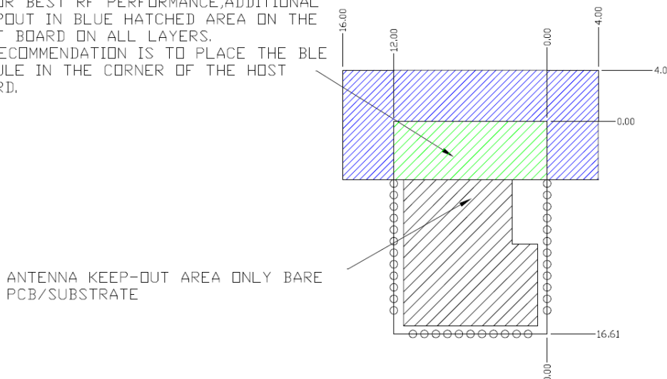
Figure 4. Optional Additional Host PCB Keep Out Area Around the CYBT-243053-02 PCB Antenna
