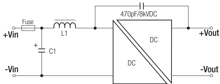
EMC Filtering - Suggestions for Class B
