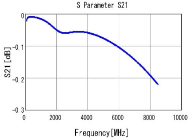
■ GRM0335C1E271JA01 S21 DCOV, 25degC
