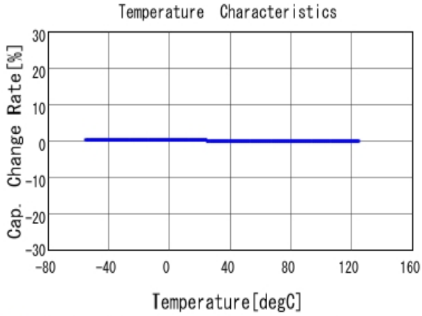
■ GRM0335C1E271JA01 C-Temp. capchange, DCOV, AC1Vrms
