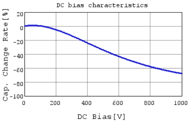
DE2E3SA102MN2AT01F C-DC bias capchange, 20.0
