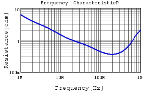
DE2E3SA102MN2AT01F R DCOV, 20degC
