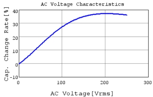
DE2E3SA102MN2AT01F C-AC Voltage capchange, I
