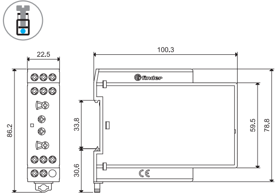
83.02/52 Screw terminal
