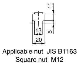
Dimensions of T-slot for mounting
