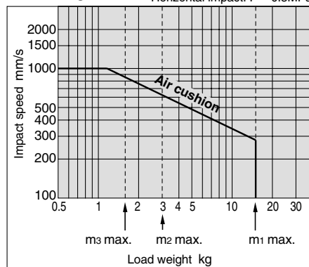
MY1B16 Horizontal impact: P = 0.5\text{MPa}
