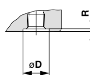
Bottom side (ZZ) piping (applicable O-ring)
