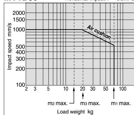
MY1B50 Horizontal impact: P = 0.5\text{MPa}
