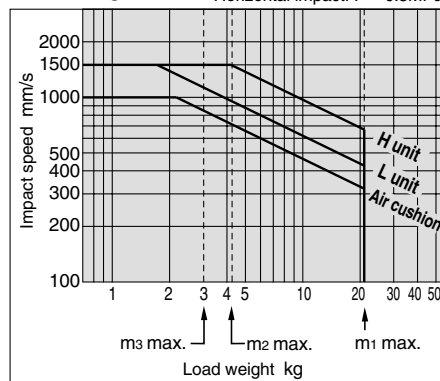
MY1B20 Horizontal impact: P = 0.5\text{MPa}
