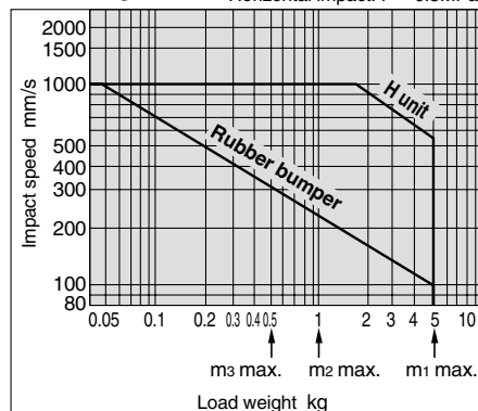
MY1B10 Horizontal impact: P = 0.5\text{MPa}
