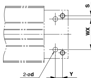
Bottom side (ZZ) piping (applicable O-ring)
