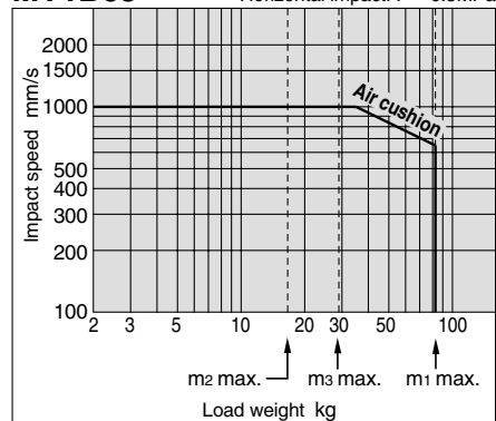
MY1B63 Horizontal impact: P = 0.5\text{MPa}
