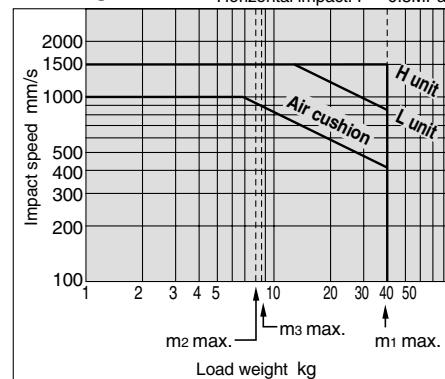
MY1B32 Horizontal impact: P = 0.5\text{MPa}
