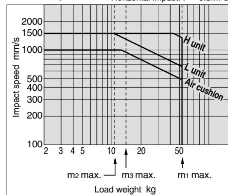
MY1B40 Horizontal impact: P = 0.5\text{MPa}
