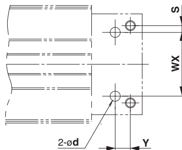
Bottom side (ZZ) piping (applicable O-ring)
