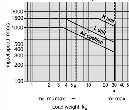
MY1B25 Horizontal impact: P = 0.5\text{MPa}
