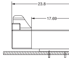
Horizontal Type
