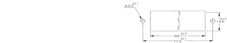
Panel Cutout
