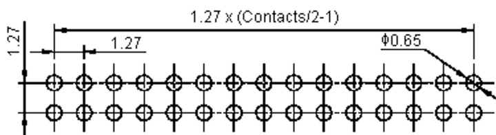
PCB Layout
