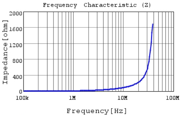
DFE322520FD-1R5M |Z|
