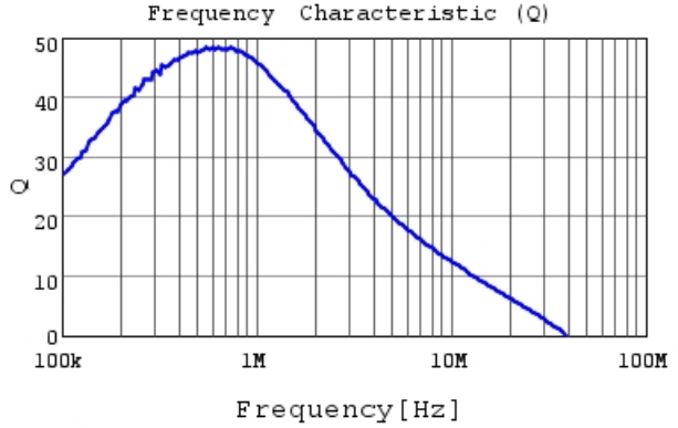
DFE322520FD-1R5M Q
