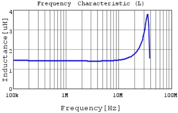
DFE322520FD-1R5M L
