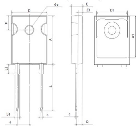
TO-247-2L, (TO-247GE-2L)
