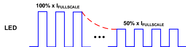
Figure 9: PWM Dimming via I 2 C Interface
