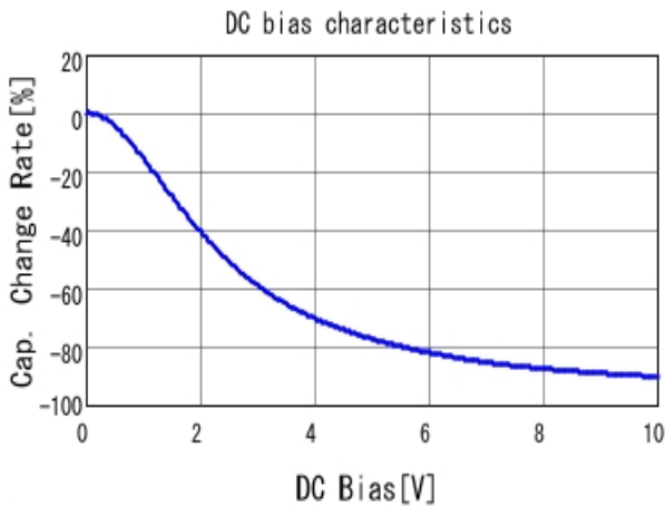
■ GRM033R61A225KE47 C-DC bias capchange, 25.0degC, AC1V
