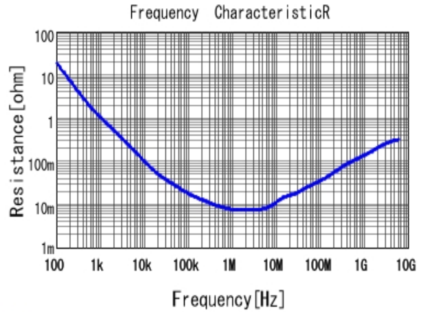
■ GRM033R61A225KE47 R DCOV, 25degC
