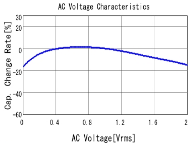
■ GRM033R61A225KE47 C-AC Voltage capchange, DCOV, 25.0d
