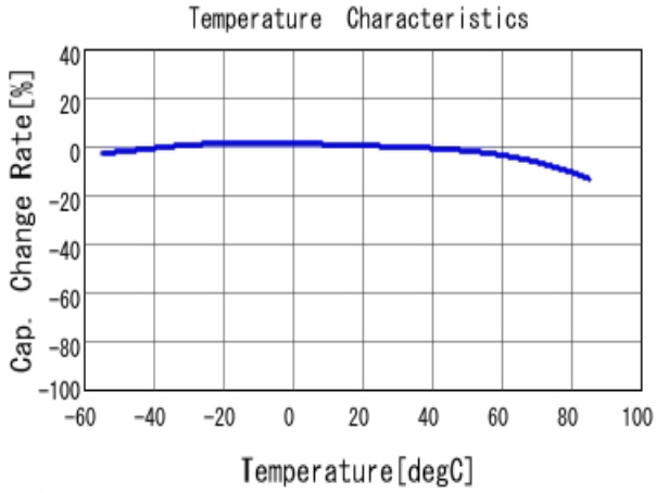
■ GRM033R61A225KE47 C-Temp. capchange, DCO. 0V, ACO. 2V rm
