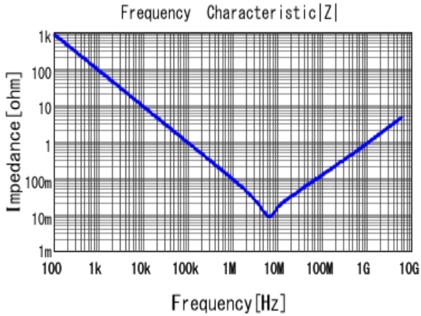
■ GRM033R61A225KE47 |Z| DCOV, 25degC
