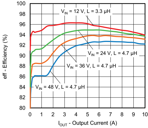
Fig. 10 - SiC476 Efficiency vs. Output Current, V_{OUT} = 5\text{ V}
