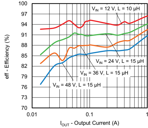
Fig. 31 - SiC479 Efficiency vs. Output Current - Light Load, V_{OUT} = 5\text{ V}
