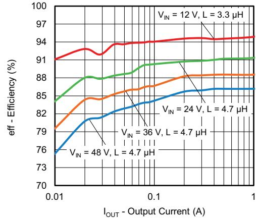
Fig. 13 - SiC476 Efficiency vs. Output Current - Light Load, V_{OUT} = 5\text{ V}
