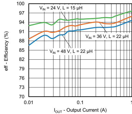
Fig. 26 - SiC478 Efficiency vs. Output Current - Light Load, V_{OUT} = 12\text{ V}
