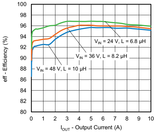
Fig. 11 - SiC476 Efficiency vs. Output Current, V_{OUT} = 12\text{ V}
