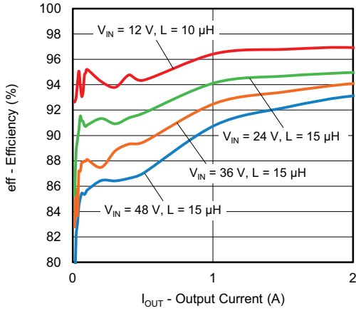
Fig. 28 - SiC479 Efficiency vs. Output Current, V_{OUT} = 5\text{ V}
