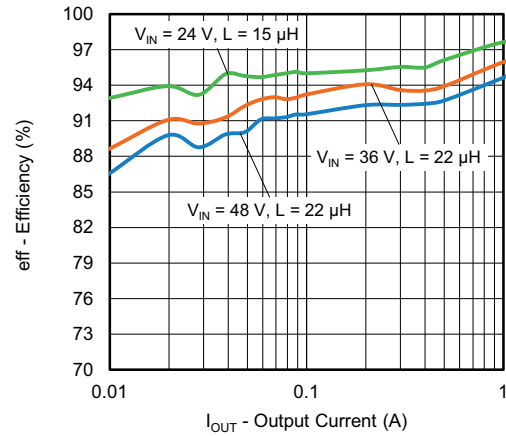
Fig. 32 - SiC479 Efficiency vs. Output Current - Light Load, V_{OUT} = 12\text{ V}
