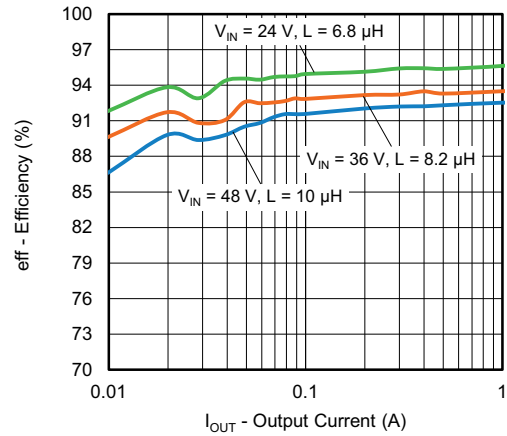
Fig. 14 - SiC476 Efficiency vs. Output Current - Light Load, V_{OUT} = 12\text{ V}
