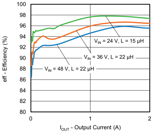
Fig. 29 - SiC479 Efficiency vs. Output Current, V_{OUT} = 12\text{ V}
