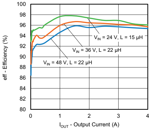
Fig. 23 - SiC478 Efficiency vs. Output Current, V_{OUT} = 12\text{ V}
