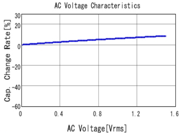
■ KCM55WR71E686MH01 C-AC Voltage capchange, DCOV, 25.0d
